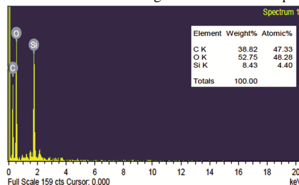
Fig. 5 — Energy dispersive spectra of luffa composite
