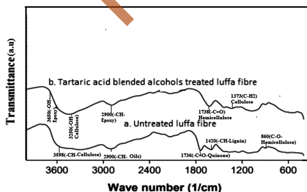
Fig. 6 — FTIR spectra of (a) untreated luffa fibre (b) treated luffa fibre
