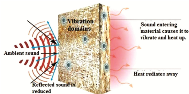
Fig. 3 — Mechanism of sound absorption within the composites
