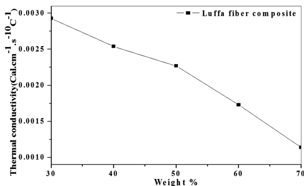
Fig. 8 — Thermal conductivity of luffa fibre biocomposite
