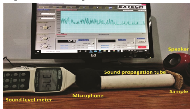
Fig. 2 — Experimental setup for measurement of sound absorption
