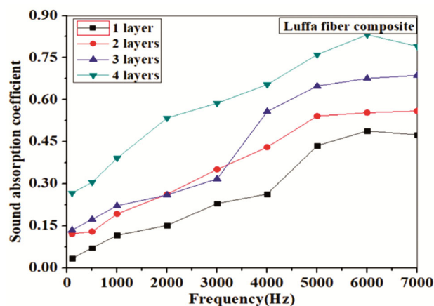
Fig. 7 — Sound absorption coefficient of luffa fiber composite
