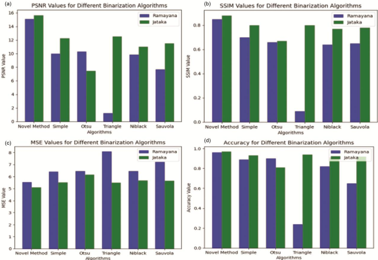
Supplementary Fig. S2 — Comparison of the results of various binarisation techniques with the novel method: (a) PSNR, (b) SSIM, (c) MSE, (d) Accuracy
