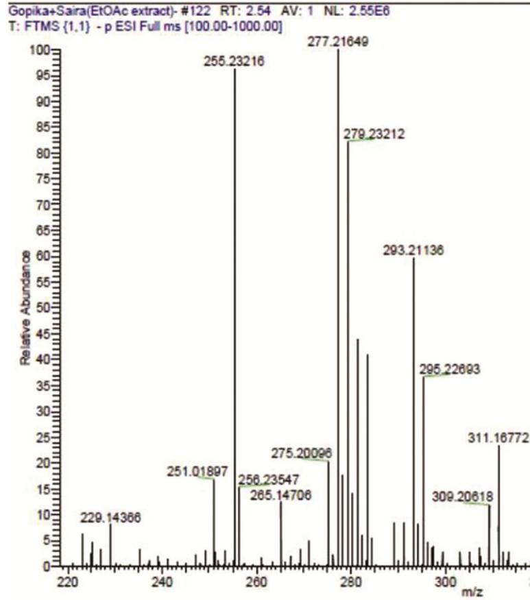
Supplementary Fig. S2 — HRMS spectrum of ethyl acetate extract of leaves of J. simplex
