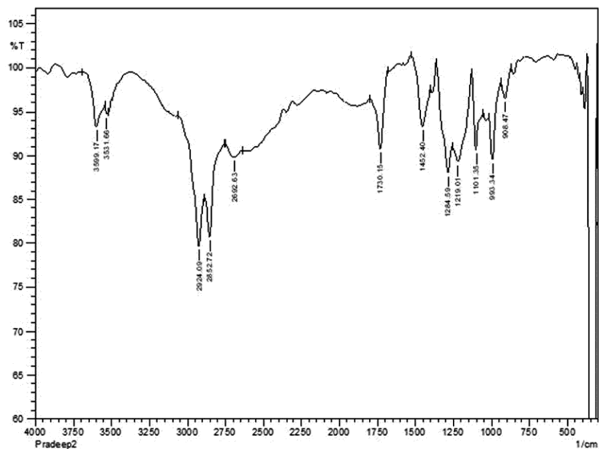
Supplementary Fig. S1 — FTIR spectrum of ethyl acetate extract of leaves of J. simplex
