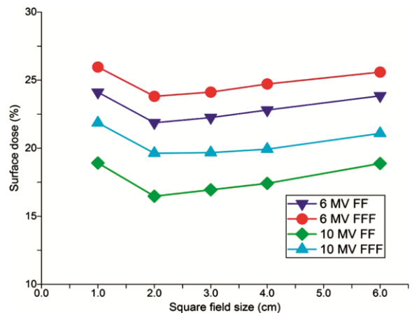
Fig. 8 — Percentage surface dose versus field size for 10 and 6 MV unflat (FFF) and flat (FF) beams.
