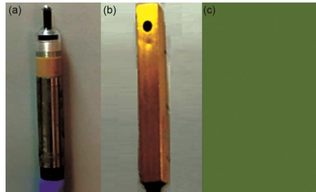
Fig. 1 — Photographs of (a) PinPoint (b) EDGE (c) EBT3 detectors.
