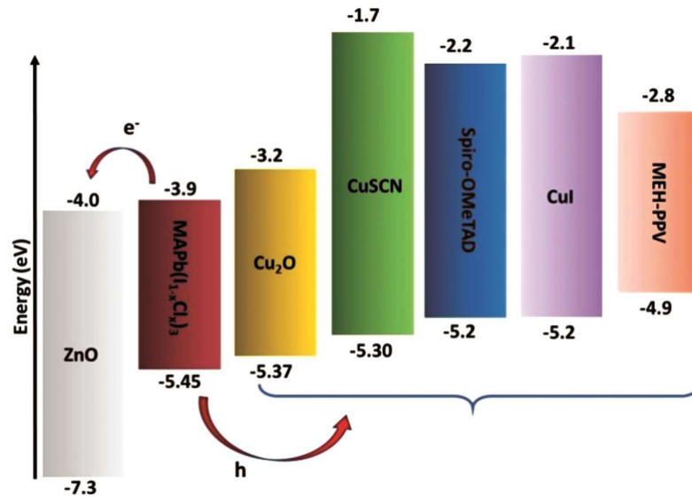
Fig. 2 — Band alignments of ZnO, perovskite absorber and various proposed HTL materials.
