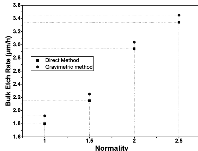
Fig. 2 — Graph between normality and bulk etch rate calculated using direct and gravimetric methods.
