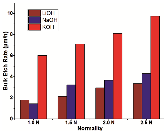
Fig. 4 — Graph showing the bulk etch rate of KOH, NaOH and LiOH at different concentrations.
