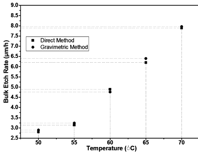
Fig. 3 — Graph between temperature and bulk etch rate calculated using direct and gravimetric methods.
