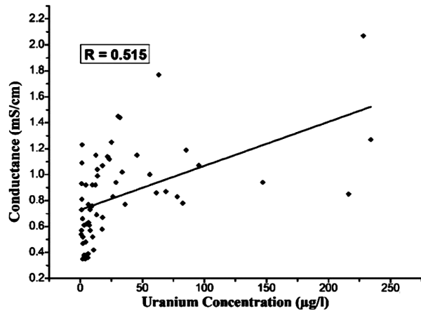
Fig. 4 — Uranium concentration vs conductance in water samples.
