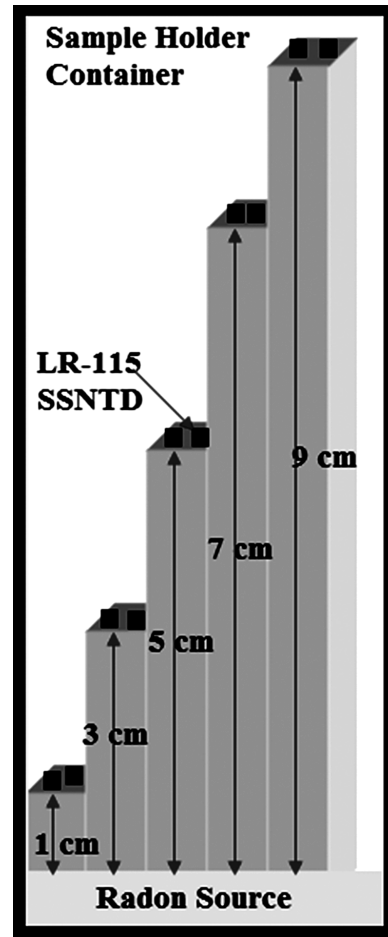
Fig. 1 — Experimental set-up for detectors deployment.
