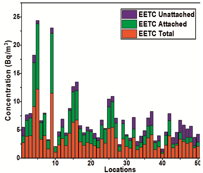
Fig. 5 — Bar graph showing the concentration of attached and unattached progenies of indoor thoron.
