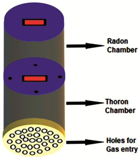
Fig. 2 — Block diagram of pin-hole dosimeter.
