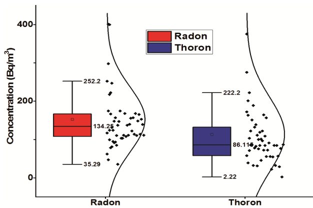
Fig. 3 — Box-whisker plot of radon and thoron concentration.
