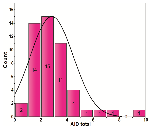
Fig. 6 — Frequency distribution plot for total annual absorbed dose due to inhalation of radon and thoron gas.
