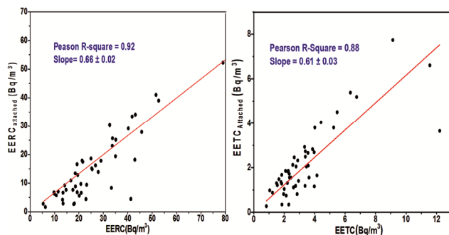
Fig.7 — Correlation plots between total and attached progeny concentrations of radon and thoron gases.
