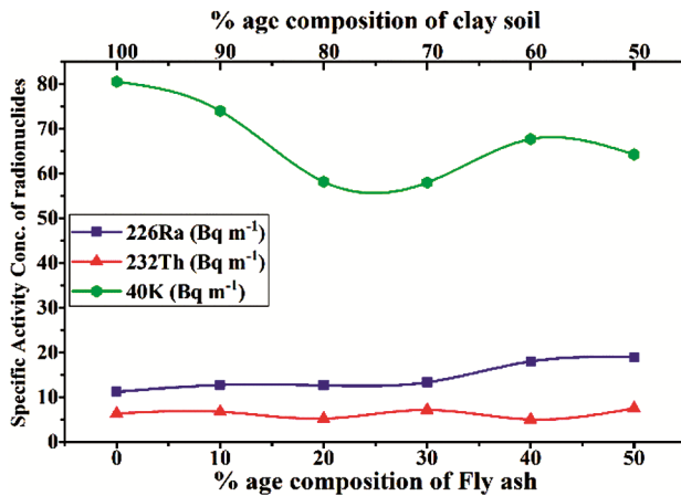
Fig. 4 — Graph showing activity concentration of radionuclides for different percentage compositions (fly ash in clay soil).
