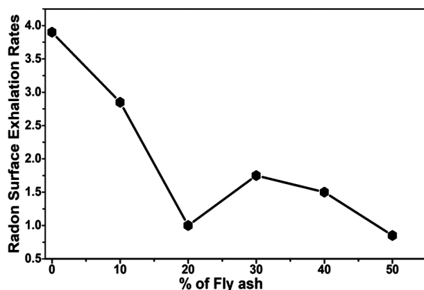
Fig. 5— Variation of radon surface exhalation rate with different amount composition of fly ash in clay soil.
