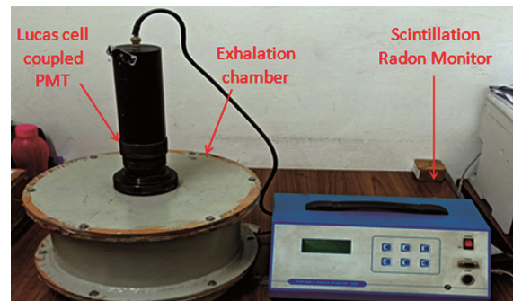
Fig. 3— Scintillation Radon Monitor with Exhalation chamber.
