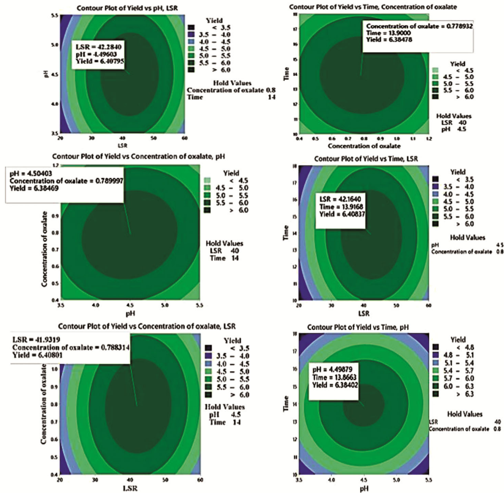
Fig. 1 — Contour plots of the yield of pectic substances from the leaves of H. pubescens as a function of liquid-to-solid ratio (LSR), pH, concentration of ammonium oxalate, and duration of heating.
