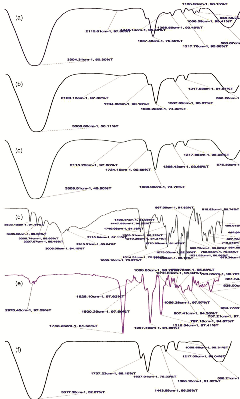
Fig. 3 — FTIR-ATR spectra (a) sucrose solution, (b) histidine solution (c) calcium chloride solution, (d) ascorbic acid powder, (e) pectic substances powder extracted from the leaves of H. pubescens , and (f) MCFM.
