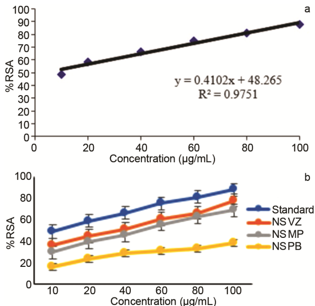
Fig. 4 — a) Standard calibration curve for Ascorbic acid; and b) DPPH activity of methanolic NSSE from different locations in comparison to AA. Results is expressed as mean±SD.
