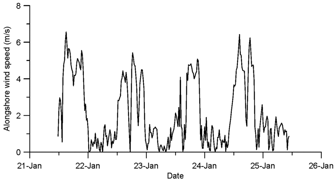
Fig. S2 — Longshore component of the wind observed off Calangute
