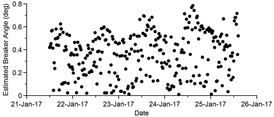
Fig. S1 — Breaker angle calculated based on Larson et al. (2010)
