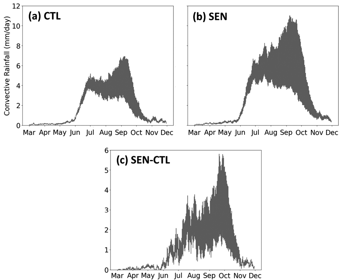
Figure S1 — Climatological annual cycle of convective rainfall activity (mm/day) in (a) CTL, and (b) SEN. Difference between climatological annual cycles of SEN and CTL model simulations in (c)
