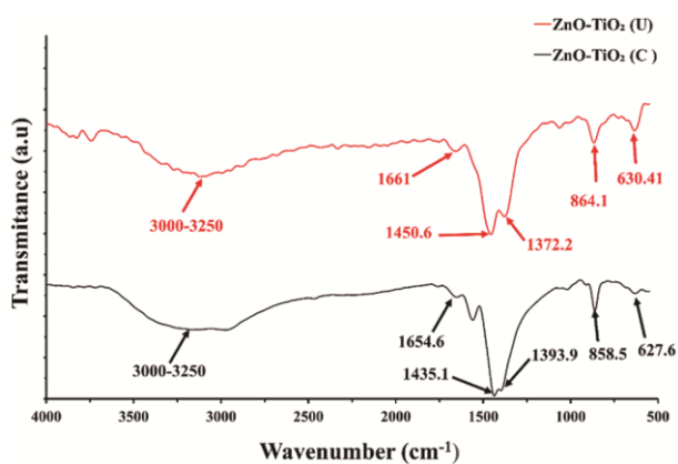
Fig. 2 — FTIR spectra of ultrasonically and conventionally synthesized ZTN
