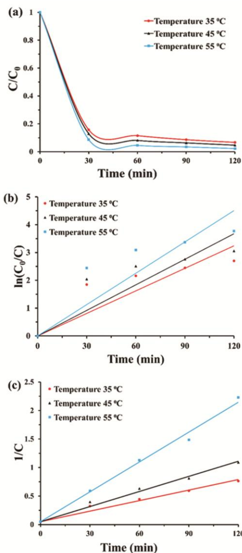
Fig. 9 — (a) Effect of temperature on dye degradation using ZTN synthesized by ultrasound method (catalyst loading = 1 g/L, initial dye concentration = 20 ppm, volume of batch = 100 mL, and pH = 7), (b) PFO kinetic model and (c) Second-order kinetic model
