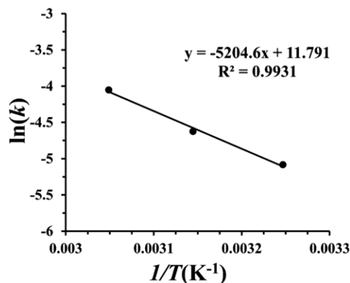
Fig. 10 — Plot of \ln(k) Vs. 1/T
