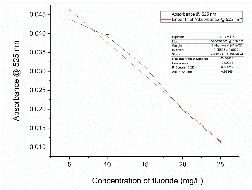
Fig. S1 — Standard graph for fluoride estimation
