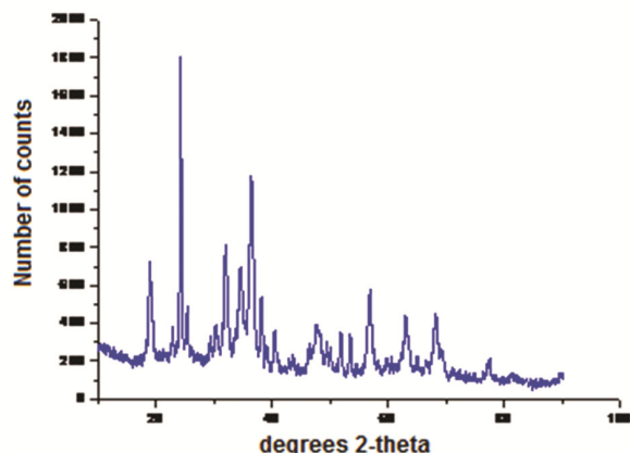
Fig. 1 — XRD pattern of ZnO/SnO 2 nanocomposite
