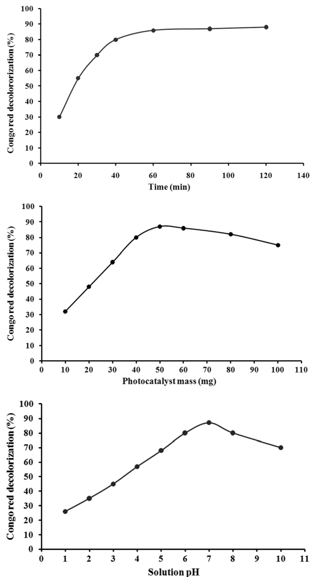
Fig. 8 — (a) Effect of the reaction time on the photo-decolorization of Congo red over \text{TiO}_2\text{S}(50) ; (b) Effect of the photocatalyst mass on the photo-decolorization of Congo red over \text{TiO}_2\text{-S}(50) ; (c) Effect of pH on the photo-decolorization of Congo red over \text{TiO}_2\text{-S}(50)
