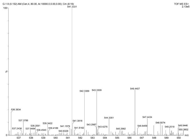
Fig.S6- Mass spectra of complex
