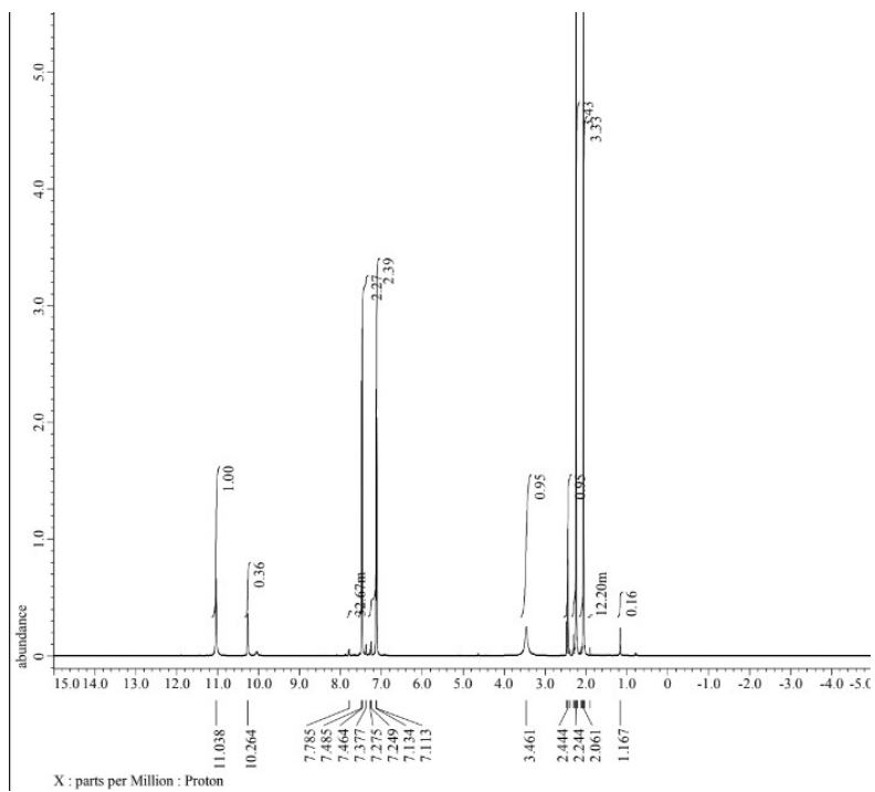
Fig.S4- ^1\text{H-NMR} spectra of Complex
