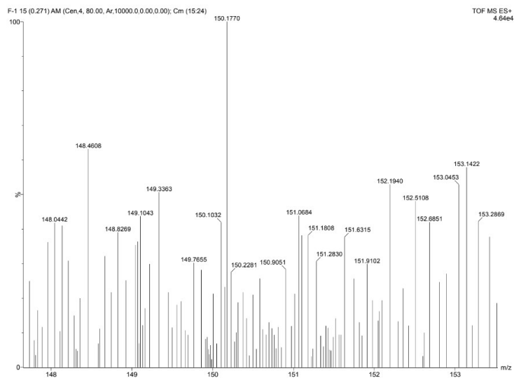
Fig.S5- Mass spectra of ligand
