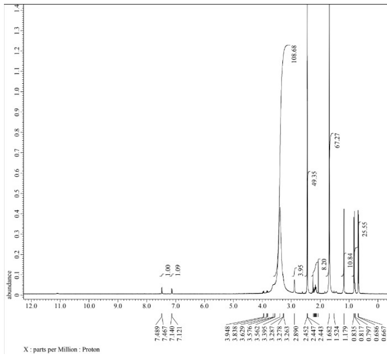
Fig.S3- ^1\text{H-NMR} spectra of ligand
