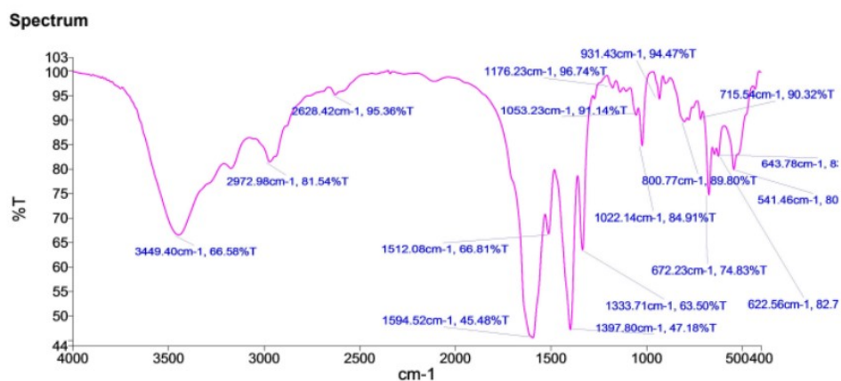
Fig.S1- FTIR spectra of ligand
