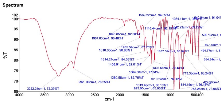
Fig.S2- FTIR spectra of complex
