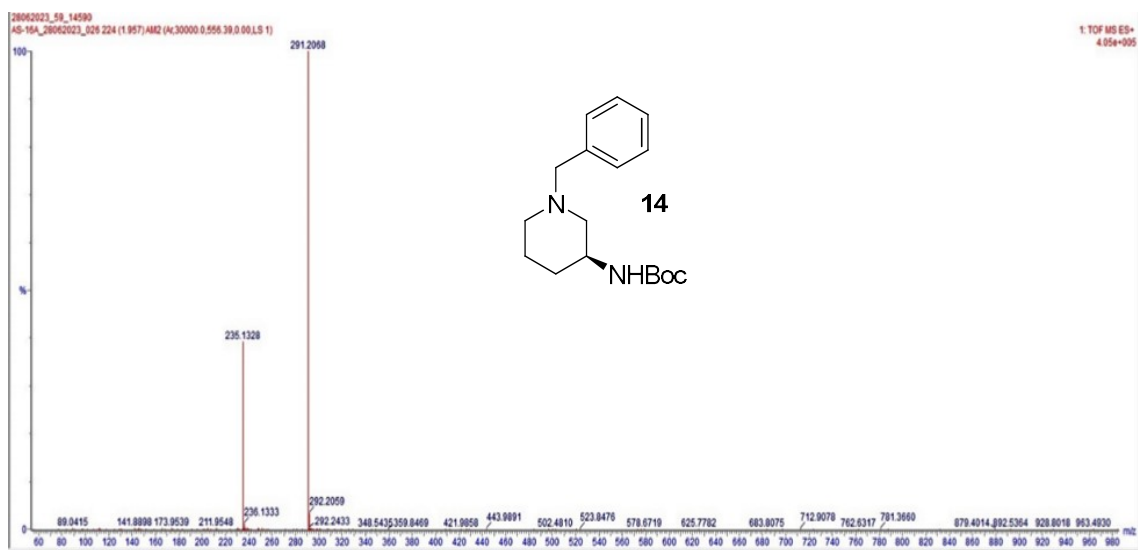
Fig. S26: HRMS Spectrum of compound 14
