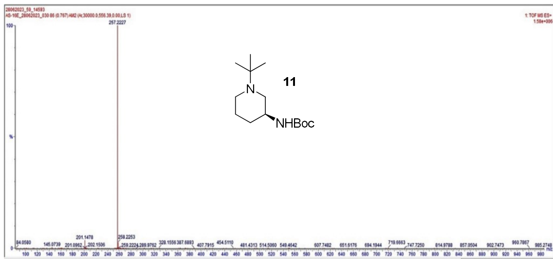
Fig. S23: HRMS Spectrum of compound 11
