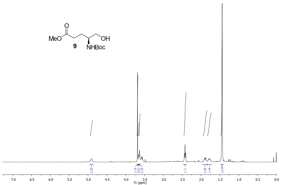
Fig. S6: ^1\text{H} NMR of Compound 9 (400 MHz, \text{CDCl}_3 )
