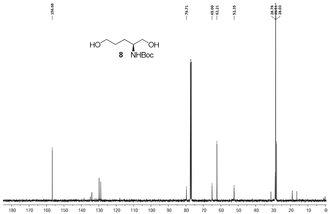
Fig. S5: ^{13}\text{C} NMR of Compound 8 (101 MHz, \text{CDCl}_3 )
