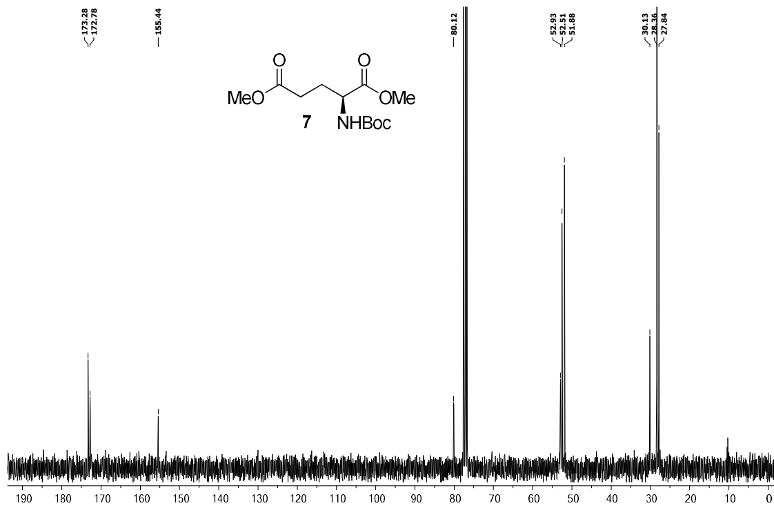
Fig. S3: ^{13}\text{C} NMR of Compound 7 (75 MHz, \text{CDCl}_3 )
