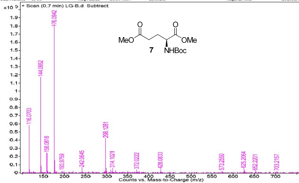
Fig. S19: HRMS Spectrum of compound 7
