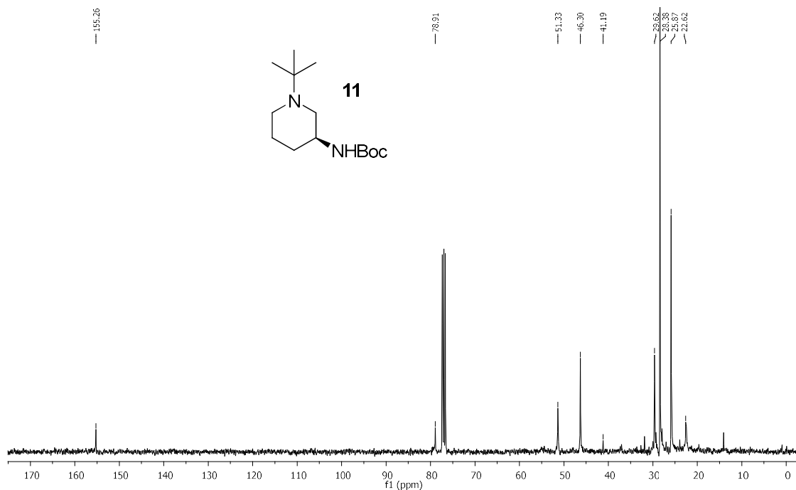
Fig. S11: ^{13}\text{C} NMR of Compound 11 (101 MHz, \text{CDCl}_3 )
