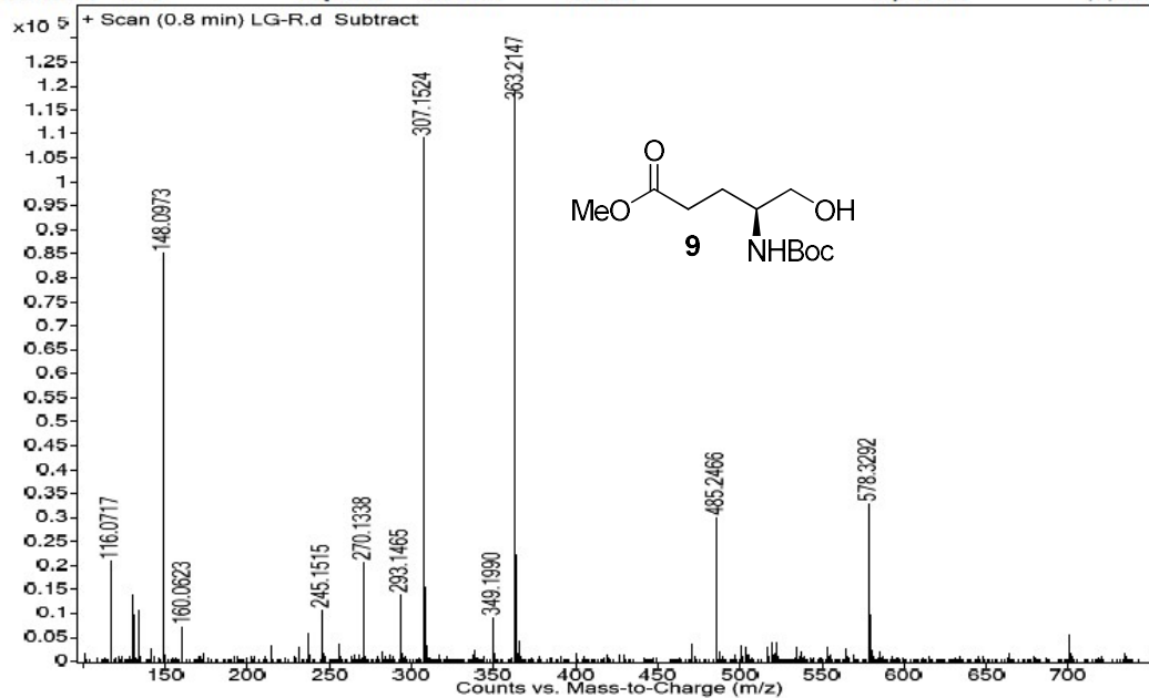
Fig. S21: HRMS Spectrum of compound 9
