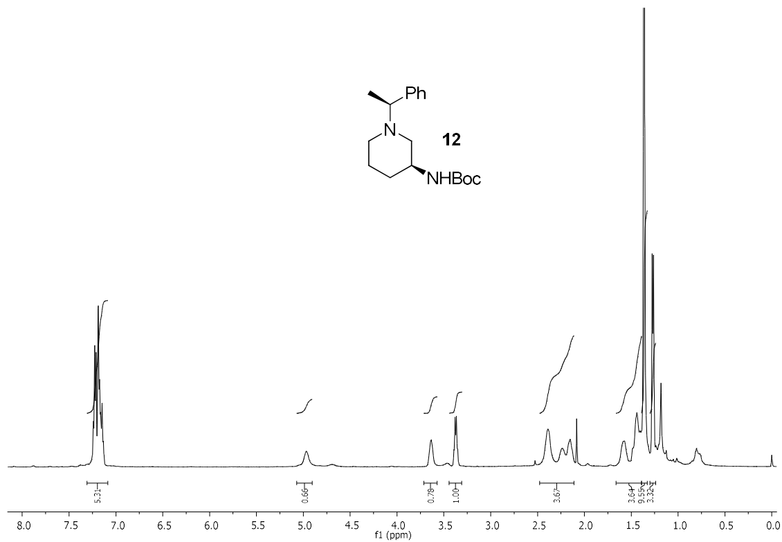
Fig. S12: ^1\text{H} NMR of Compound 12 (500 MHz, \text{CDCl}_3 )
