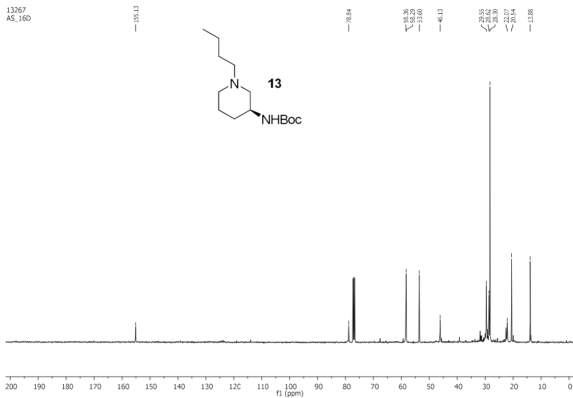
Fig. S15: 13 C NMR of Compound 13 (101 MHz, CDCl 3 )
