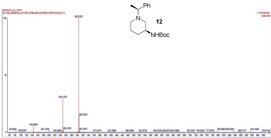
Fig. S24: HRMS Spectrum of compound 12
