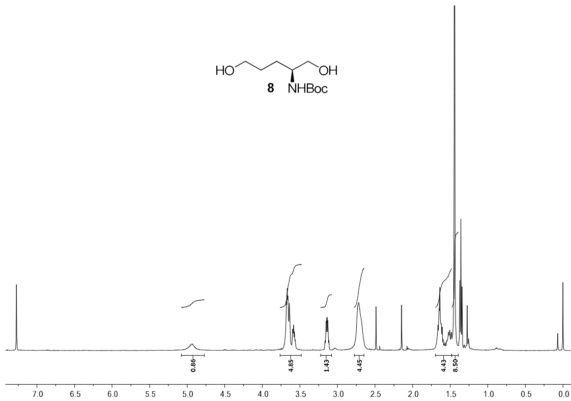
Fig. S4: ^1\text{H} NMR of Compound 8 (500 MHz, \text{CDCl}_3 )
