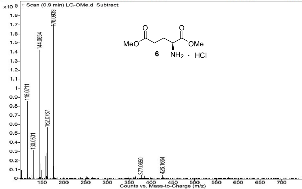
Fig. S18: HRMS Spectrum of compound 6
