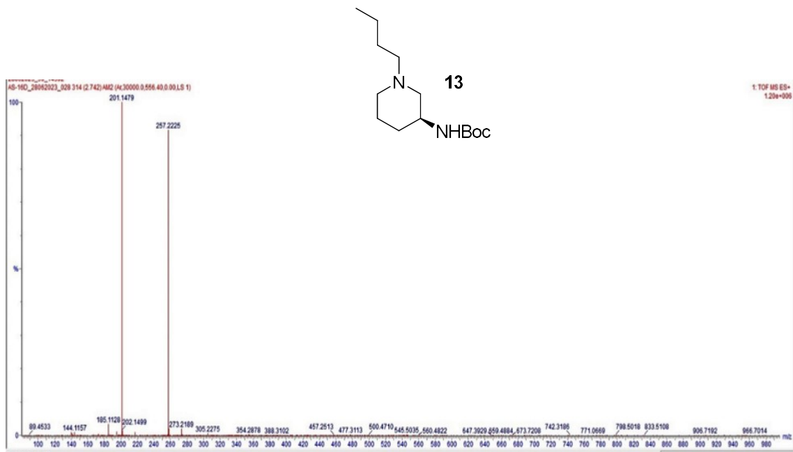
Fig. S25: HRMS Spectrum of compound 13
