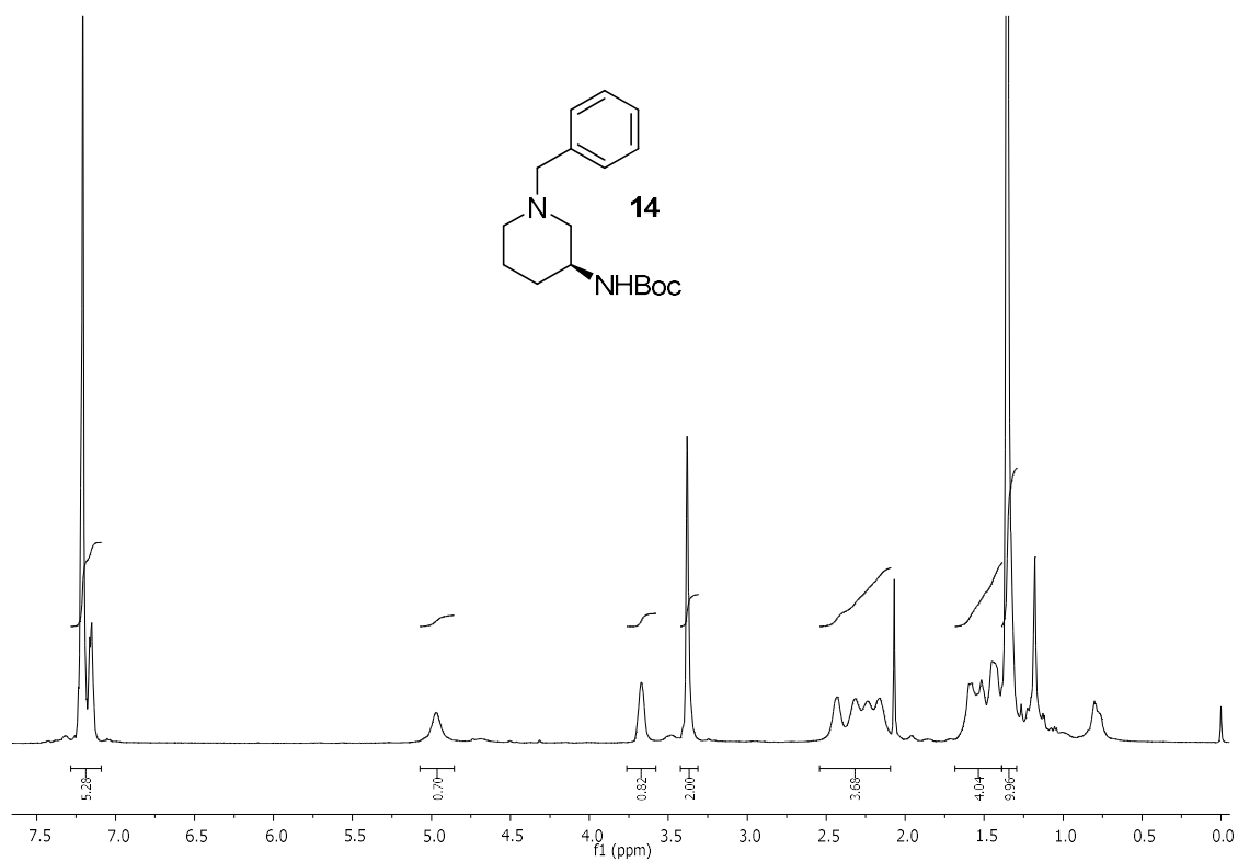
Fig. S16: 1 H NMR of Compound 14 (500 MHz, CDCl 3 )
