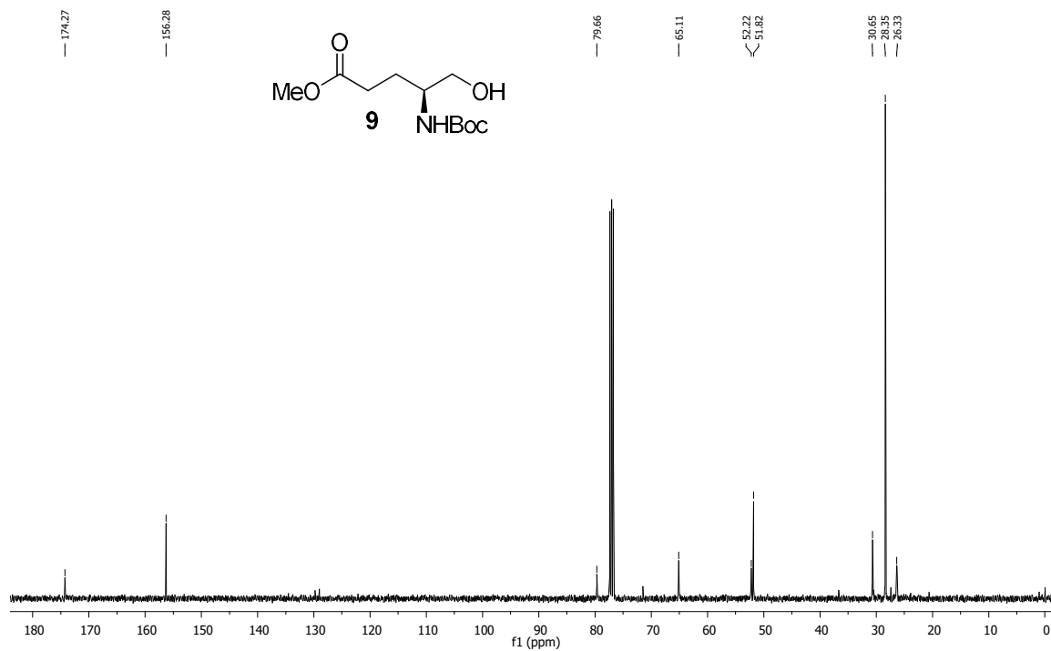
Fig. S7: ^{13}\text{C} NMR of Compound 9 (101 MHz, \text{CDCl}_3 )
