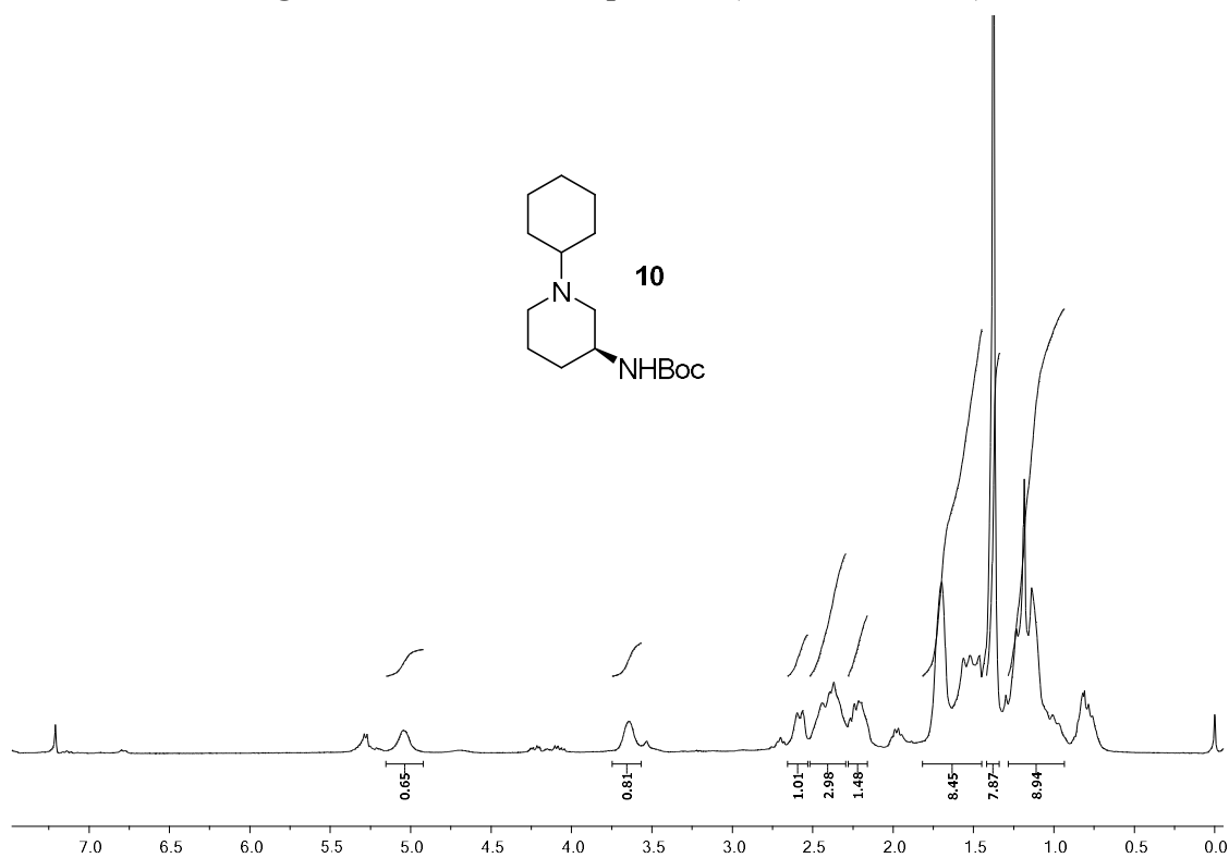
Fig. S8: ^1\text{H} NMR of Compound 10 (300 MHz, \text{CDCl}_3 )
