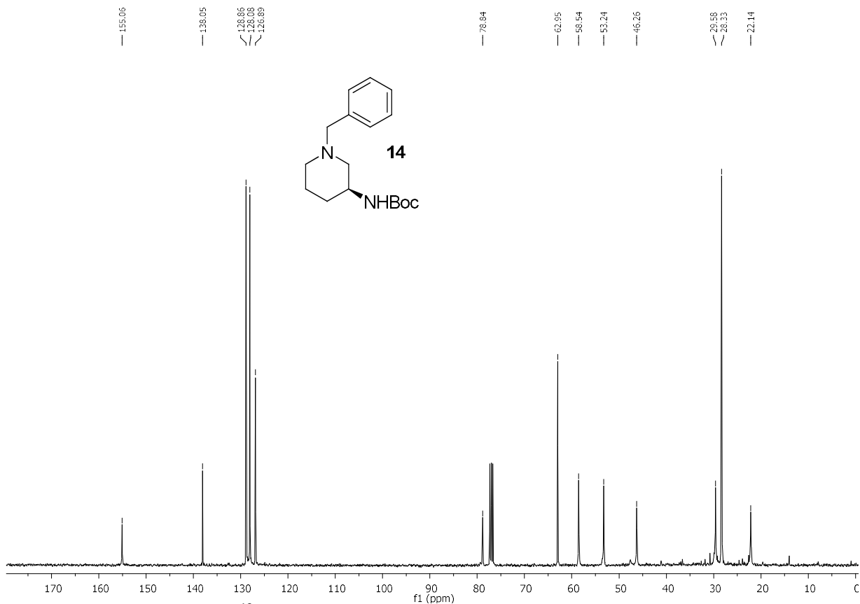
Fig. S17: ^{13}\text{C} NMR of Compound 14 (101 MHz, \text{CDCl}_3 )
