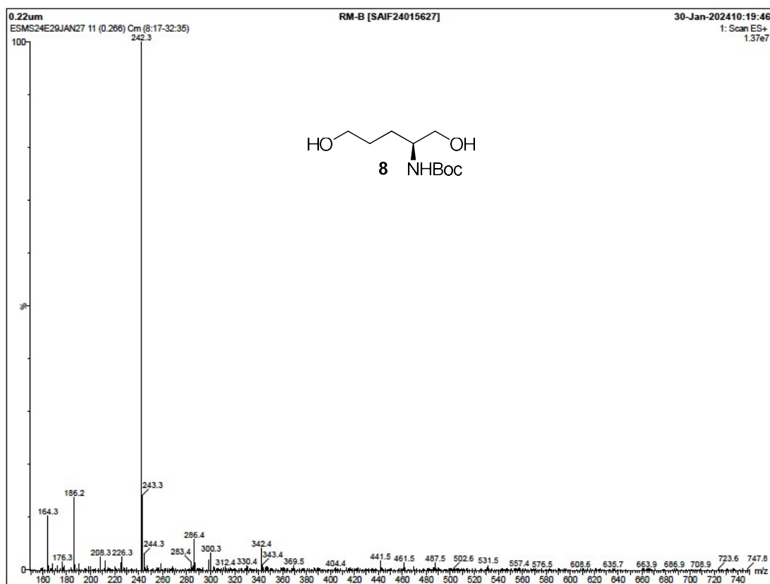
Fig. S20: ESI-MS Spectrum of compound 8
