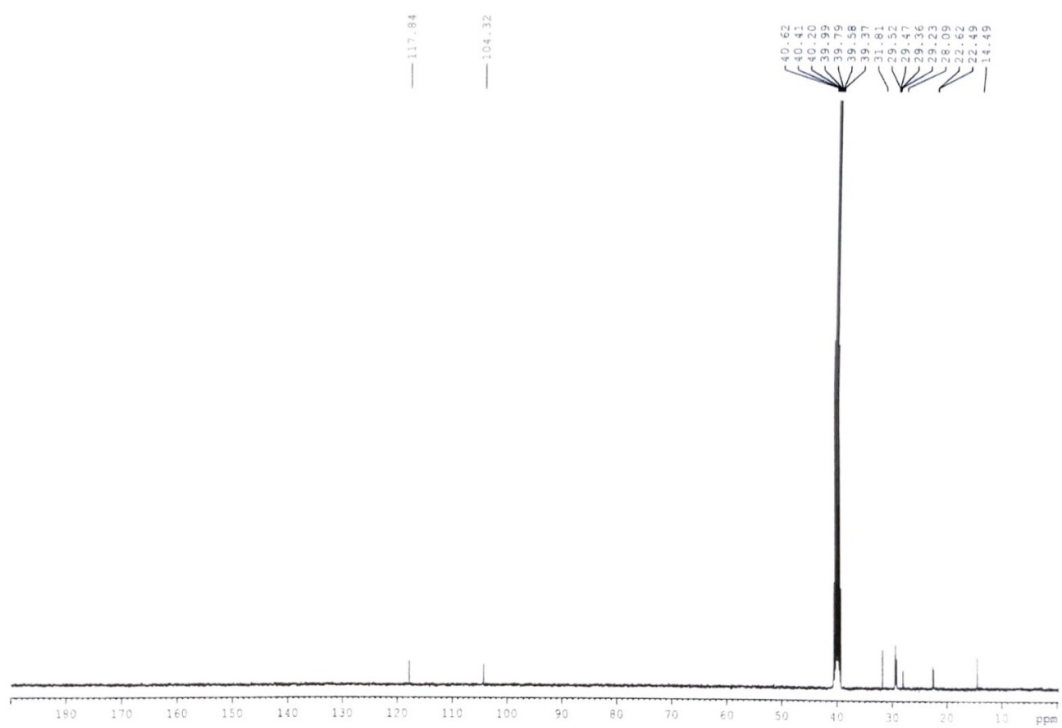
Figure S2: ^{13}\text{C} NMR spectra of Embelin
