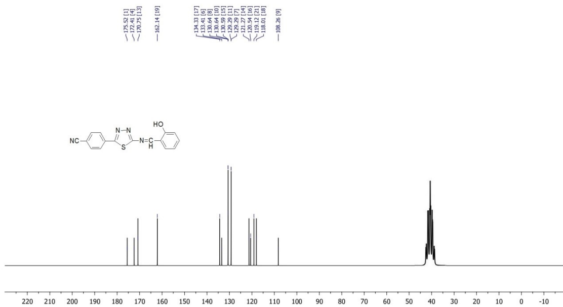
Figure 5 ^{13}\text{C} NMR spectra of Ligand.
