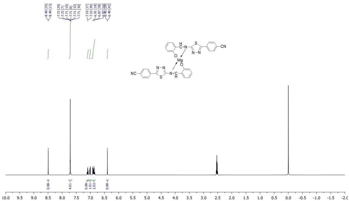
Figure 6 ^1\text{H} NMR spectra of Complex Mg.
