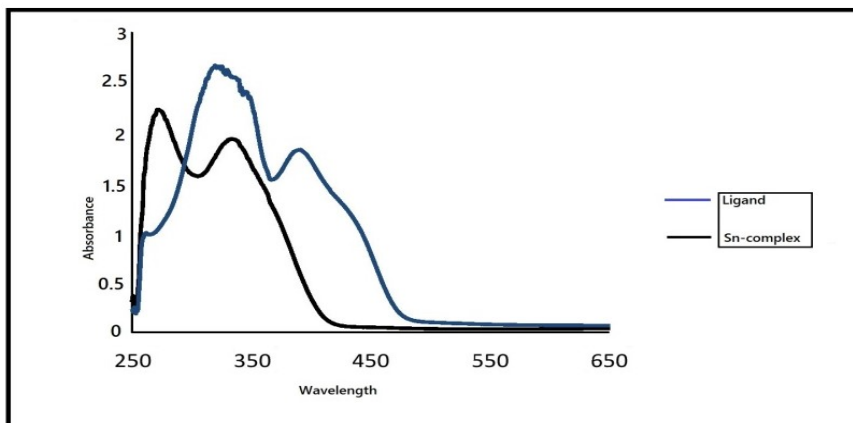
Figure 3 Electronic spectra of Sn Complex.
