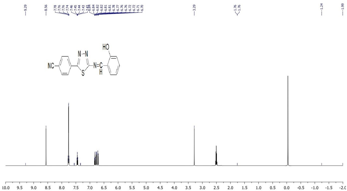
Figure 4 ^1\text{H} NMR spectra of Ligand.
