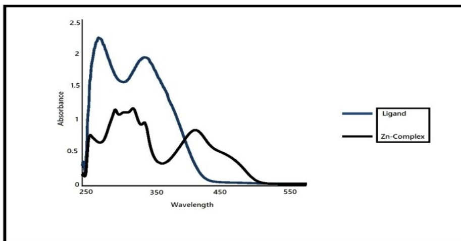
Figure 2 Electronic spectra of Zn Complex.
