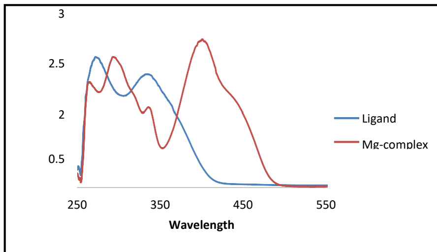
Figure 1 Electronic spectra of Mg Complex.
