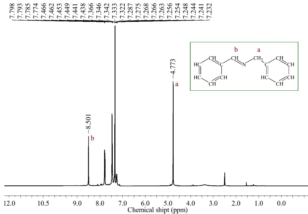
Fig. S1 – 1 H NMR of imine
