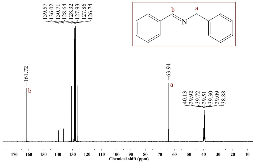
Fig. S2 – ^{13}\text{C} NMR of imine
