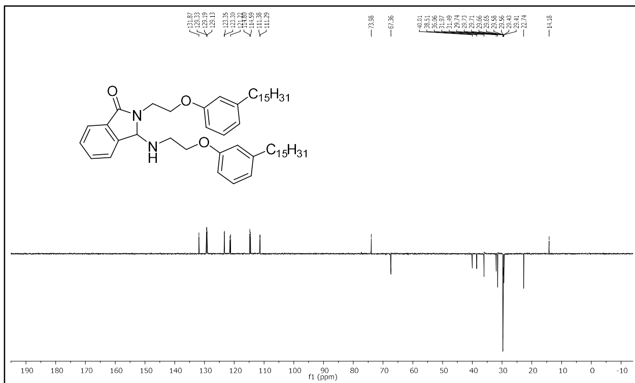
DEPT-135 spectrum of 2-(2-(3-pentadecylphenoxy)ethyl)-3-((2-(3-pentadecylphenoxy)ethyl)amino)isoindolin-1-one 3a .
