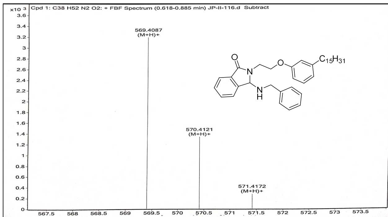
HRMS spectrum of 3-(benzylamino)-2-(2-(3-pentadecylphenoxy)ethyl)isoindolin-1-one 2 .
