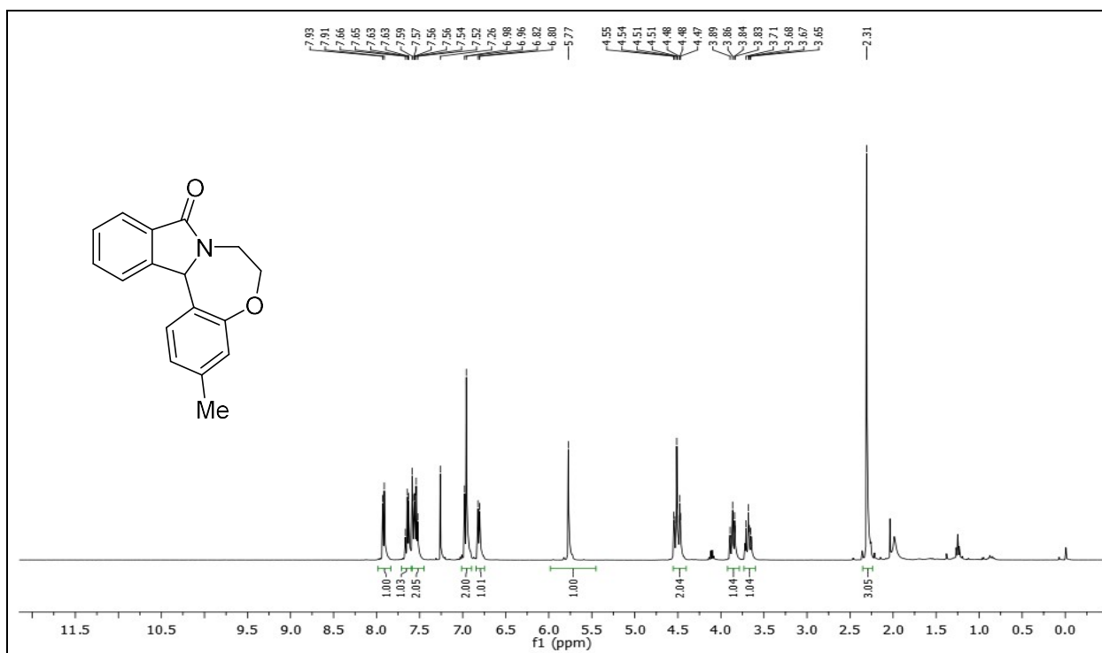
1 H NMR(400 MHz, CDCl 3 ) spectrum of 3-methyl-6,7-dihydrobenzo[6,7][1,4]oxazepino[5,4- a ]isoindol-9(13bH)-one 10b .
