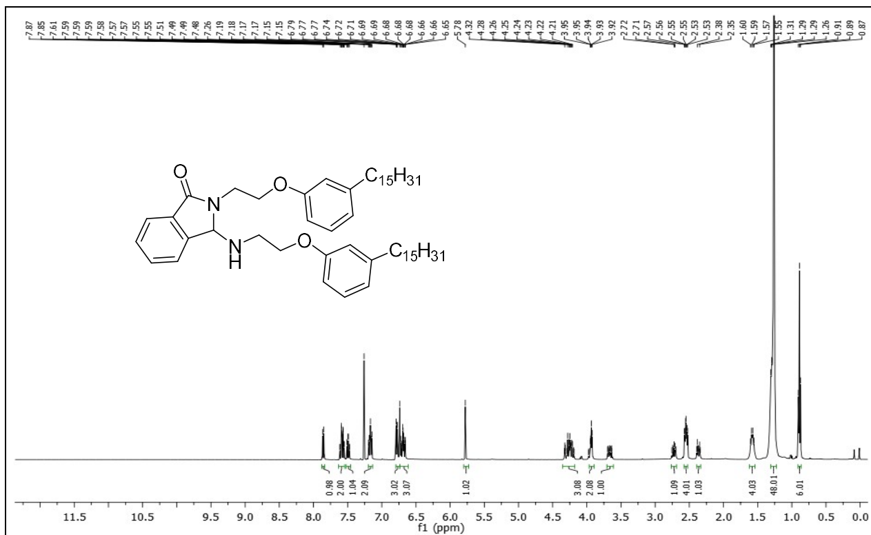
1 H NMR (400 MHz, CDCl 3 ) spectrum of 2-(2-(3-pentadecylphenoxy)ethyl)-3-((2-(3-pentadecylphenoxy)ethyl)amino)isoindolin-1-one 3a .
