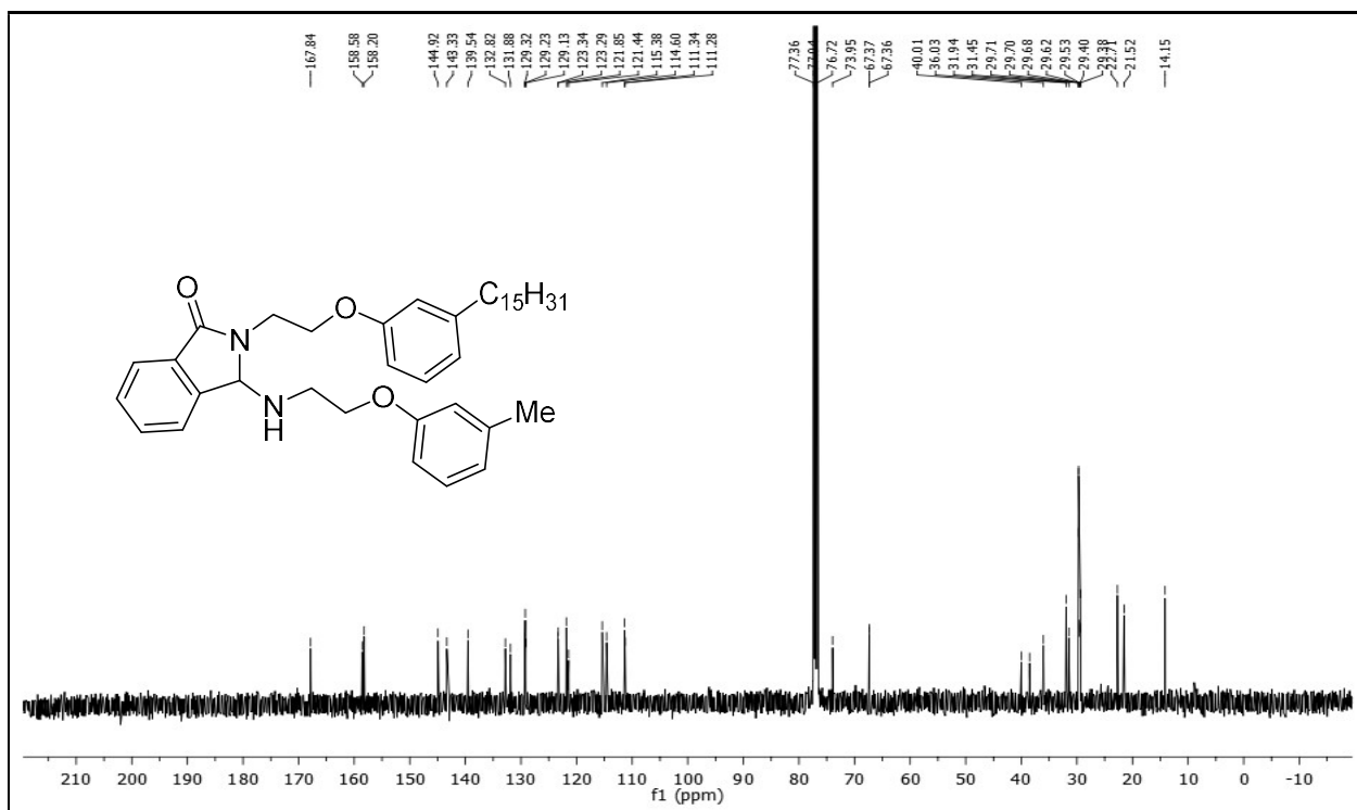
13 C NMR (100 MHz, CDCl 3 ) spectrum of 2-(2-(3-pentadecylphenoxy)ethyl)-3-((2-( m -tolylloxy)ethyl)amino)isoindolin-1-one 3c .
