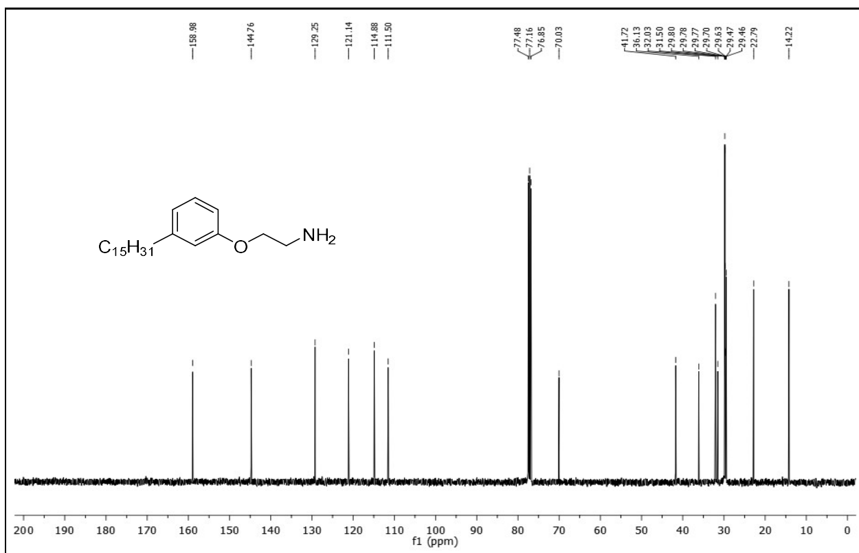
13 C NMR (100 MHz, CDCl 3 ) spectrum of 2-(3-pentadecylphenoxy)ethan-1-amine 6a .
