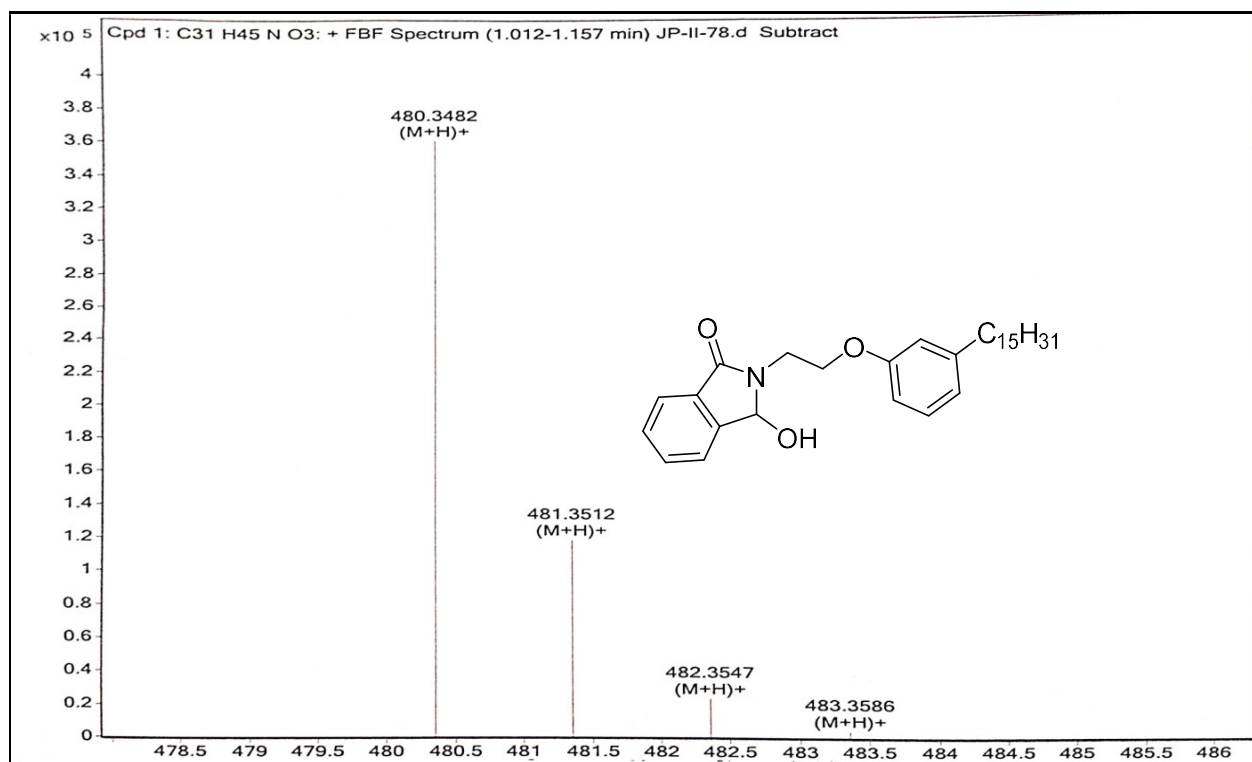
HRMS spectrum of 3-hydroxy-2-(2-(3-pentadecylphenoxy)ethyl)isoindolin-1-one 7a .
