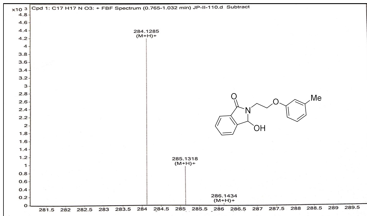
HRMS spectrum of 3-hydroxy-2-(2-( m -tolylloxy)ethyl)isoindolin-1-one 7b .
