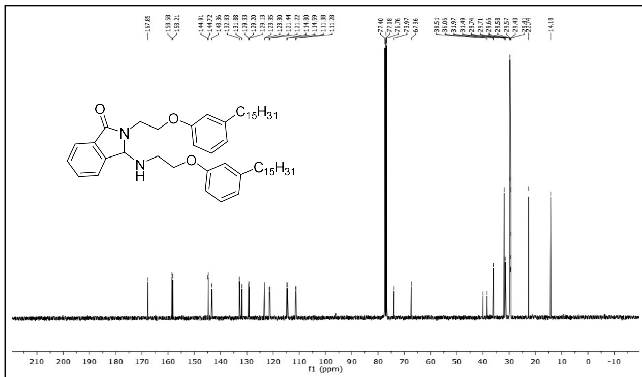
13 C NMR (100 MHz, CDCl 3 ) spectrum of 2-(2-(3-pentadecylphenoxy)ethyl)-3-((2-(3-pentadecylphenoxy)ethyl)amino)isoindolin-1-one 3a .
