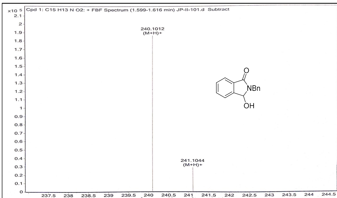
HRMS spectrum of 2-benzyl-3-hydroxyisoindolin-1-one 8 .
