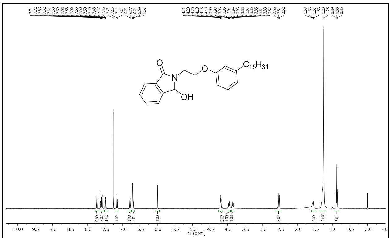
1 H NMR (400 MHz, CDCl 3 ) spectrum of 3-hydroxy-2-(2-(3-pentadecylphenoxy)ethyl)isoindolin-1-one (7a).
