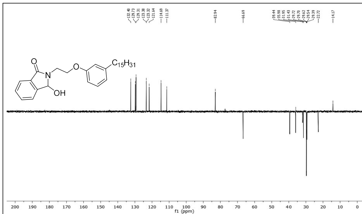
DEPT-135 spectrum of 3-hydroxy-2-(2-(3-pentadecylphenoxy)ethyl)isoindolin-1-one 7a .
