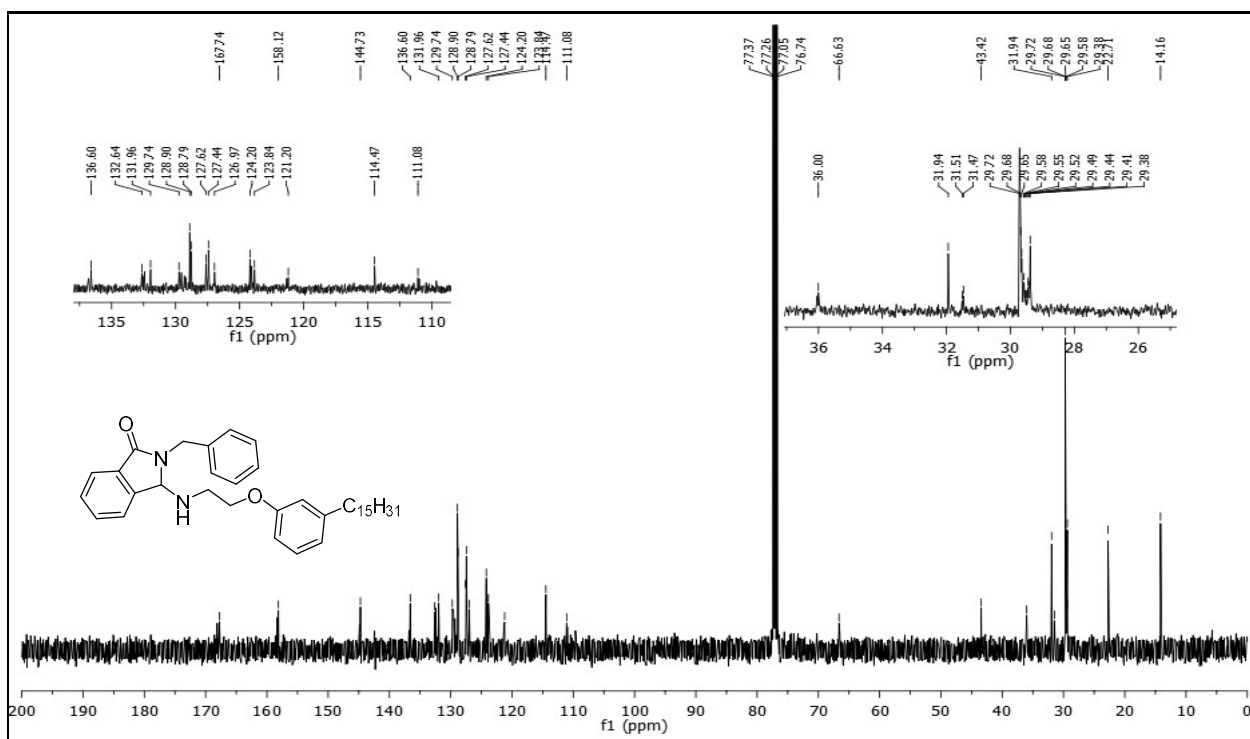
13 C NMR (100 MHz, CDCl 3 ) spectrum of 2-benzyl-3-((2-(3-pentadecylphenoxy)ethyl)amino)isoindolin-1-one 9 .
