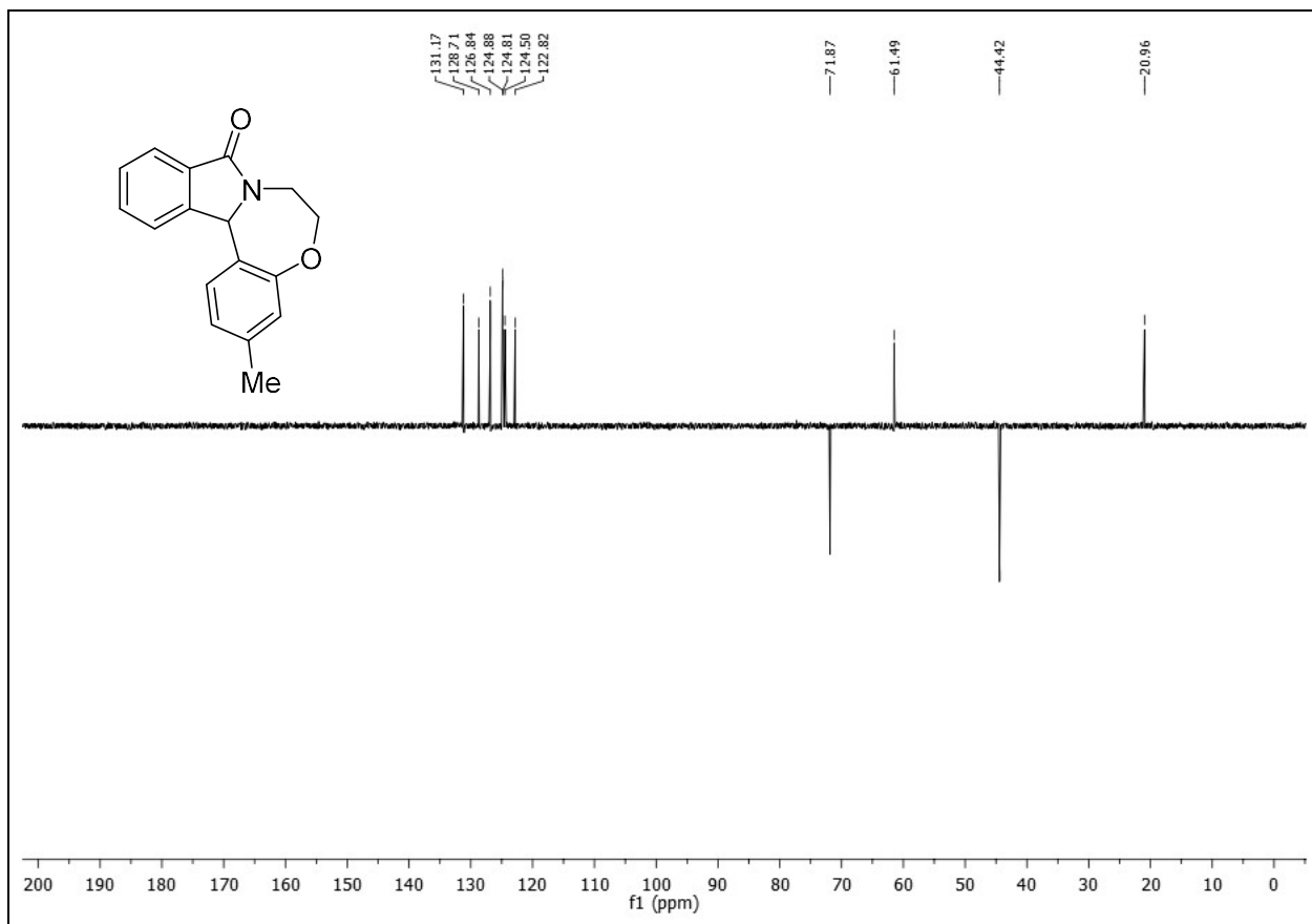
DEPT-135 spectrum of 3-methyl-6,7-dihydrobenzo[6,7][1,4]oxazepino[5,4-a]isoindol-9(13bH)-one 10b .
