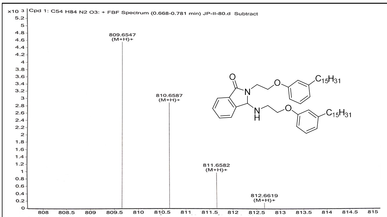
HRMS spectrum of 2-(2-(3-pentadecylphenoxy)ethyl)-3-((2-(3-pentadecyl phenoxy)ethyl)amino)isoindolin-1-one 3a .
