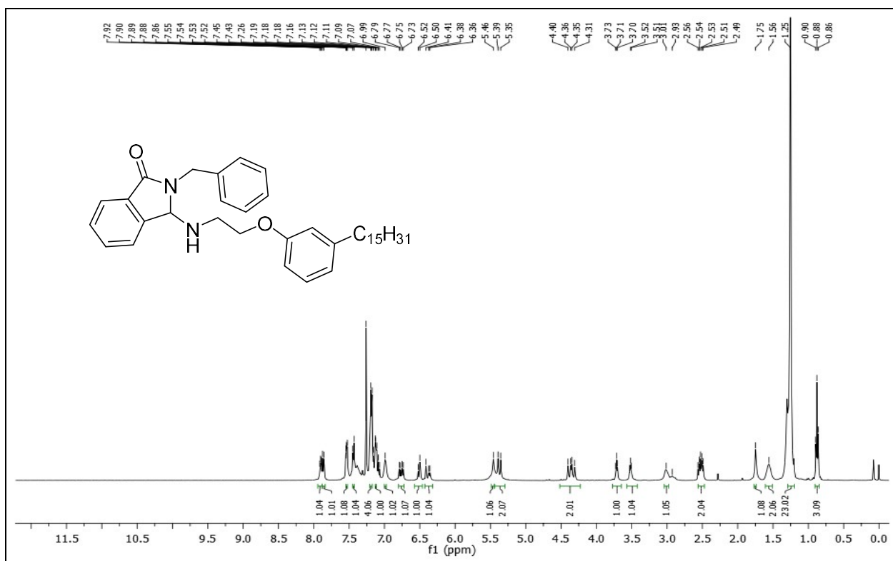
1 H NMR (400 MHz, CDCl 3 ) spectrum of 2-benzyl-3-((2-(3-pentadecylphenoxy)ethyl)amino)isoindolin-1-one 9 .
