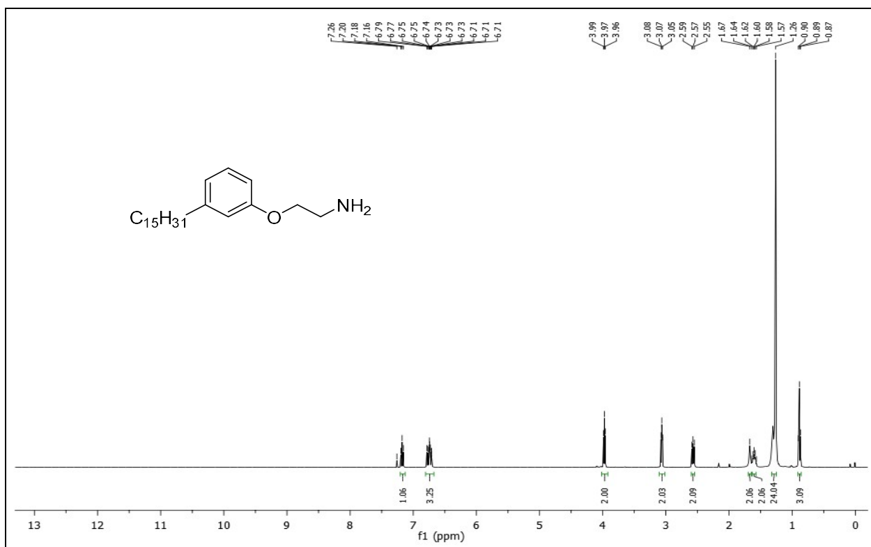
1 H NMR (400 MHz, CDCl 3 ) spectrum of 2-(3-pentadecylphenoxy)ethan-1-amine 6a .
