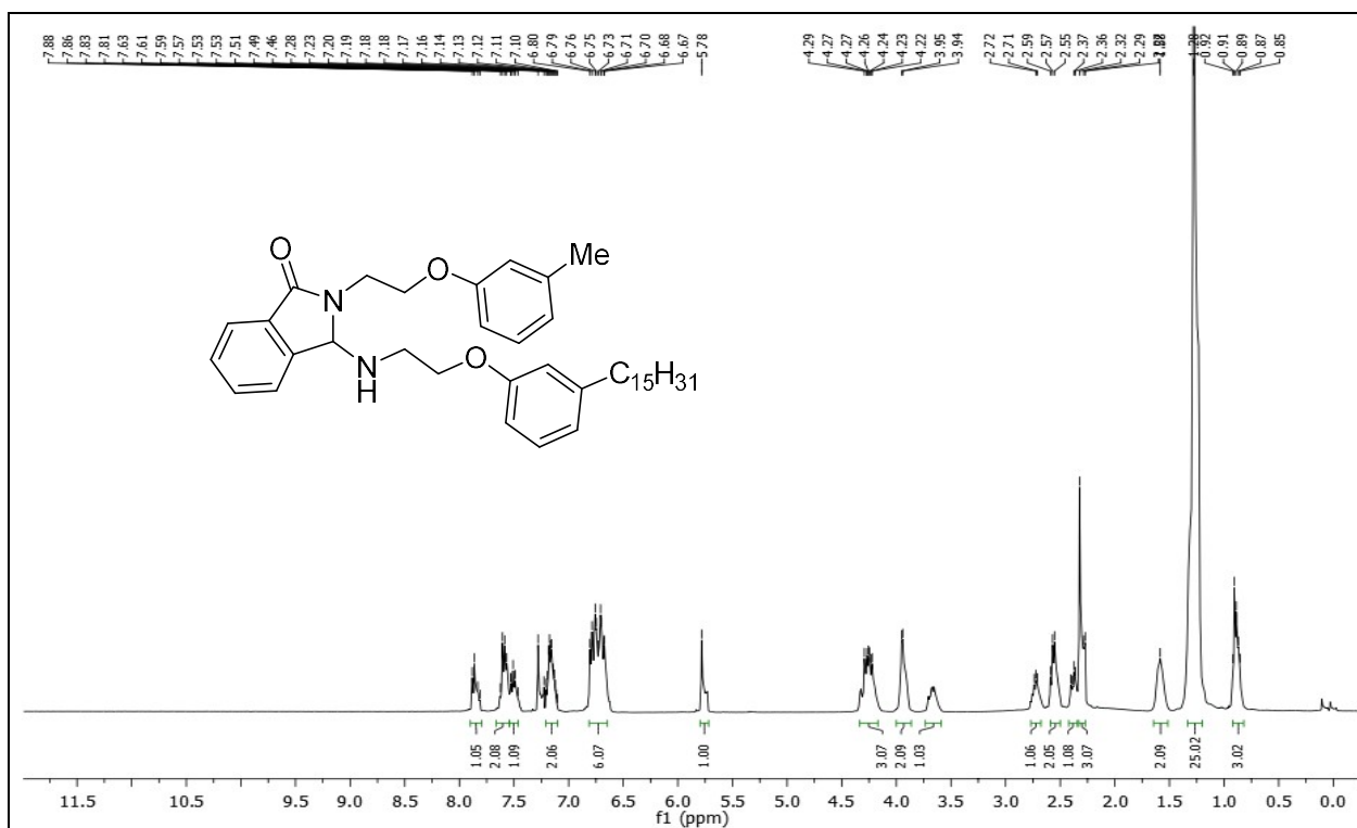
1 H NMR (400 MHz, CDCl 3 ) spectrum of 3-((2-(3-pentadecylphenoxy)ethyl)amino)-2-(2-( m -tolylloxy)ethyl)isoindolin-1-one 3b .
