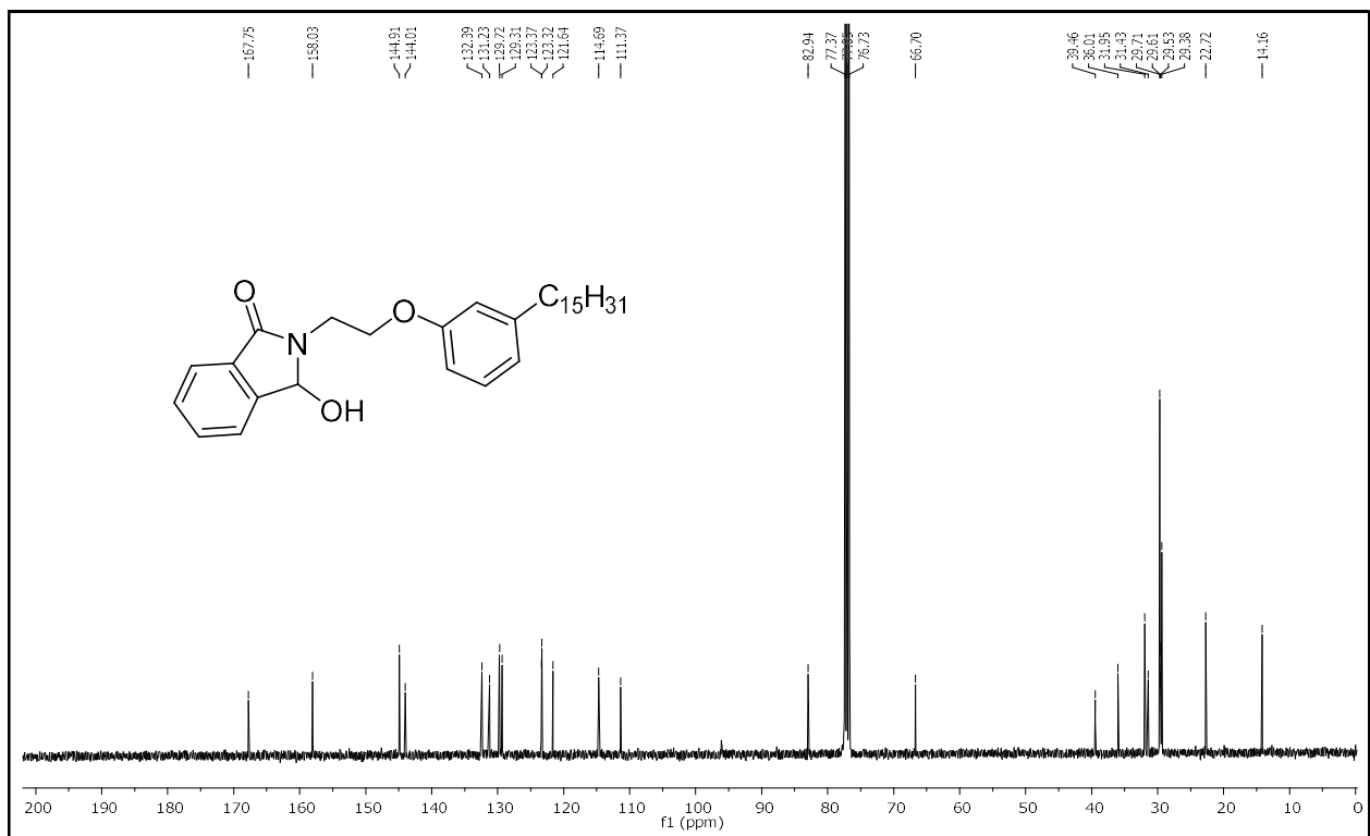
13 C NMR (100 MHz, CDCl 3 ) spectrum of 3-hydroxy-2-(2-(3-pentadecylphenoxy)ethyl)isoindolin-1-one (7a).
