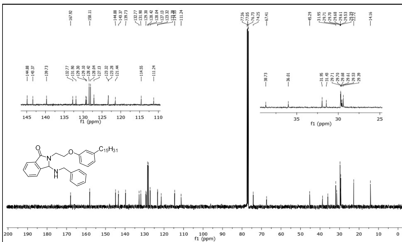
13 C NMR (100 MHz, CDCl 3 ) spectrum of 3-(benzylamino)-2-(2-(3-pentadecylphenoxy)ethyl)isoindolin-1-one 2.
