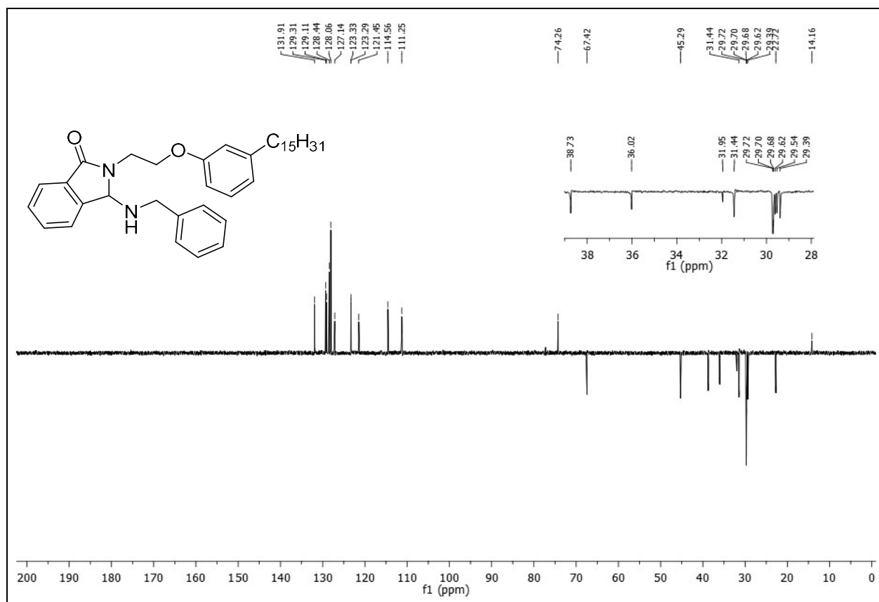
DEPT-135 spectrum of 3-(benzylamino)-2-(2-(3-pentadecylphenoxy)ethyl)isoindolin-1-one 2 .
