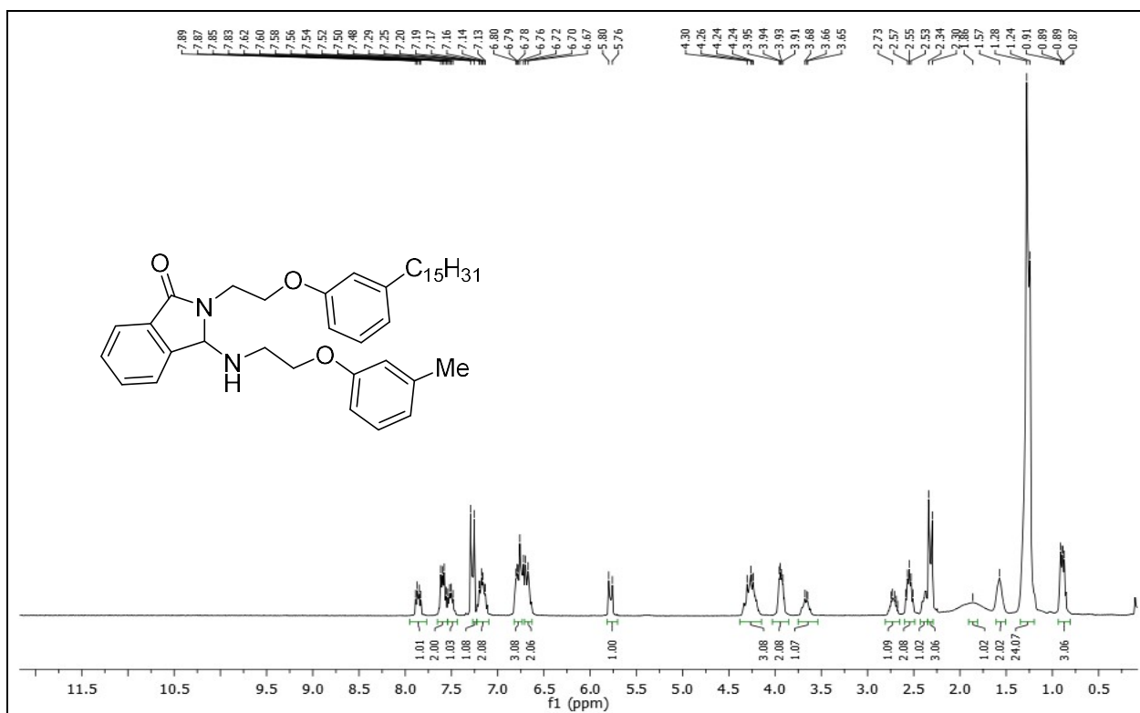
1 H NMR (400 MHz, CDCl 3 ) spectrum of 2-(2-(3-pentadecylphenoxy)ethyl)-3-((2-( m -tolylloxy)ethyl)amino)isoindolin-1-one 3c .
