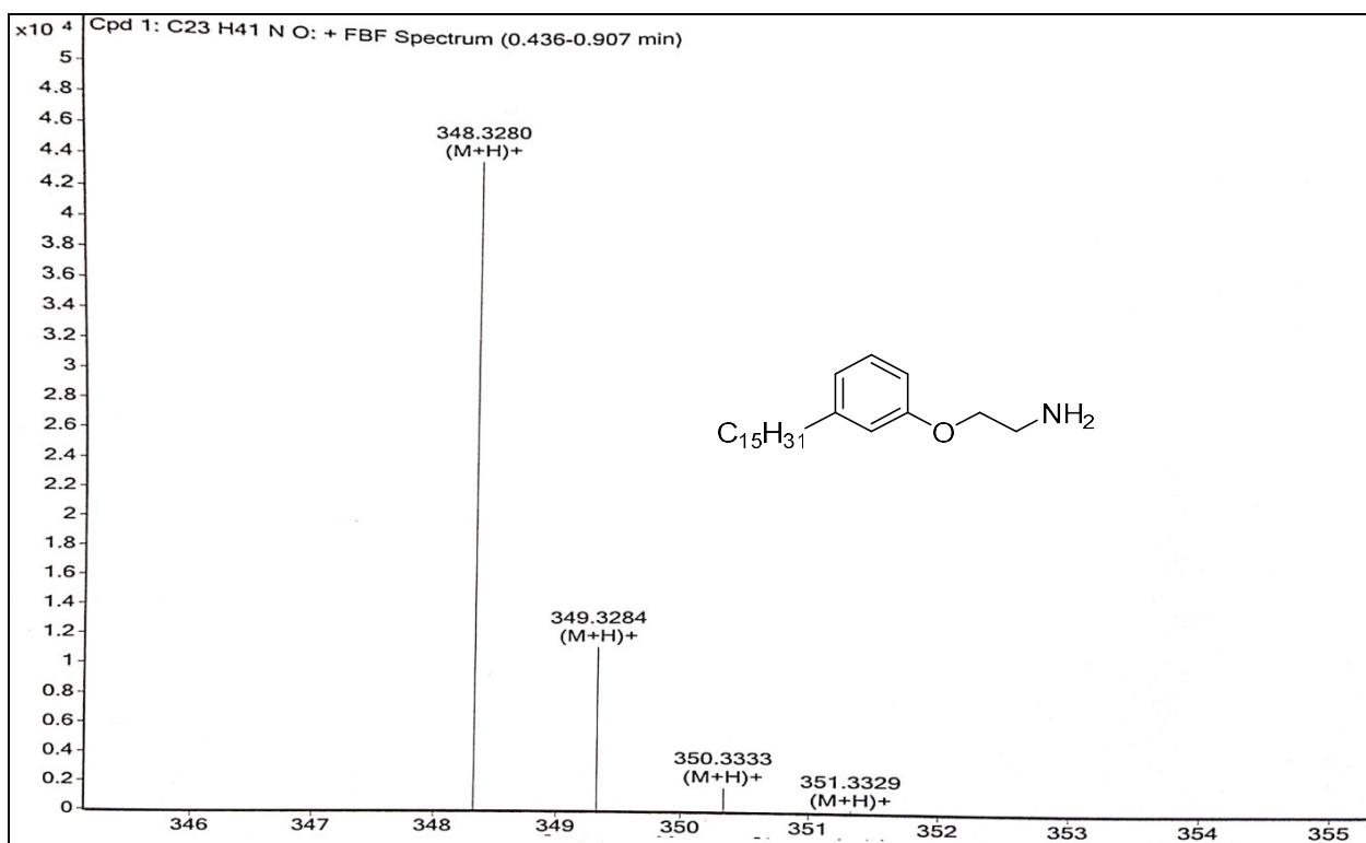
HRMS spectrum of 2-(3-pentadecylphenoxy)ethan-1-amine 6a .
