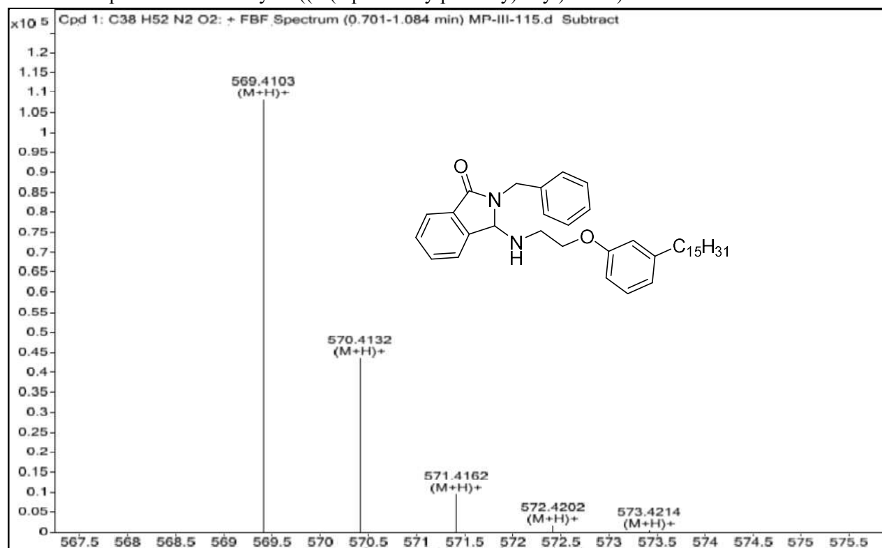
HRMS spectrum of 2-benzyl-3-((2-(3-pentadecylphenoxy)ethyl)amino)isoindolin-1-one 9 .
