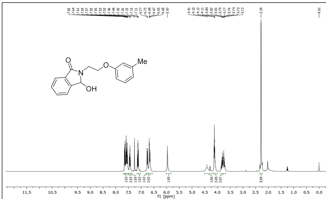
1 H NMR (400 MHz, CDCl 3 ) spectrum of 3-hydroxy-2-(2-( m -tolyl)oxy)ethylisoindolin-1-one 7b .
