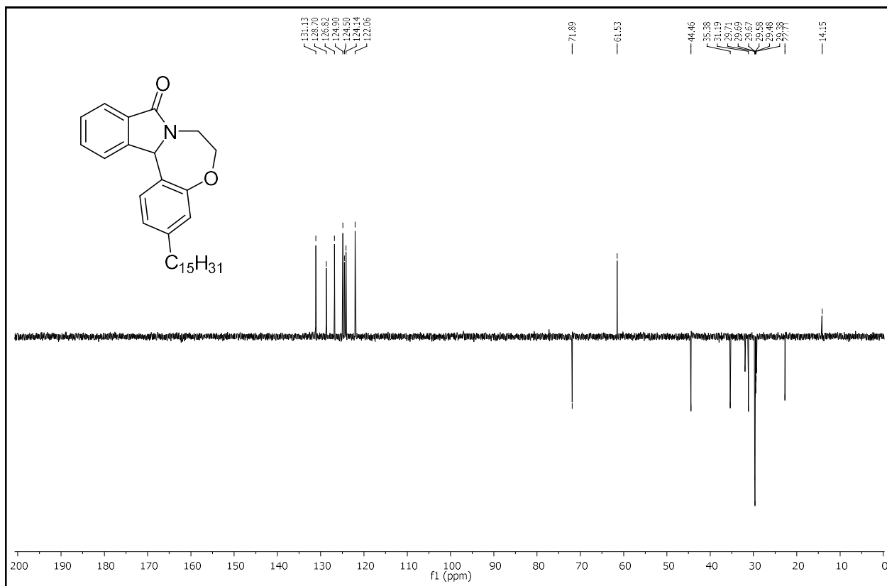
DEPT-135 spectrum of 3-pentadecyl-6,7-dihydrobenzo[6,7][1,4]oxazepino [5,4- a ]isoindol-9(13 bH )-one 10a .
