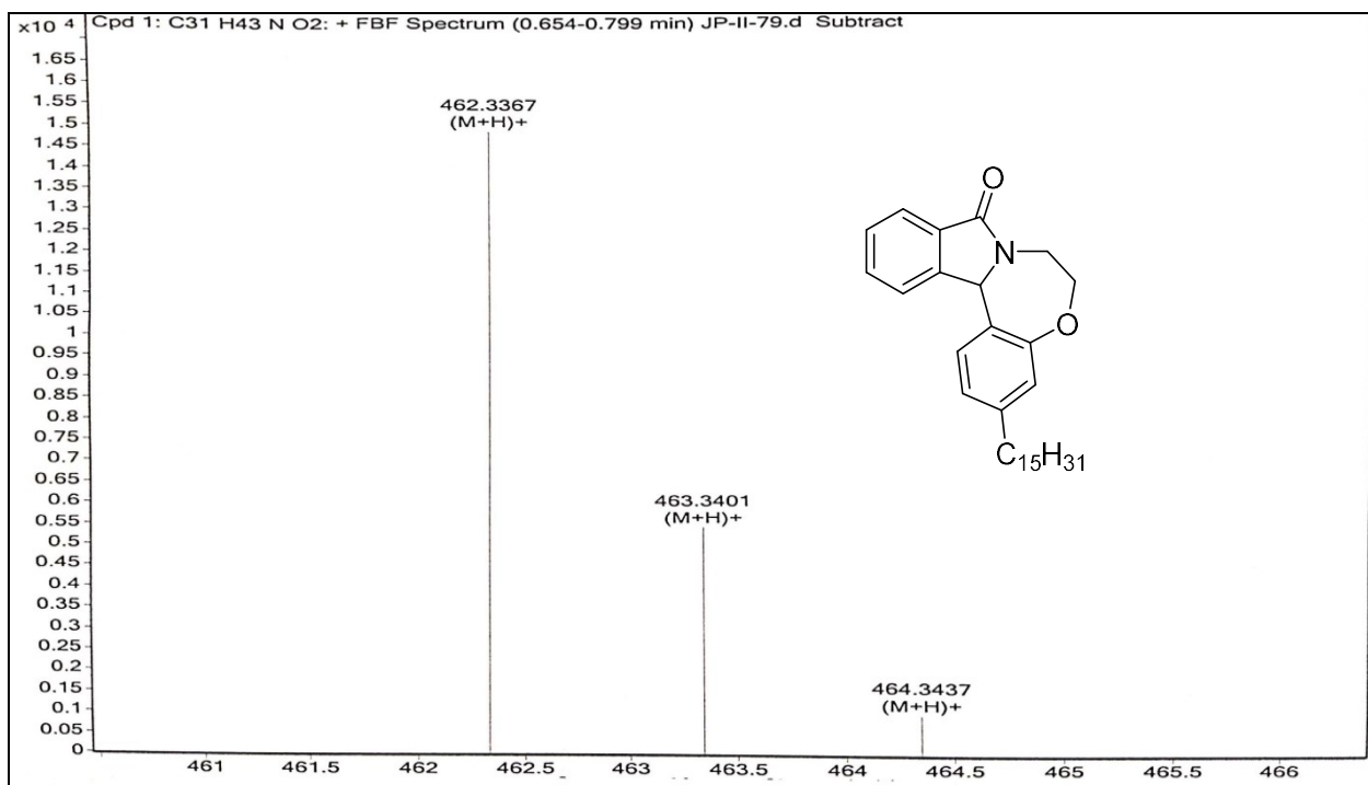
HRMS spectrum of 3-pentadecyl-6,7-dihydrobenzo[6,7][1,4]oxazepino [5,4- a ]isoindol-9(13 bH )-one 10a .
