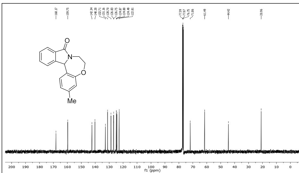
13 C NMR(100 MHz, CDCl 3 ) spectrum of 3-methyl-6,7-dihydrobenzo[6,7][1,4]oxazepino[5,4- a ]isoindol-9(13bH)-one 10b .
