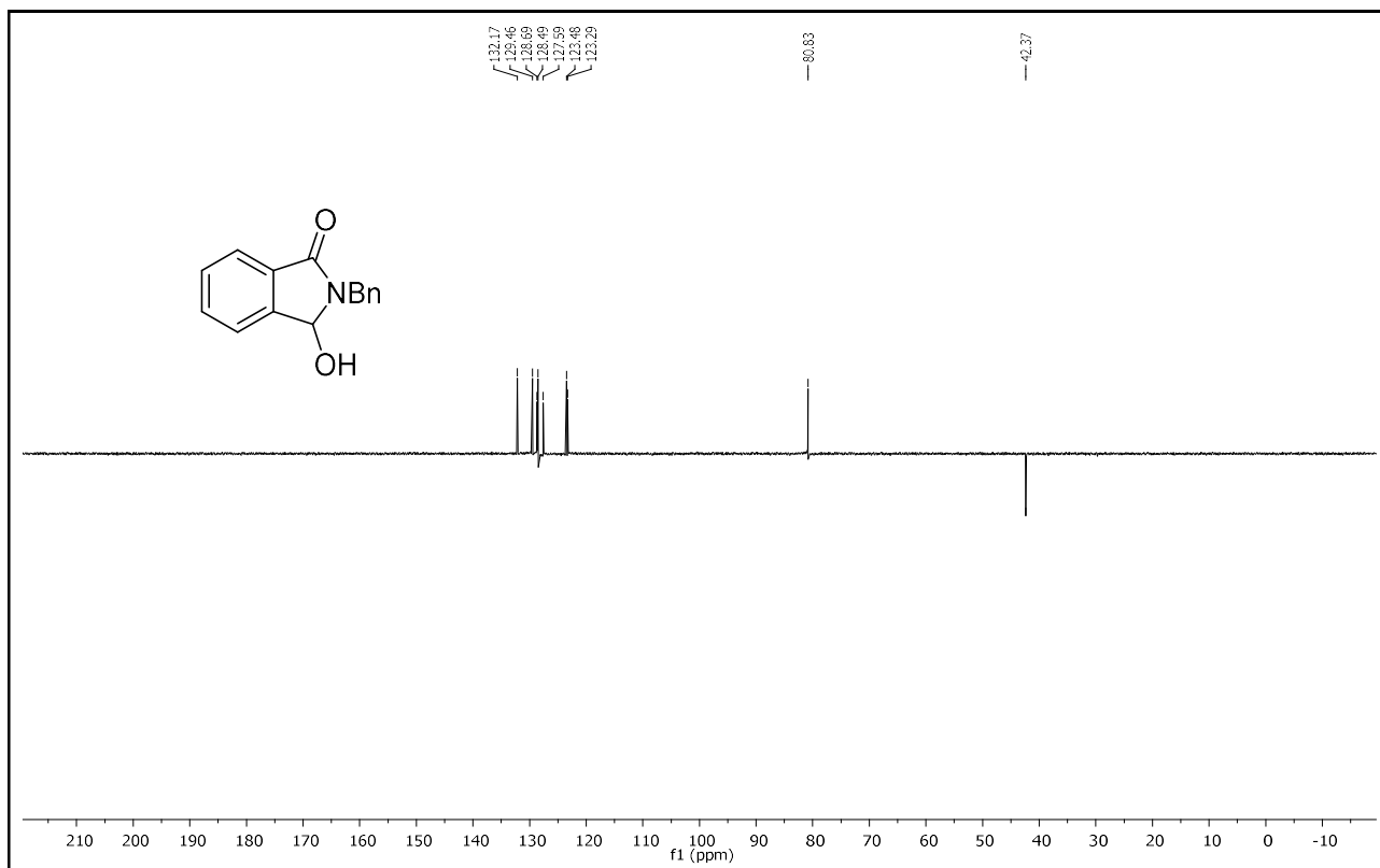
DEPT-135 spectrum of 2-benzyl-3-hydroxyisoindolin-1-one 8 .
