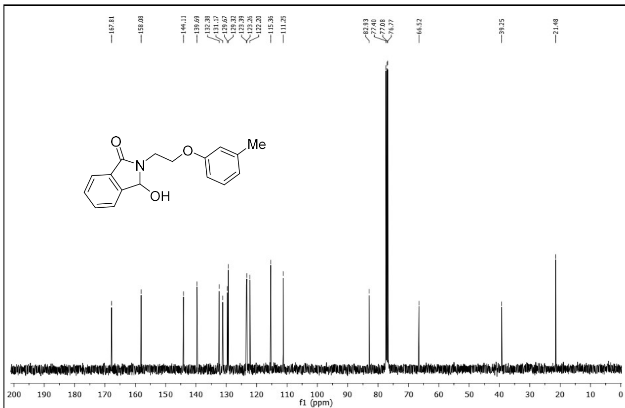
13 C NMR (100 MHz, CDCl 3 ) spectrum of 3-hydroxy-2-(2-( m -tolyl)oxy)ethylisoindolin-1-one 7b .
