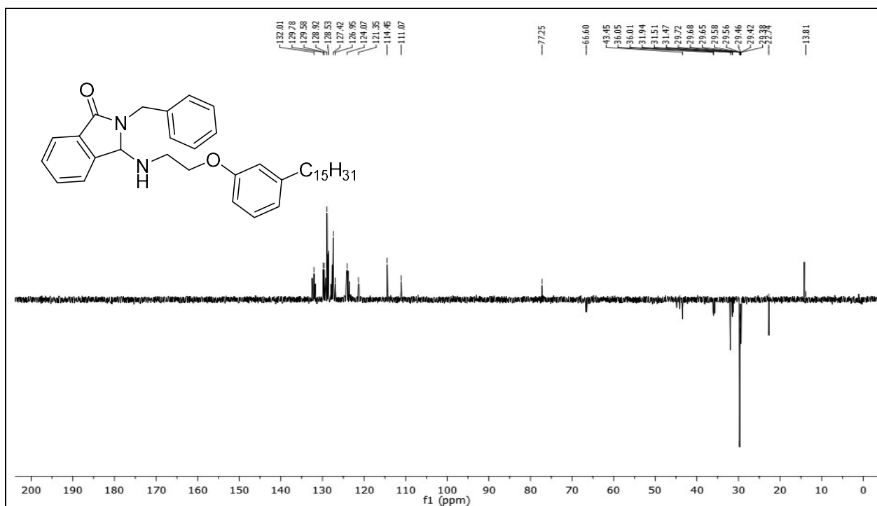
DEPT-135 spectrum of 2-benzyl-3-((2-(3-pentadecylphenoxy)ethyl)amino)isoindolin-1-one 9 .
