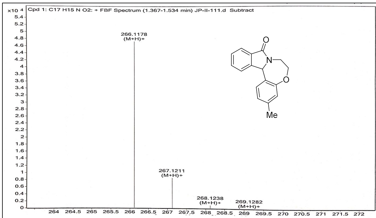
HRMS spectrum of 3-methyl-6,7-dihydrobenzo[6,7][1,4]oxazepino[5,4-a]isoindol-9(13bH)-one 10b .
