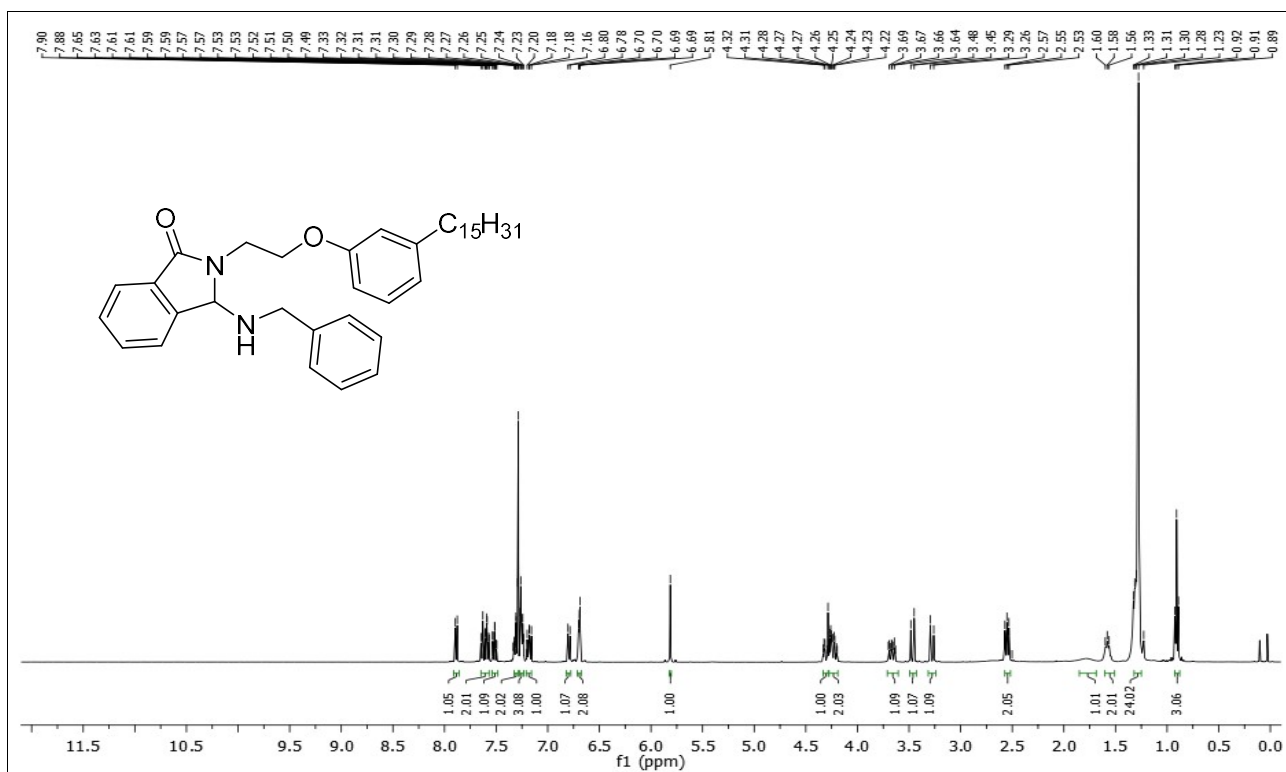
1 H NMR (400 MHz, CDCl 3 ) spectrum of 3-(benzylamino)-2-(2-(3-pentadecylphenoxy)ethyl)isoindolin-1-one 2.
