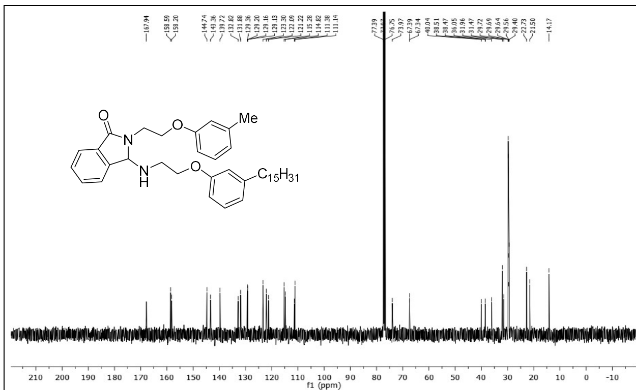
13 C NMR (100 MHz, CDCl 3 ) spectrum of 3-((2-(3-pentadecylphenoxy)ethyl)amino)-2-(2-( m -tolylloxy)ethyl)isoindolin-1-one 3b .
