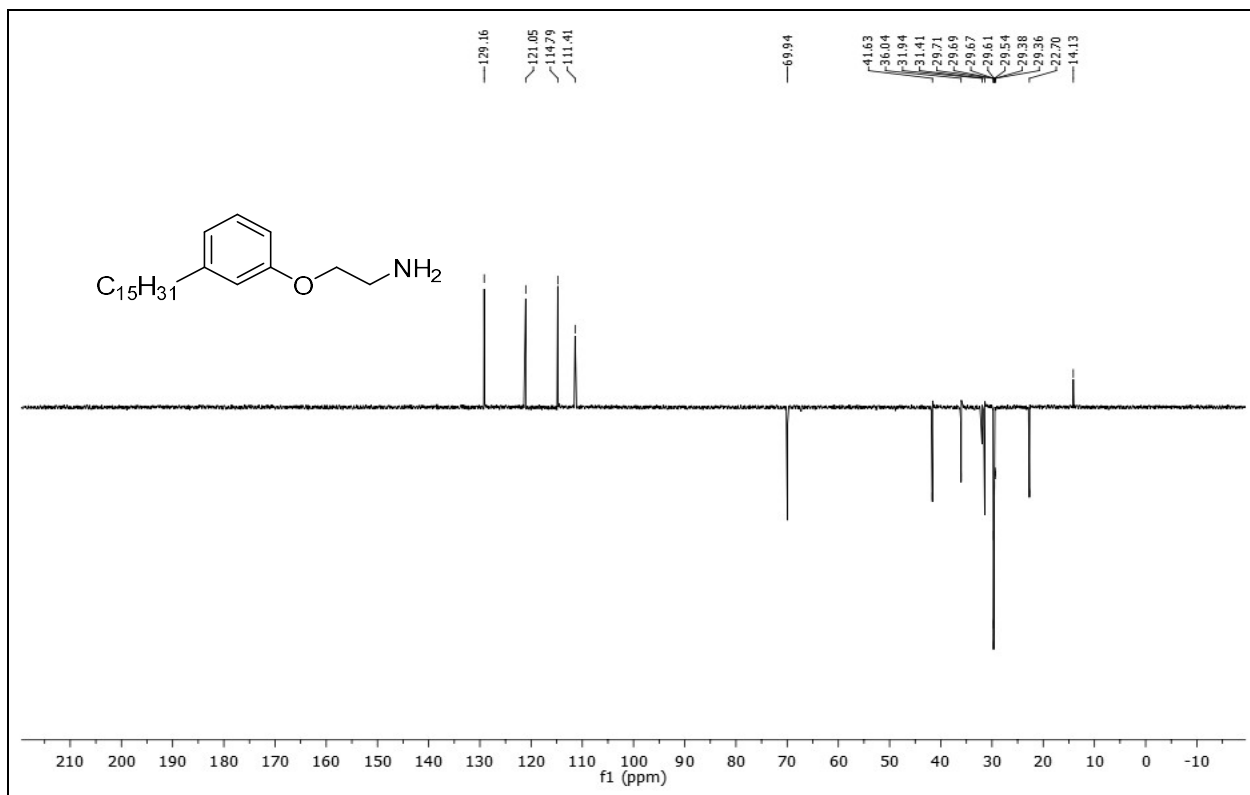
DEPT-135 spectrum of 2-(3-pentadecylphenoxy)ethan-1-amine 6a .
