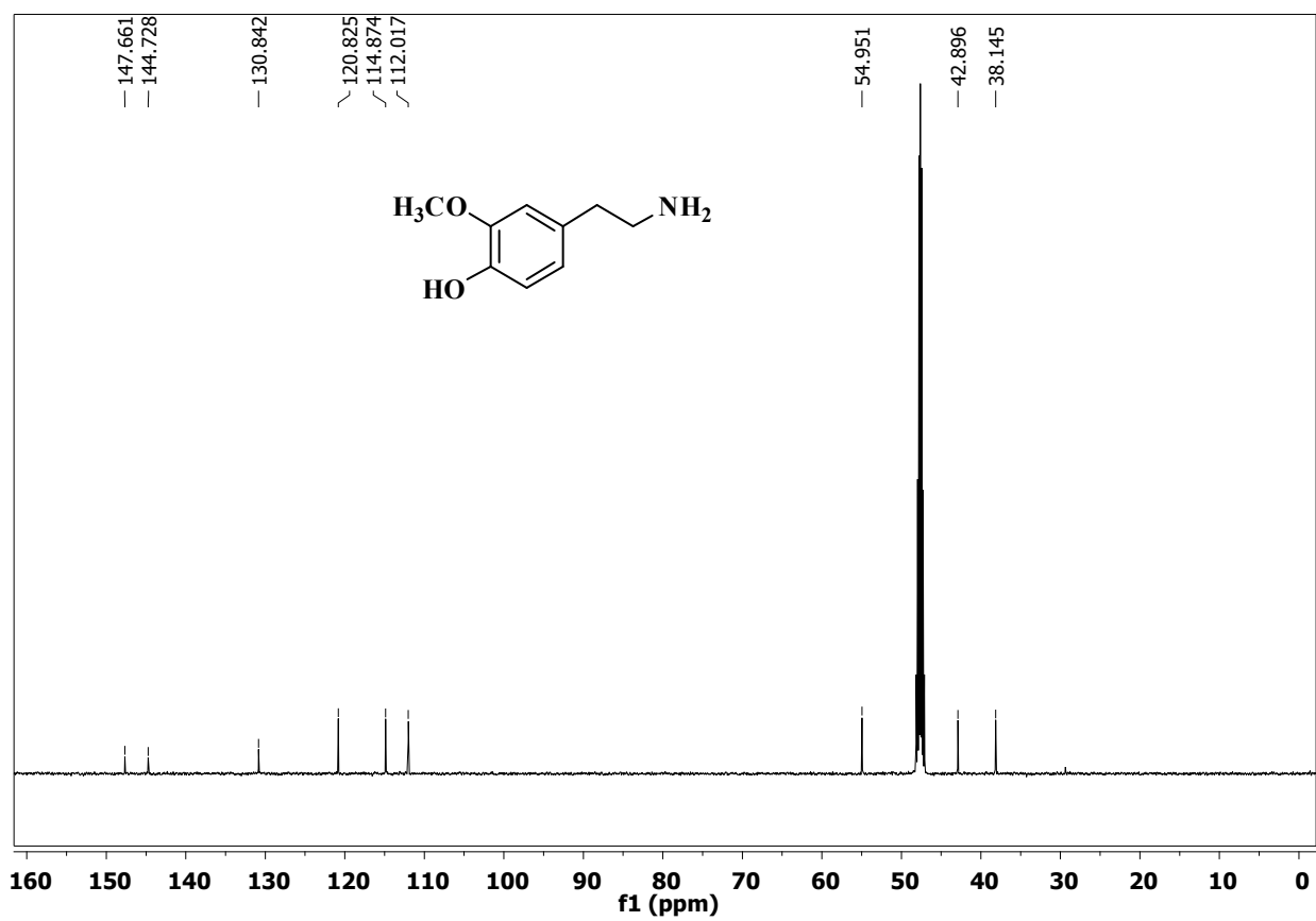
^{13}\text{C} NMR spectrum of compound 8 in \text{CD}_3\text{OD} (126 MHz)
