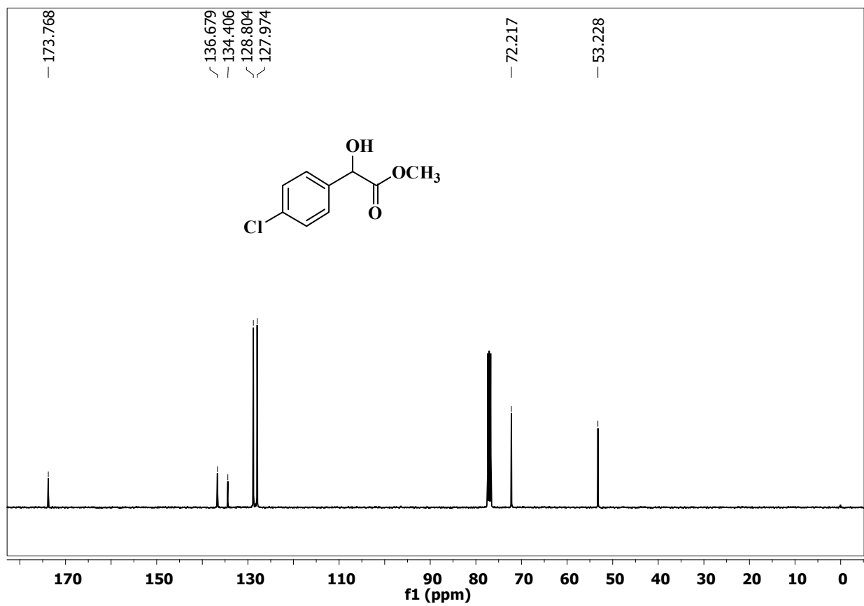
^{13}\text{C} NMR spectrum of compound 3 in \text{CDCl}_3 (101 MHz)
