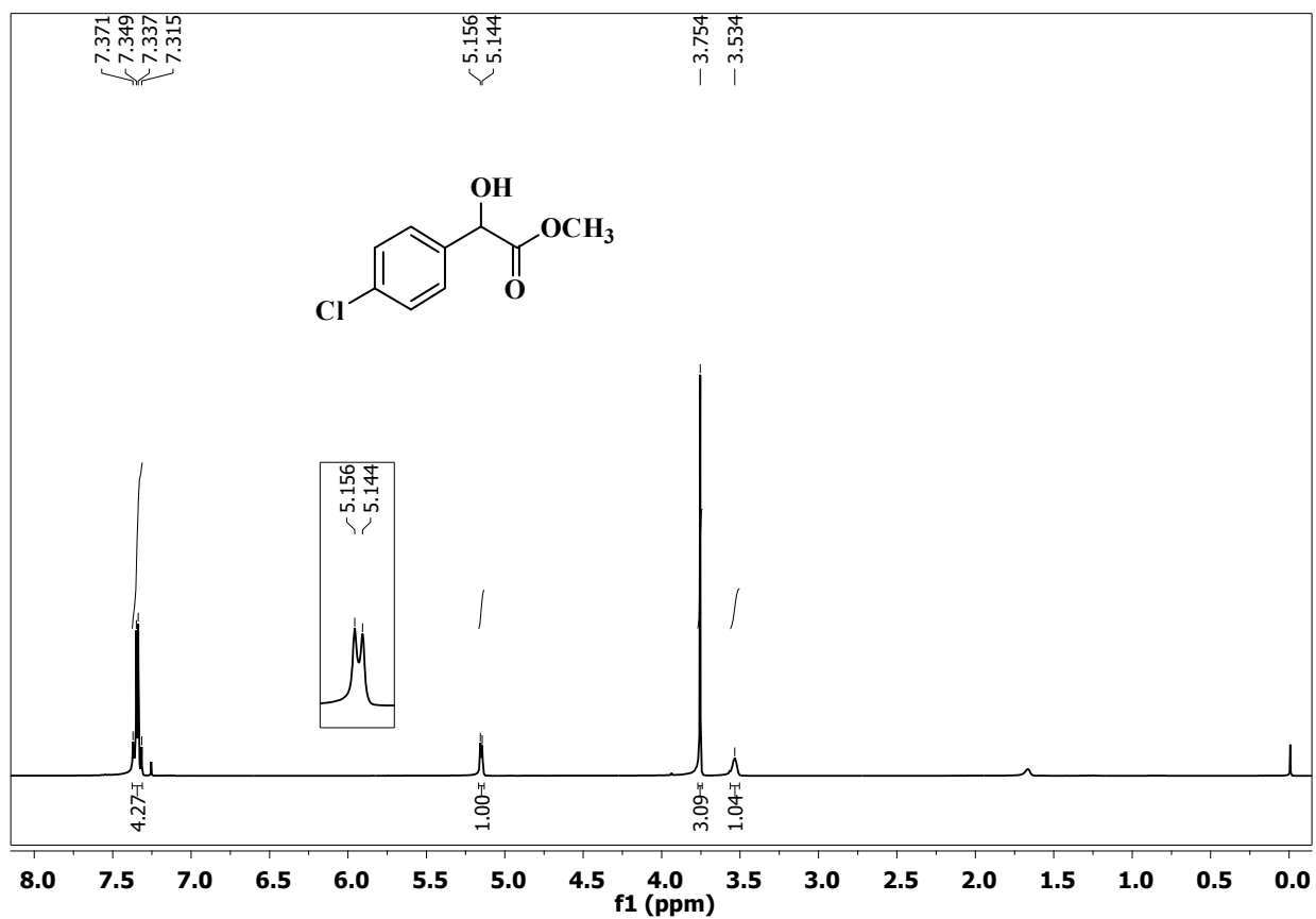
^1\text{H} NMR spectrum of compound 3 in \text{CDCl}_3 (400 MHz)
