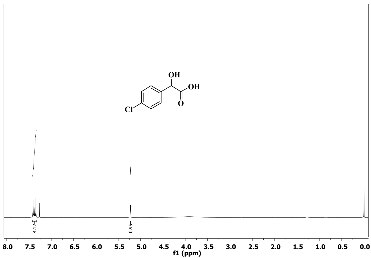
^1\text{H} NMR spectrum of compound 2 in \text{CDCl}_3 (400 MHz)
