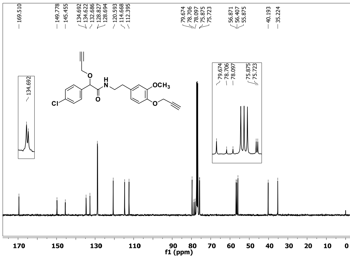
13 C NMR spectrum of Mandipropamid in CDCl 3 (101 MHz)
