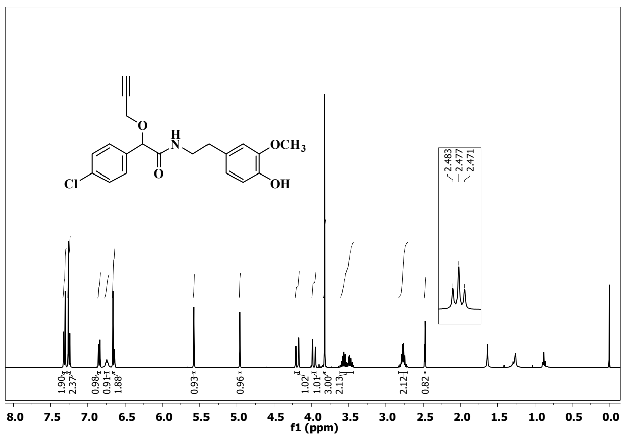
1 H NMR spectrum of compound 9 in CDCl 3 (400 MHz)
