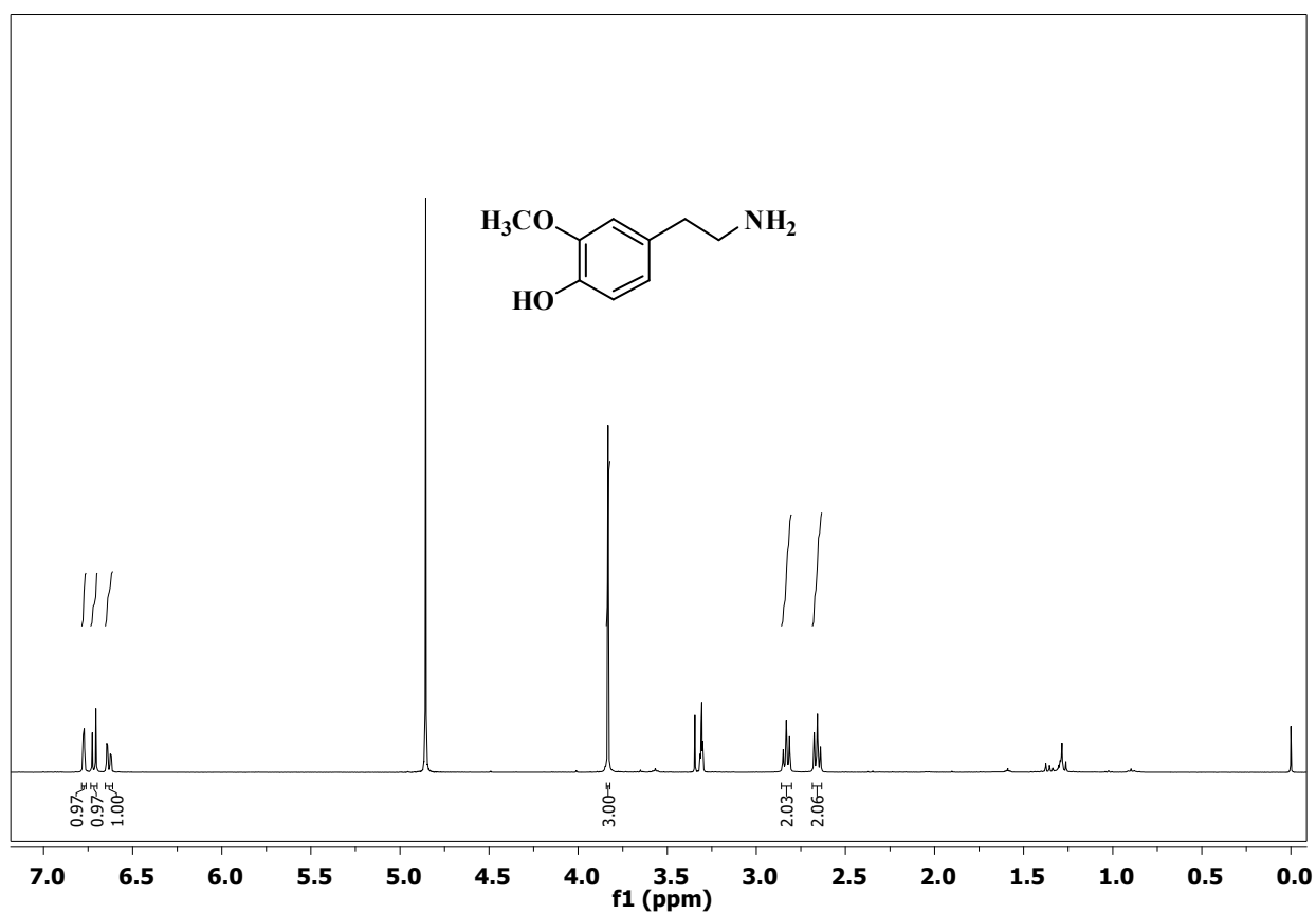
1 H NMR spectrum of compound 8 in CD 3 OD (400 MHz)
