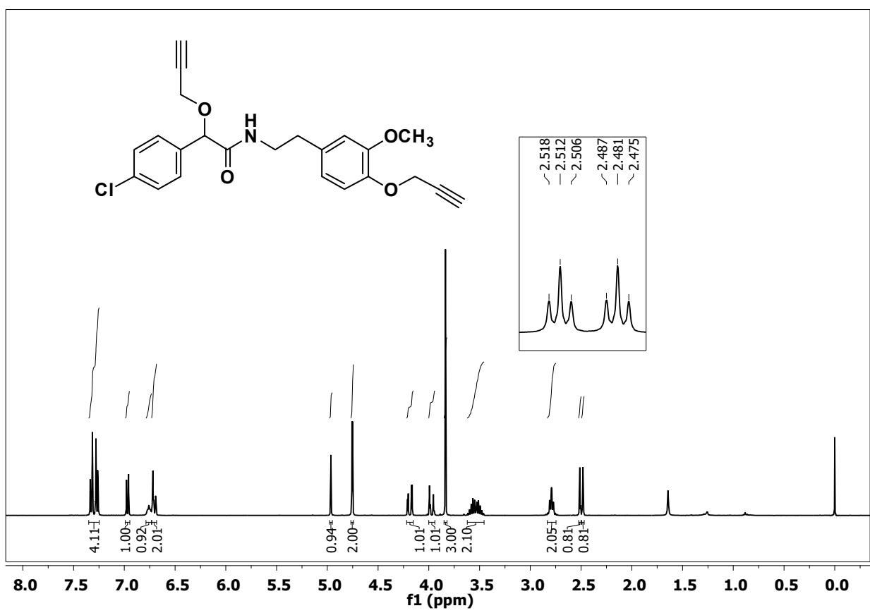
1 H NMR spectrum of Mandipropamid in CDCl 3 (400 MHz)
