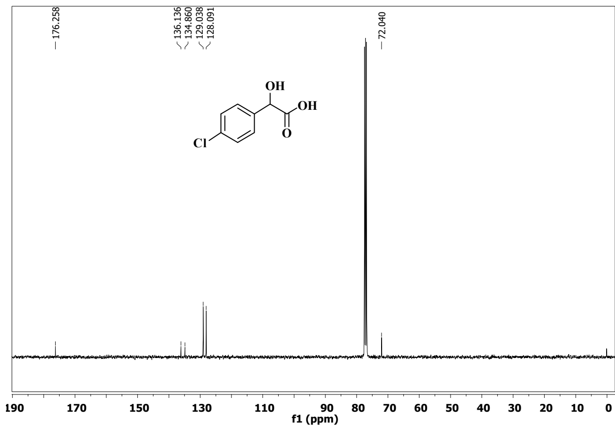
^{13}\text{C} NMR spectrum of compound 2 in \text{CDCl}_3 (101 MHz)
