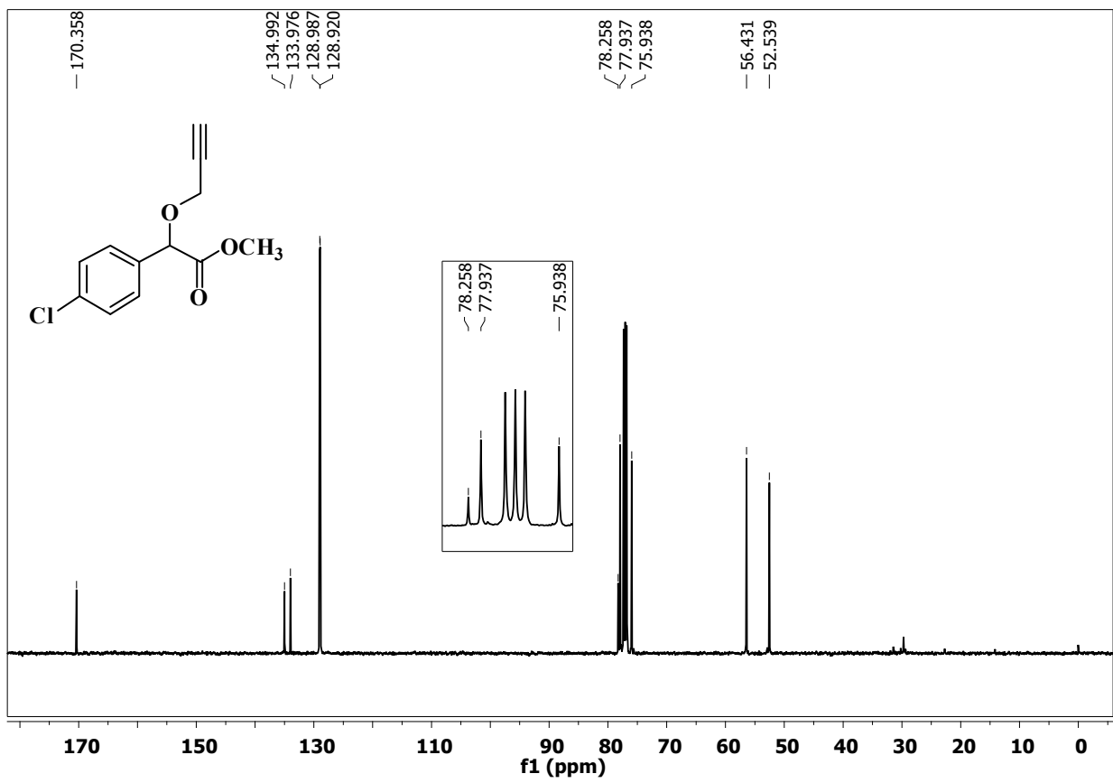
^{13}\text{C} NMR spectrum of compound 4 in \text{CDCl}_3 (126 MHz)
