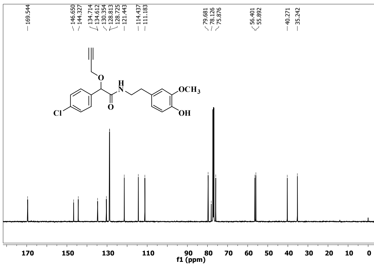
^{13}\text{C} NMR spectrum of compound 9 in \text{CDCl}_3 (126 MHz)
