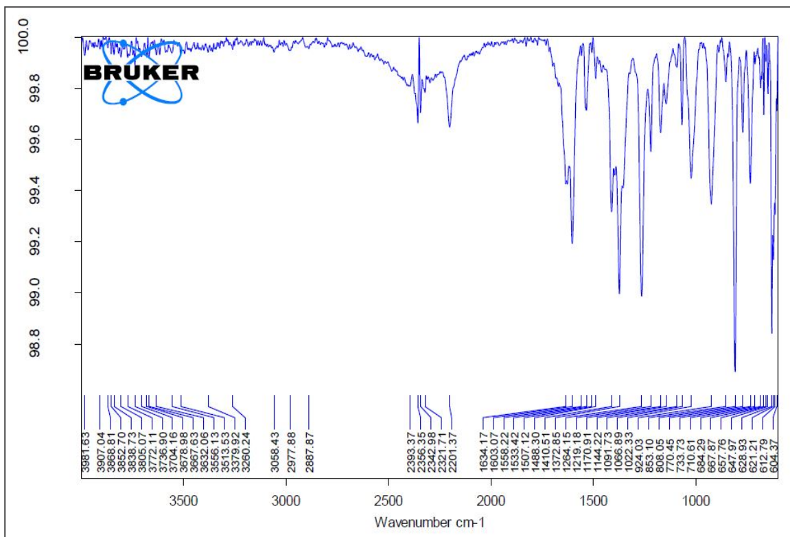
Figure S3. IR spectrum of [Zn(4,4-Bipy) 2 (CED)] (3)
