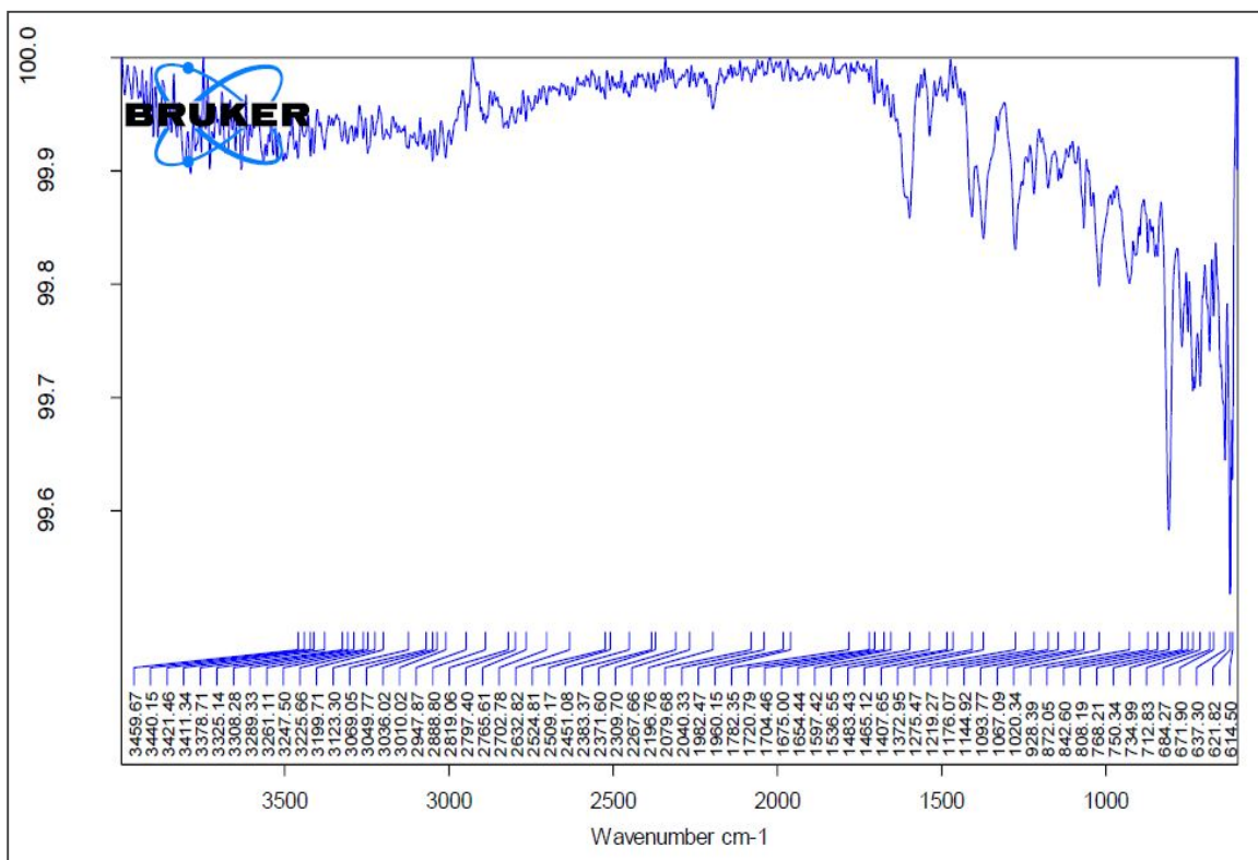
Figure S4. IR spectrum of [Cd(4,4-Bipy) 2 (CED)] (4)
