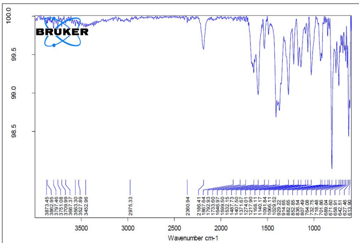
Figure S2. IR spectrum of [Co(4,4-Bipy) 2 (CED)] (2)
