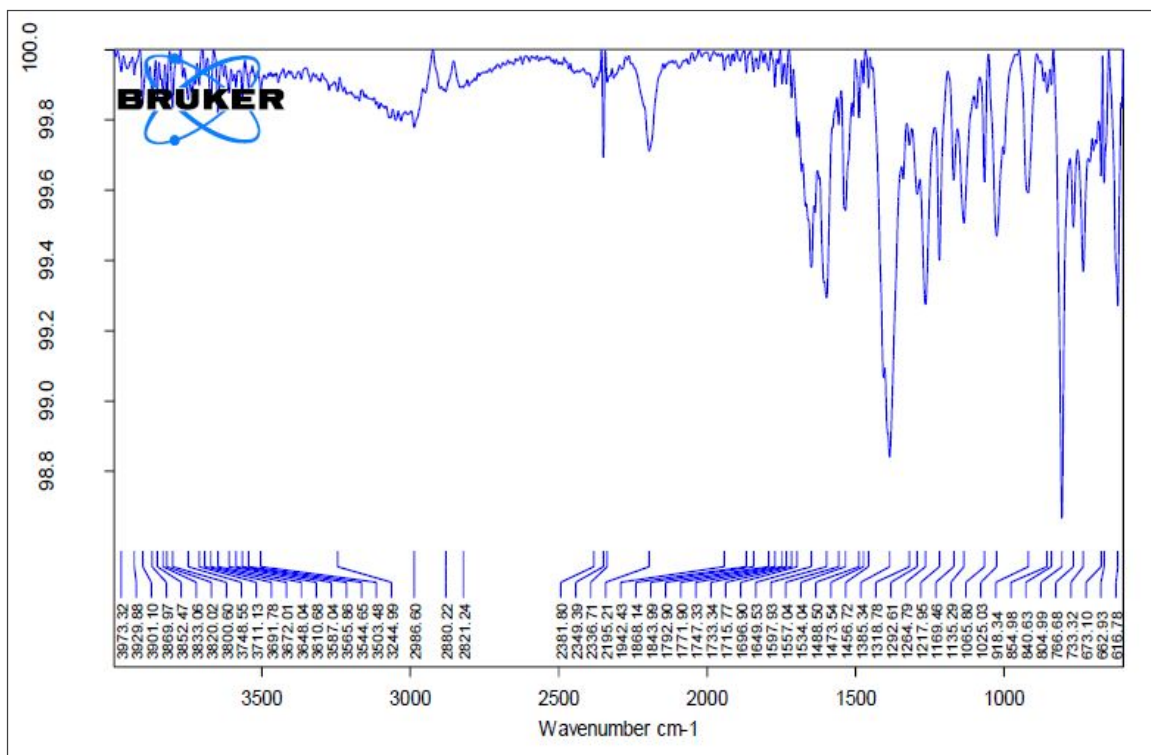
Figure S1. IR spectrum of [Ni(4,4-Bipy) 2 (CED)] (1)
