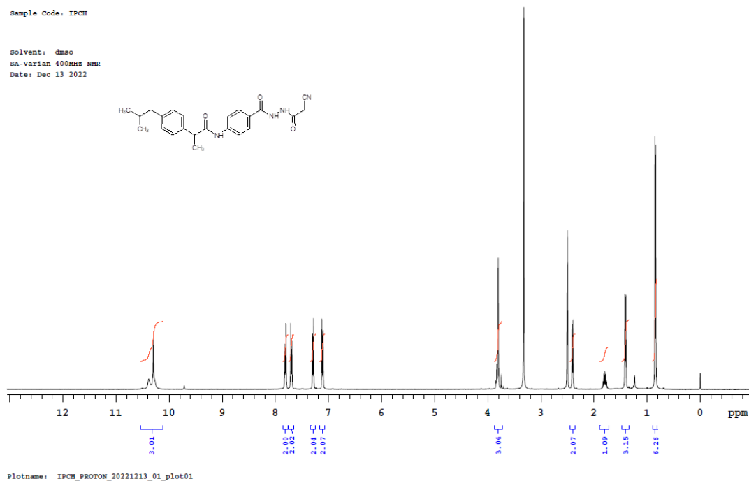
Fig 2: 1 H-NMR spectrum of 5
