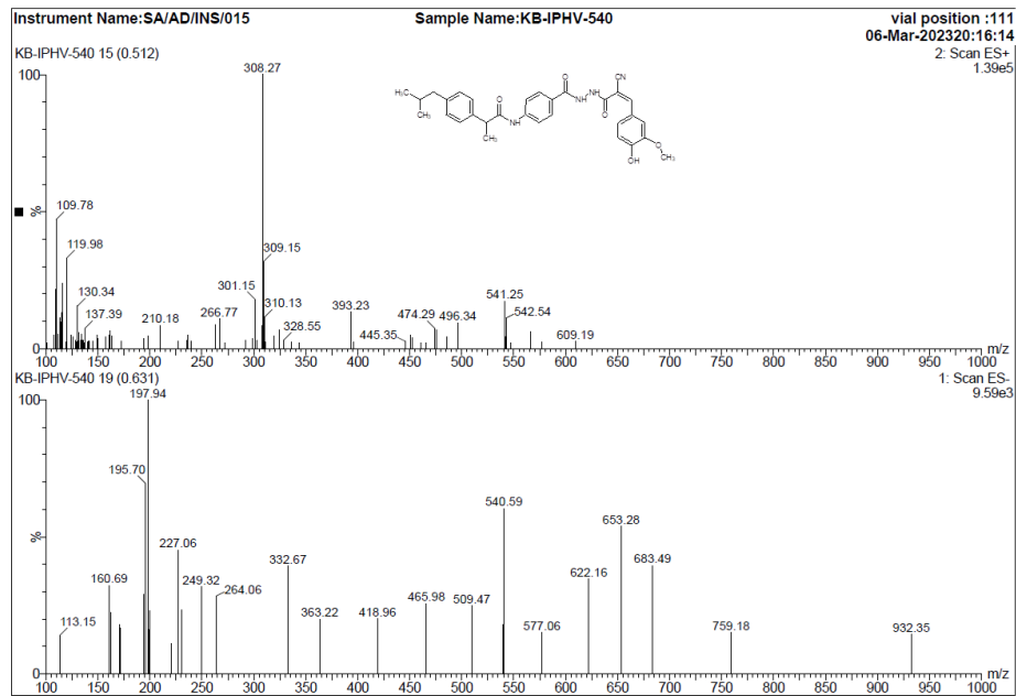
Fig 8: Mass spectrum of 6c
