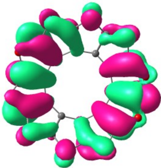
HOMO-2
