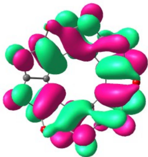
HOMO-2
