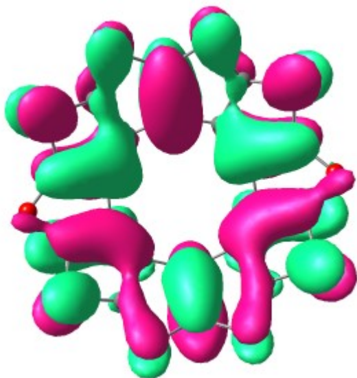
HOMO-2
