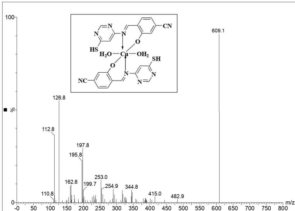
Figure 29S. Mass Spectrum of Cu Complex
