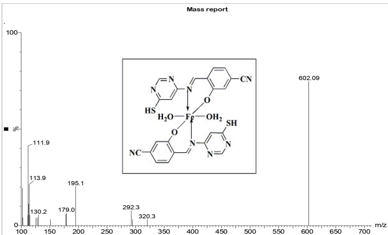
Figure 8S. Mass Spectrum of Fe complex
