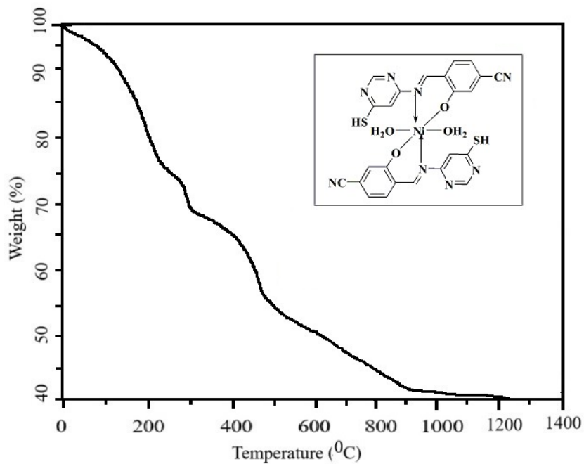
Figure 22S. TGA of Ni complex
