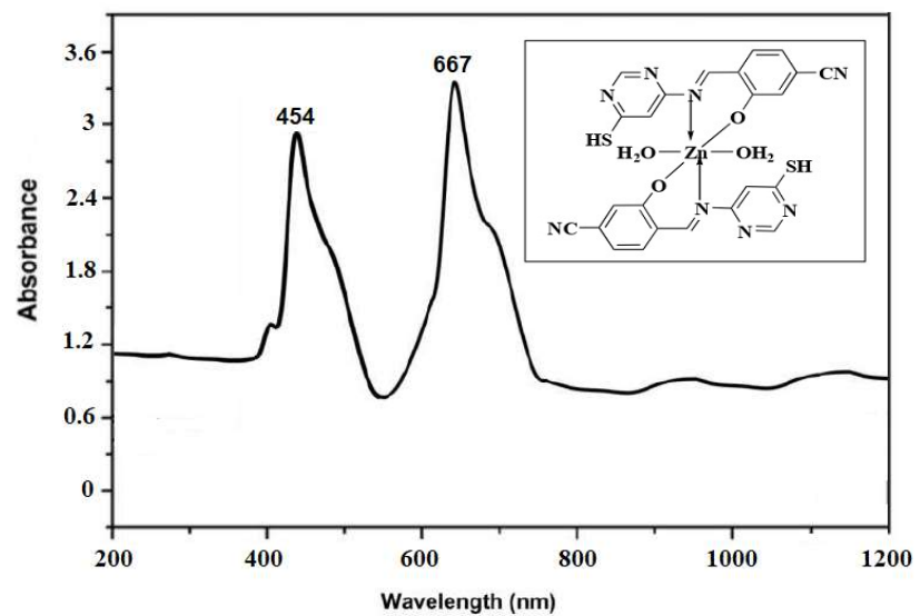
Figure 35S. UV visible Spectrum of Zn Complex
