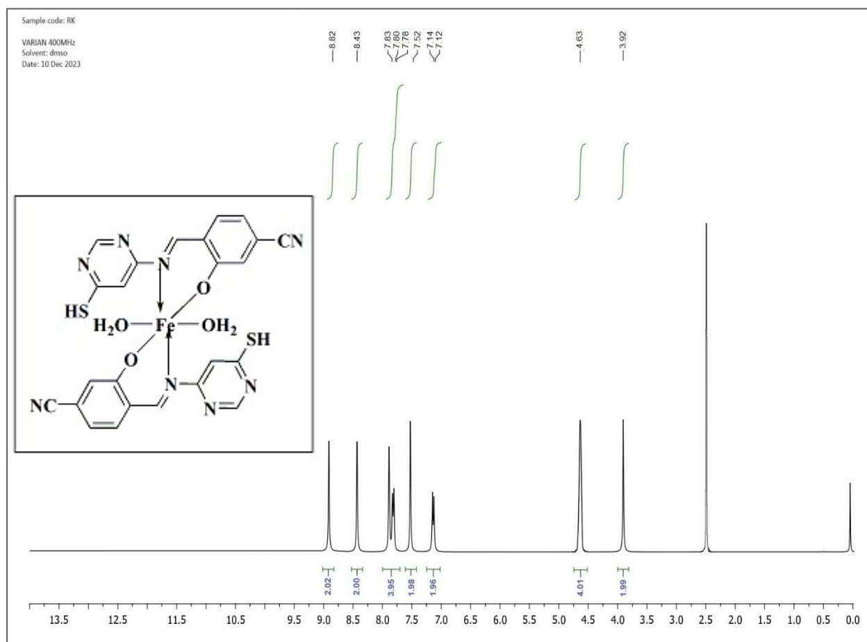
Figure 6S. 1 H NMR Spectrum of Fe complex
