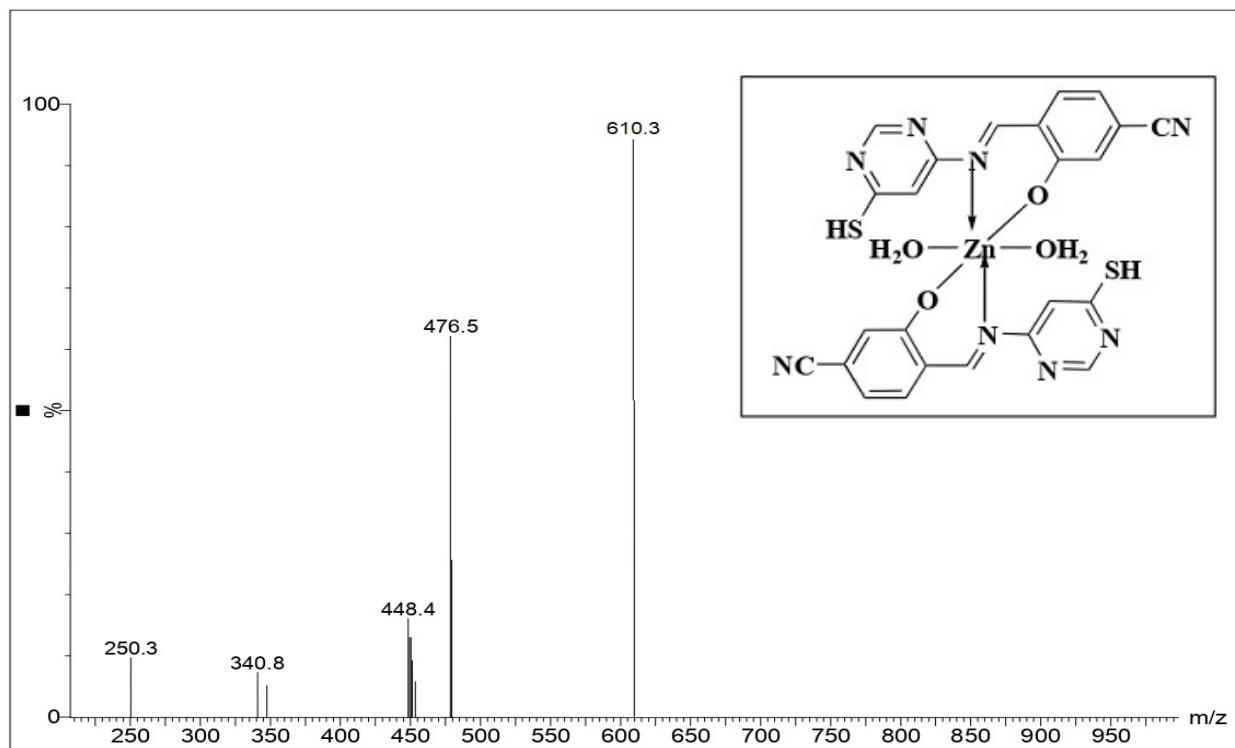
Figure 33S. Mass Spectrum of Zn Complex
