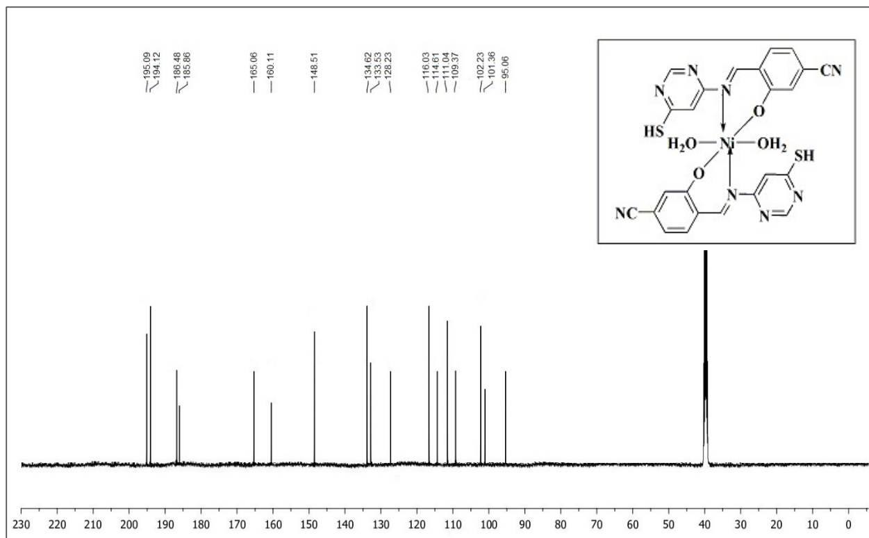
Figure 19S. ^{13}\text{C} NMR Spectrum of Ni complex
