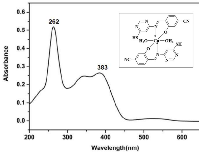
Figure 31S. UV visible Spectrum of Cu Complex
