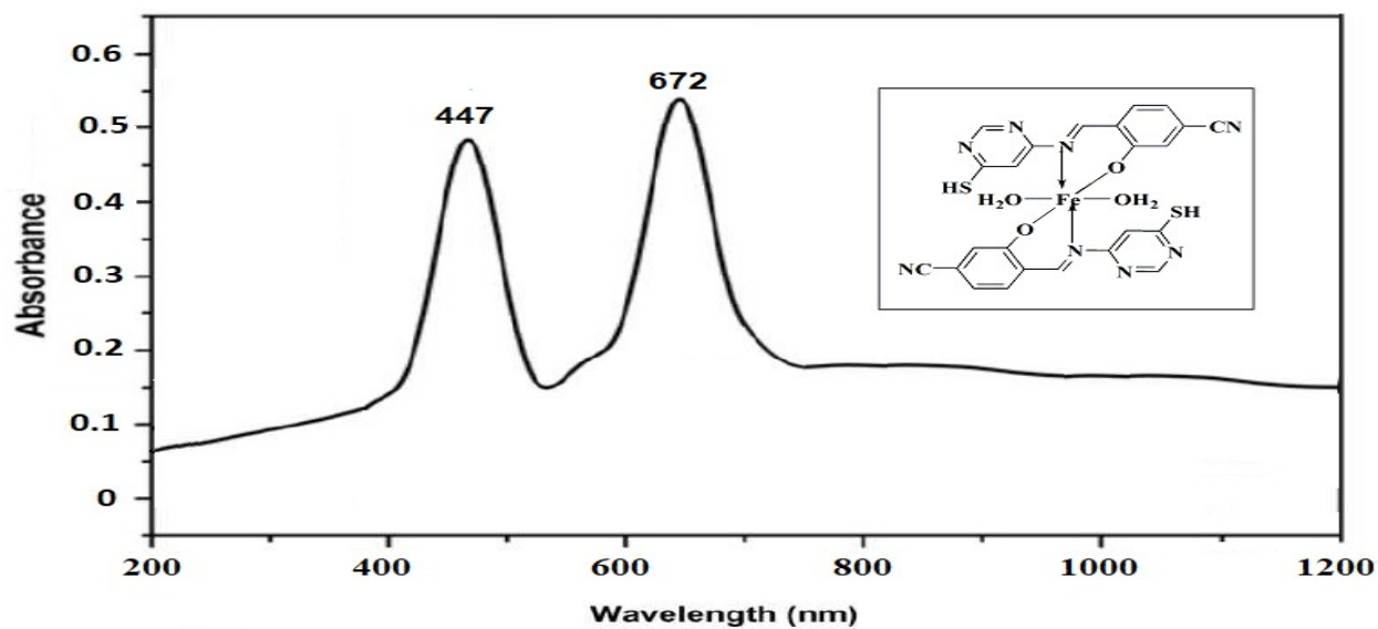
Figure 11S. UV Visible Spectrum of Fe complex
