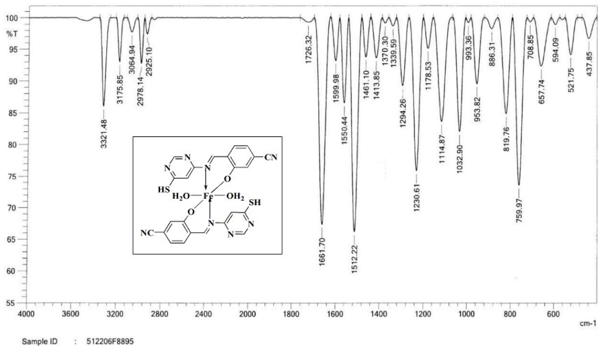
Figure 9S. IR Spectrum of Fe complex
