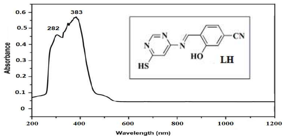
Figure 5S. UV Visible Spectrum of ligand (LH)
