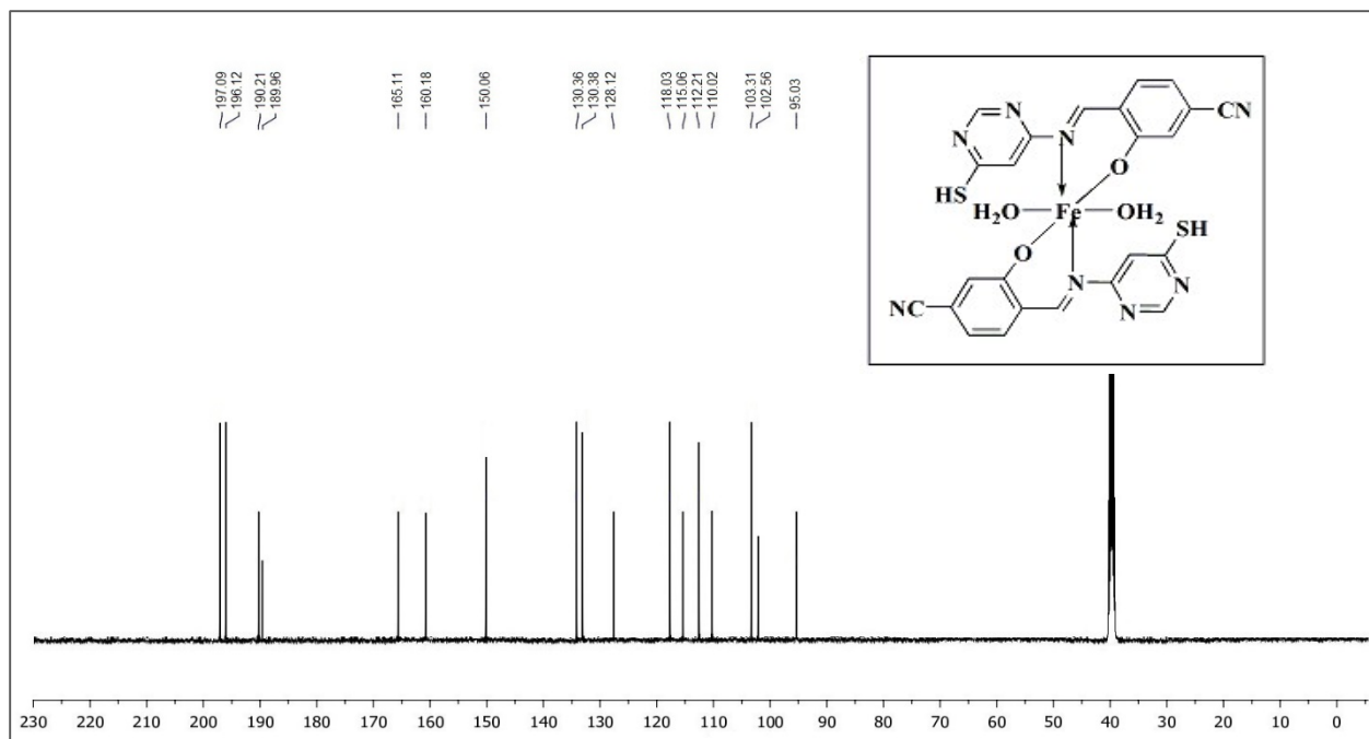
Figure 7S. ^{13}\text{C} NMR Spectrum of Fe complex
