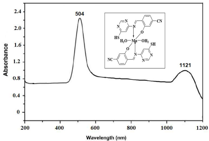
Figure 27S. UV visible Spectrum of Mn Complex
