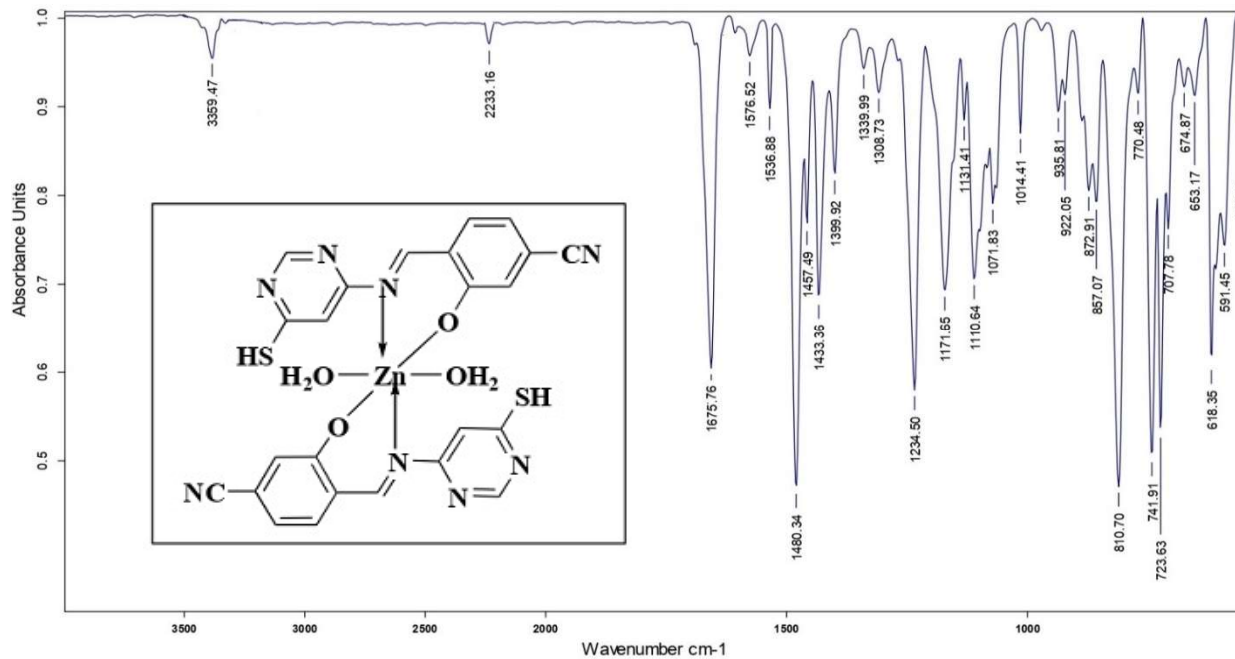
Figure 32S. IR Spectrum of Zn Complex
