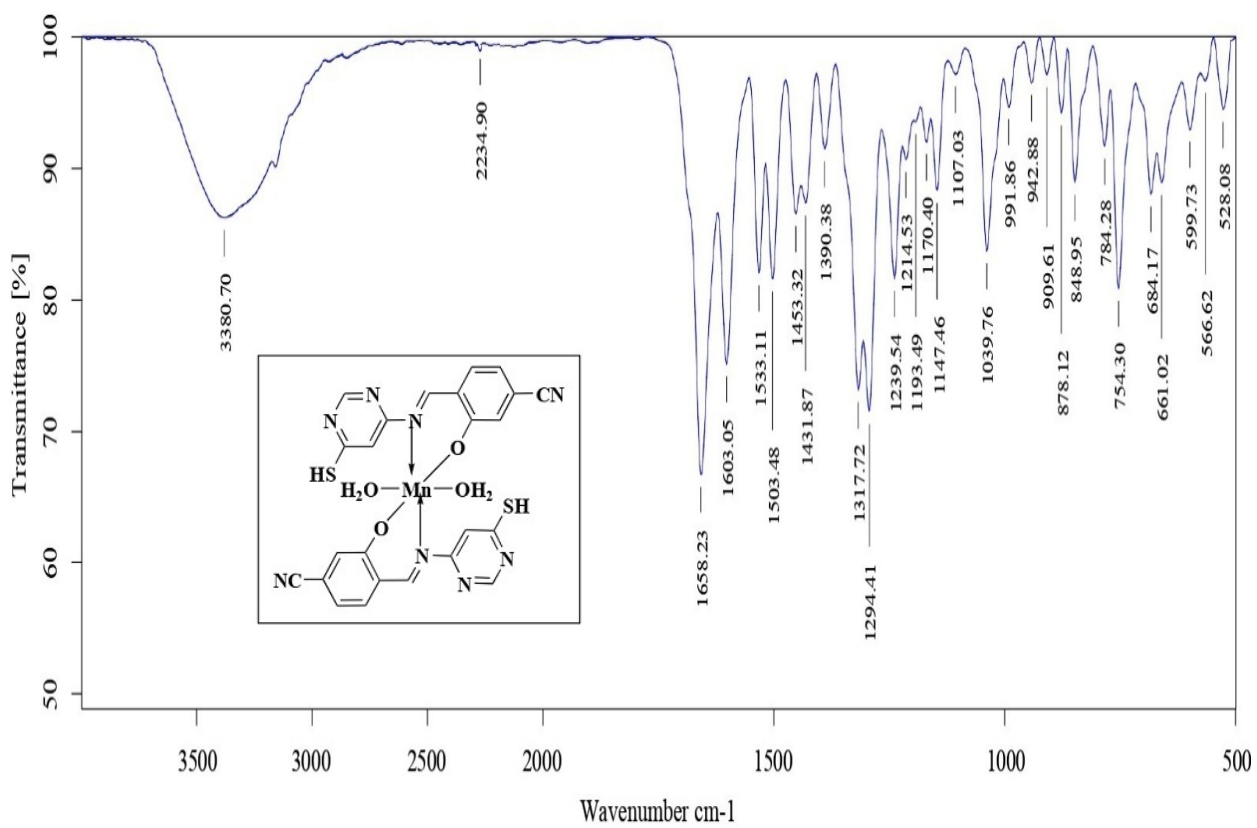
Figure 24S. IR Spectrum of Mn Complex
