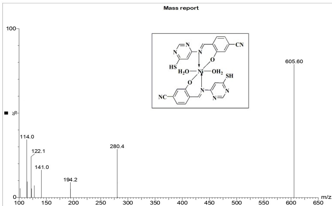
Figure 20S. Mass Spectrum of Ni complex
