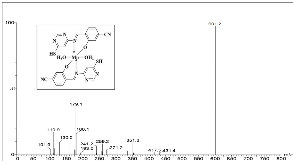
Figure 25S. Mass Spectrum of Mn Complex
