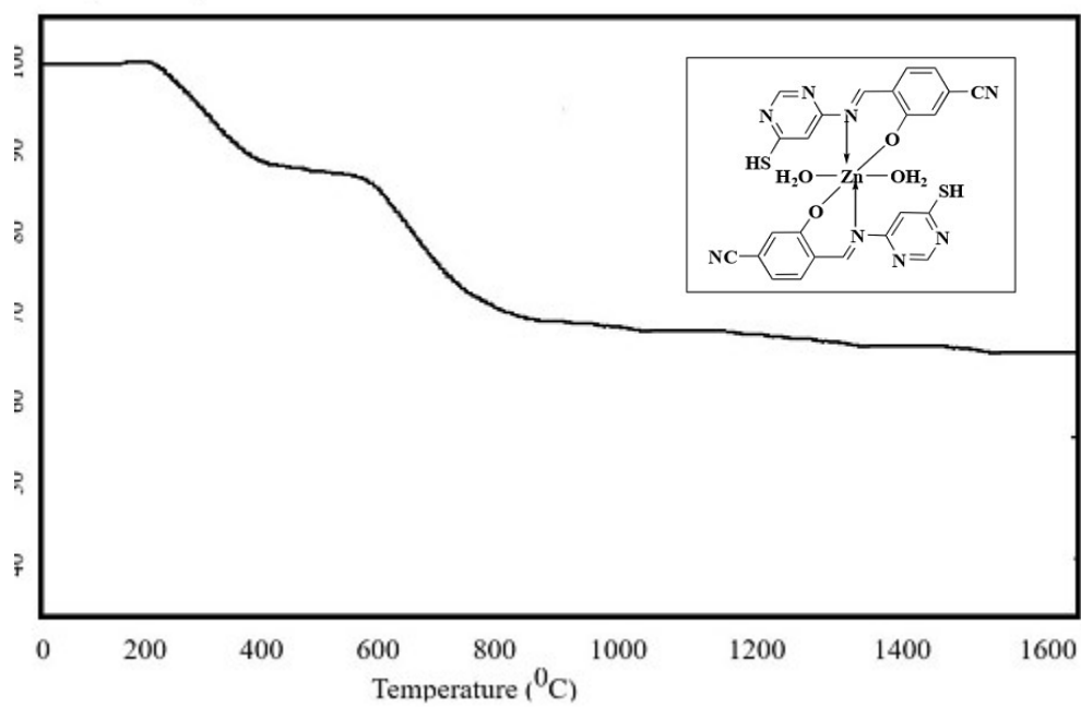
Figure 34S. TGA of Zn Complex
