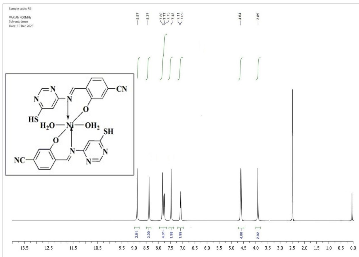
Figure 18S. 1 H NMR Spectrum of Ni complex
