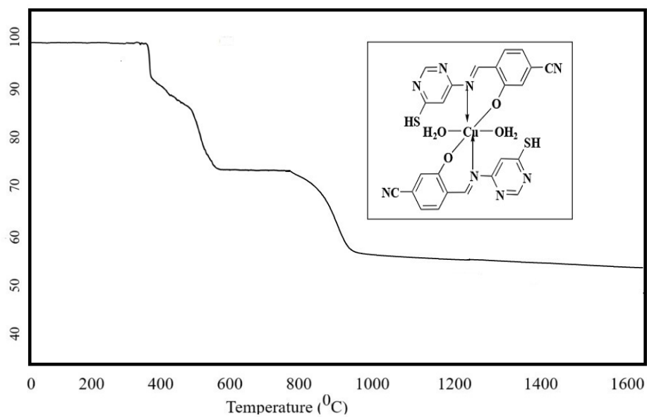
Figure 30S. TGA of Cu Complex
