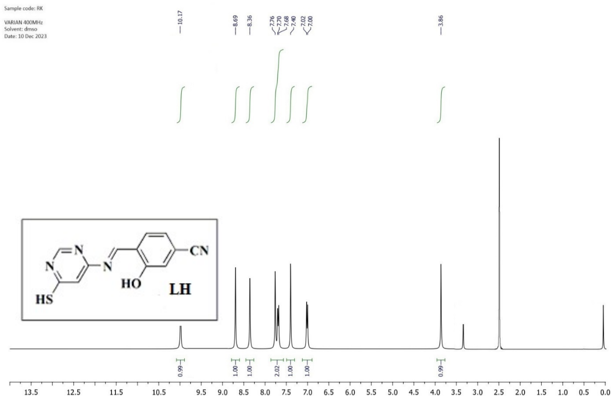
Figure 1S. ^1\text{H} NMR Spectrum of ligand (LH)
