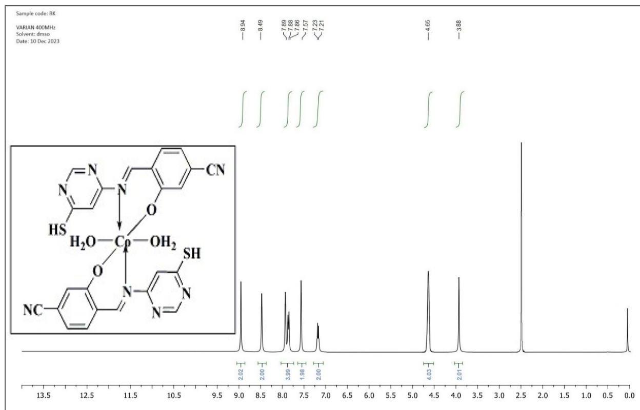
Figure 12S. 1 H NMR Spectrum of Co complex
