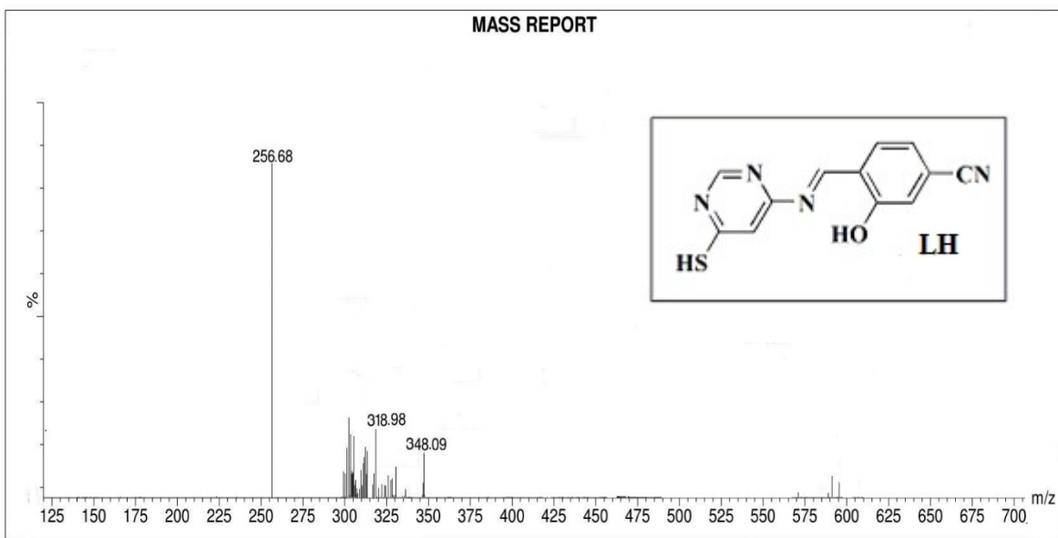
Figure 3S. Mass Spectrum of ligand (LH)
