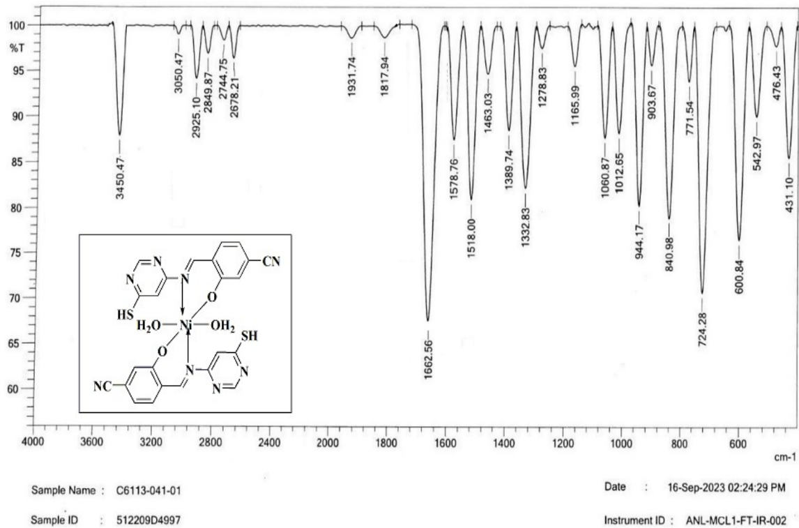
Figure 21S. IR Spectrum of Ni complex
