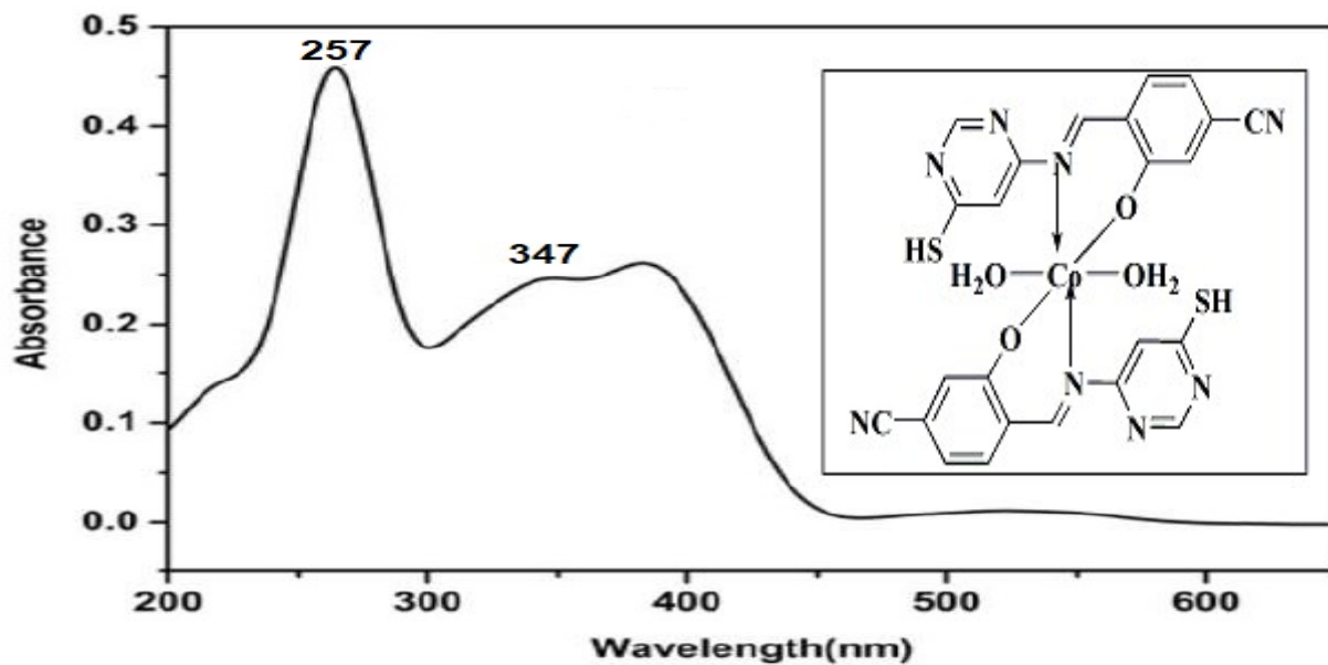
Figure 17S. UV Visible spectrum of Co complex
