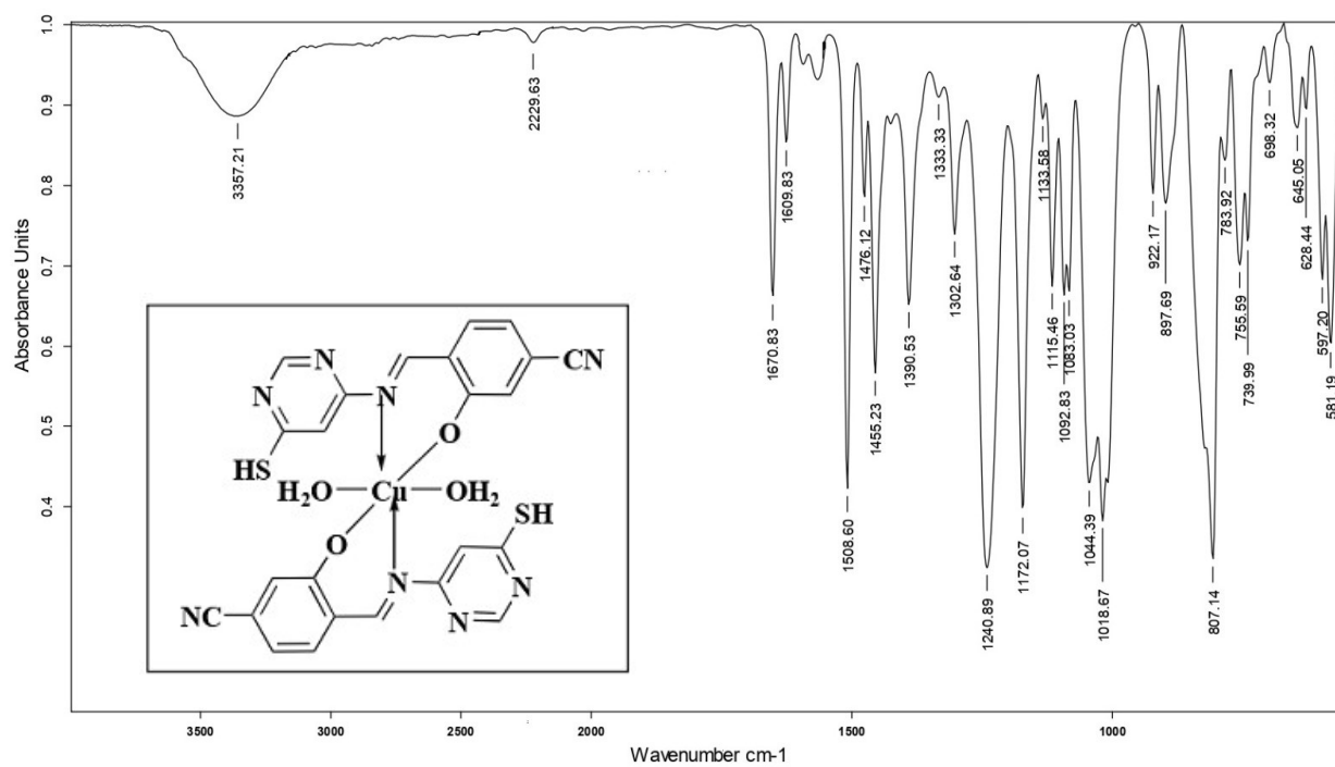
Figure 28S. IR Spectrum of Cu Complex
