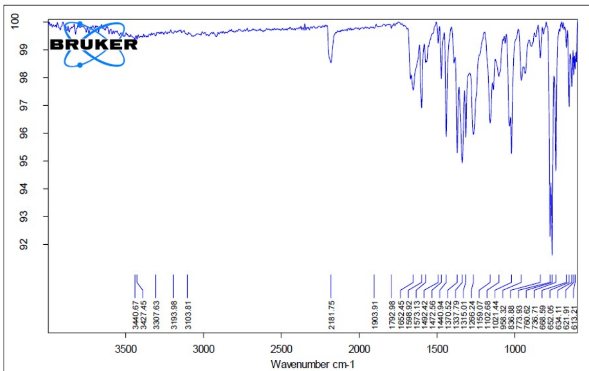
Figure S2. IR spectrum of Ni(o-phen) 2 (CED) complex (2)
