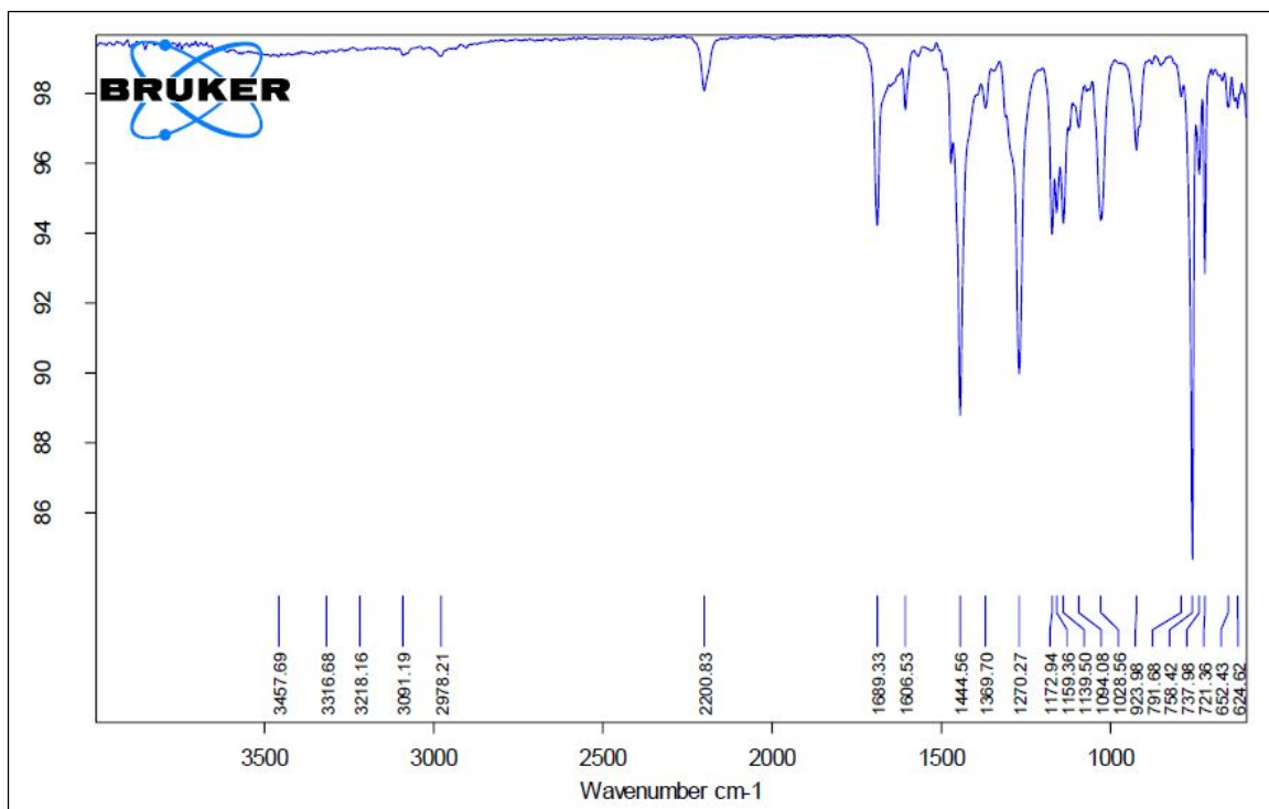
Figure S5. IR spectrum of Ni(bipy) 2 (CED) complex (5)
