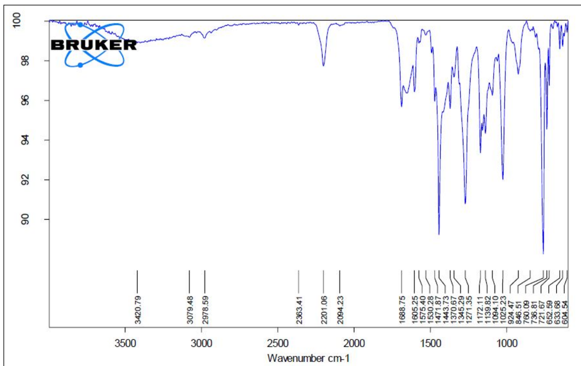
Figure S4. IR spectrum of Ni(bipy)(CED).4H 2 O complex (4)
