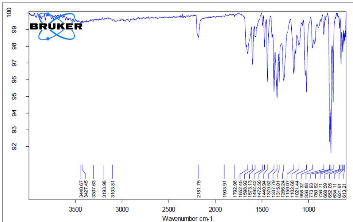
Figure S6. IR spectrum of Ni(bipy) 3 (CED) complex (6)
