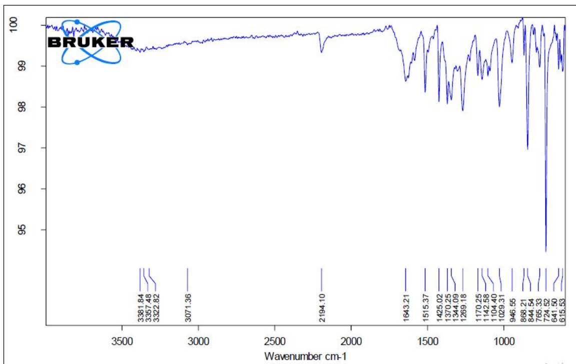
Figure S3. IR spectrum of Ni(o-phen) 3 (CED) complex (3)
