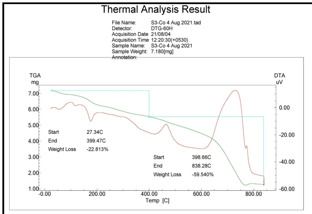
Fig. SI-18. TGA/DTA curves of Co(II) complex
