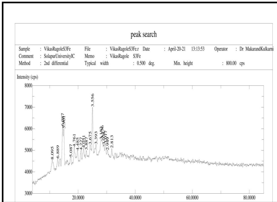
Fig. SI-22. Powder XRD of Fe(III) complex
