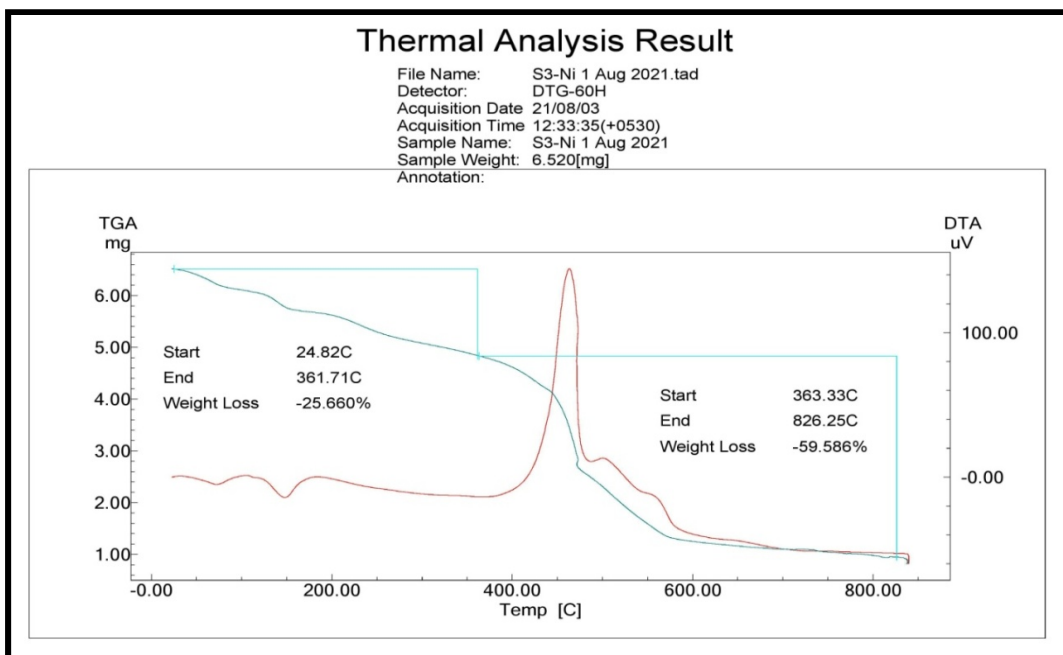
Fig. SI-19. TGA/DTA curves of Ni(II) complex
