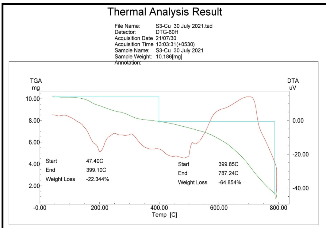
Fig. SI-20. TGA/DTA curves of Cu(II) complex
