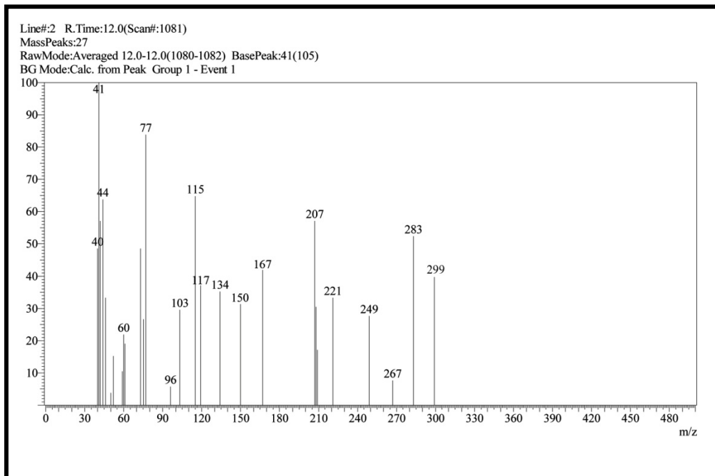
Fig. SI-15. Mass spectrum of Schiff base ligand ( S_3 )
