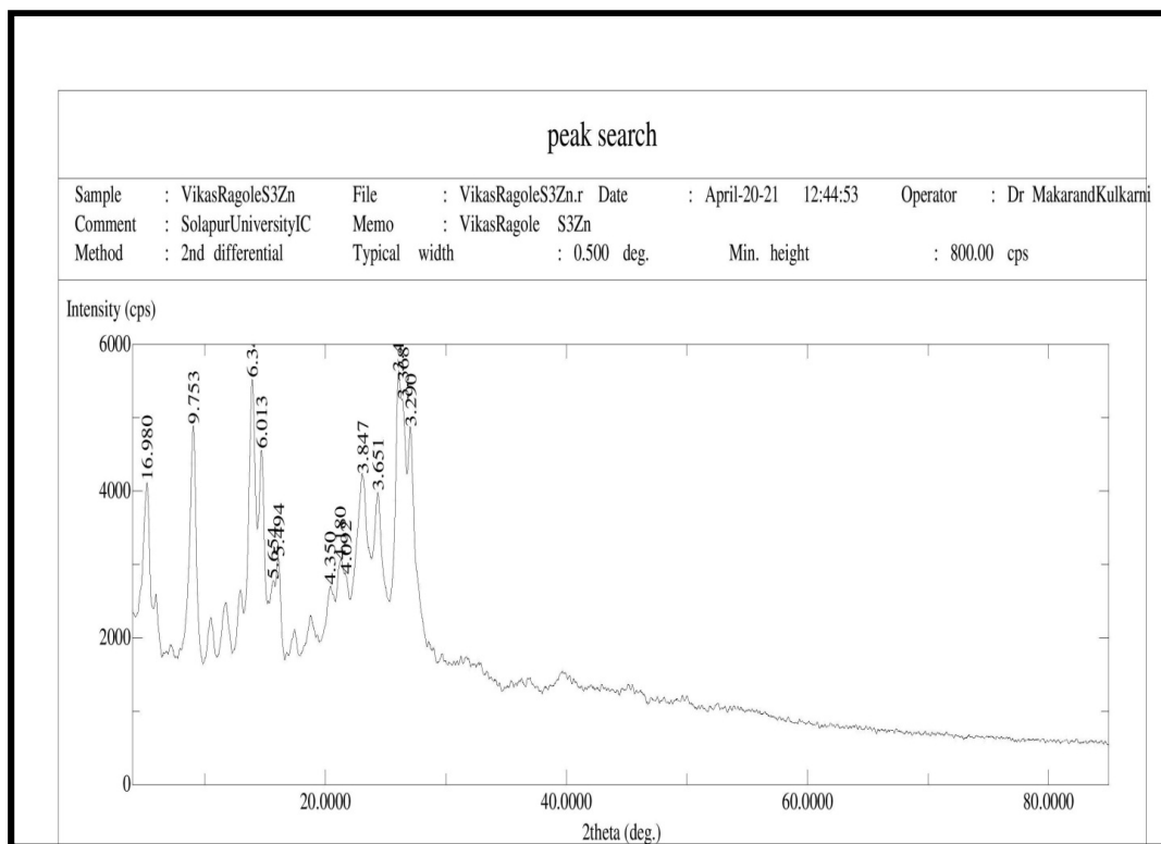
Fig. SI-26. Powder XRD of Zn(II) complex
