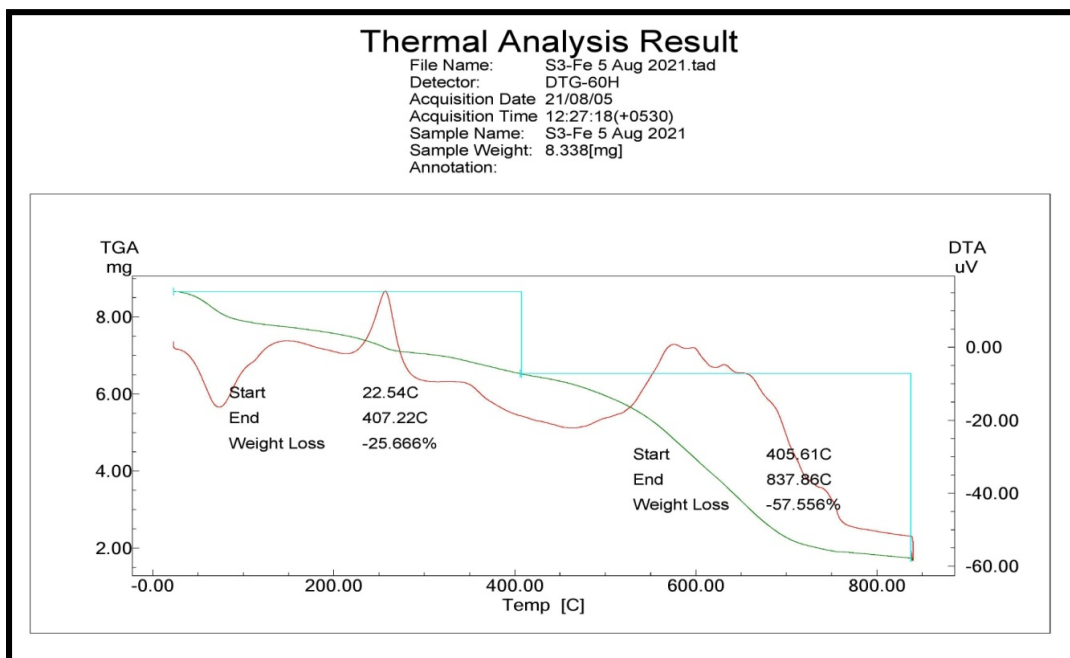
Fig. SI-17. TGA/DTA Curves of Fe(III)
