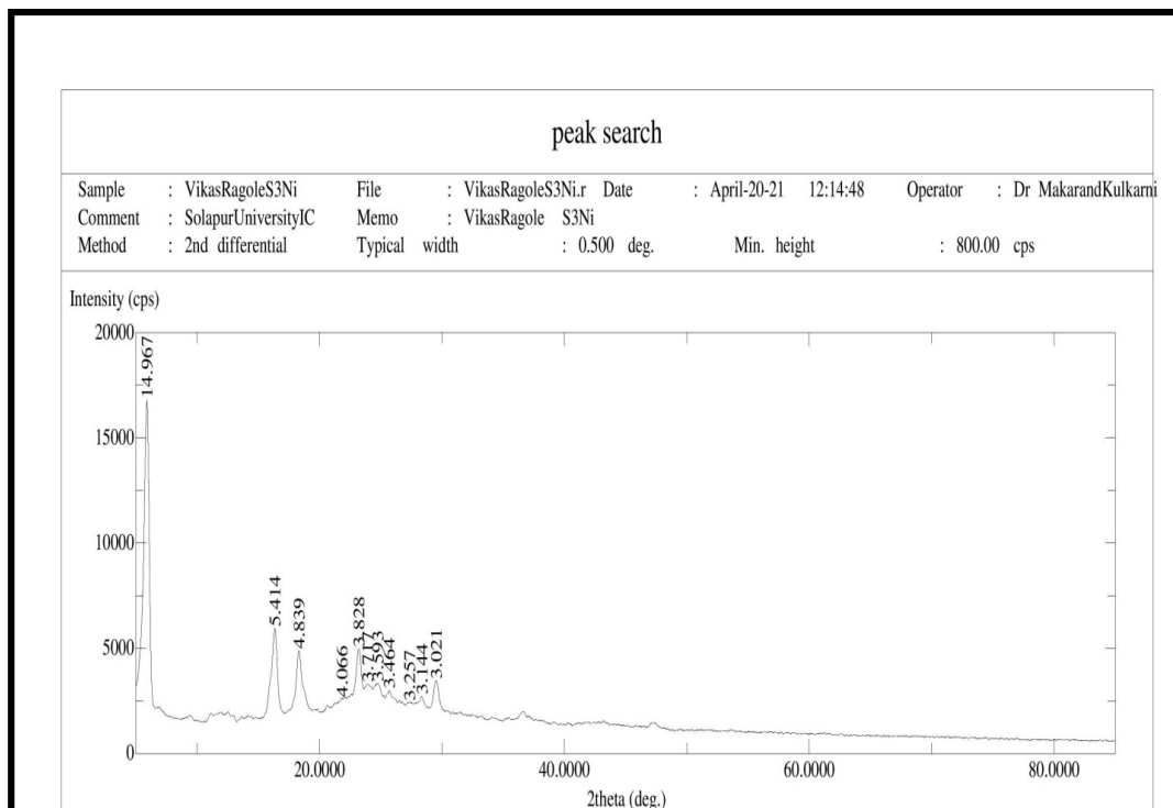
Fig. SI-24. Powder XRD of Ni(II) complex
