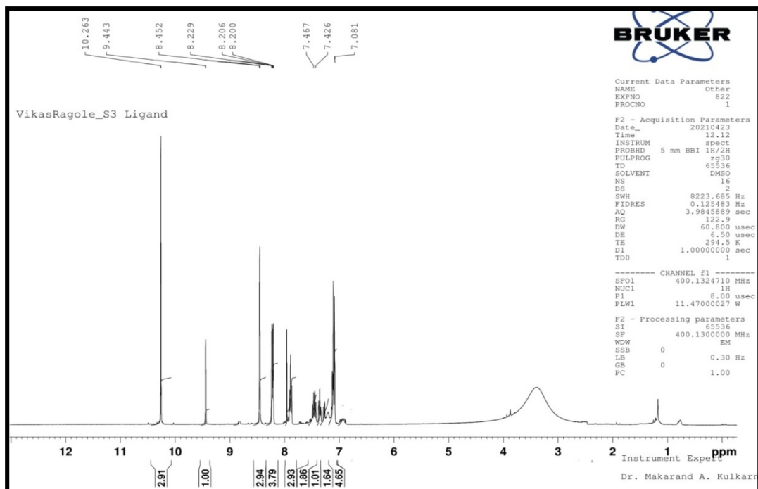
Fig. SI-13. ^1\text{H} NMR spectrum of Schiff base ligand ( \text{S}_3 )
