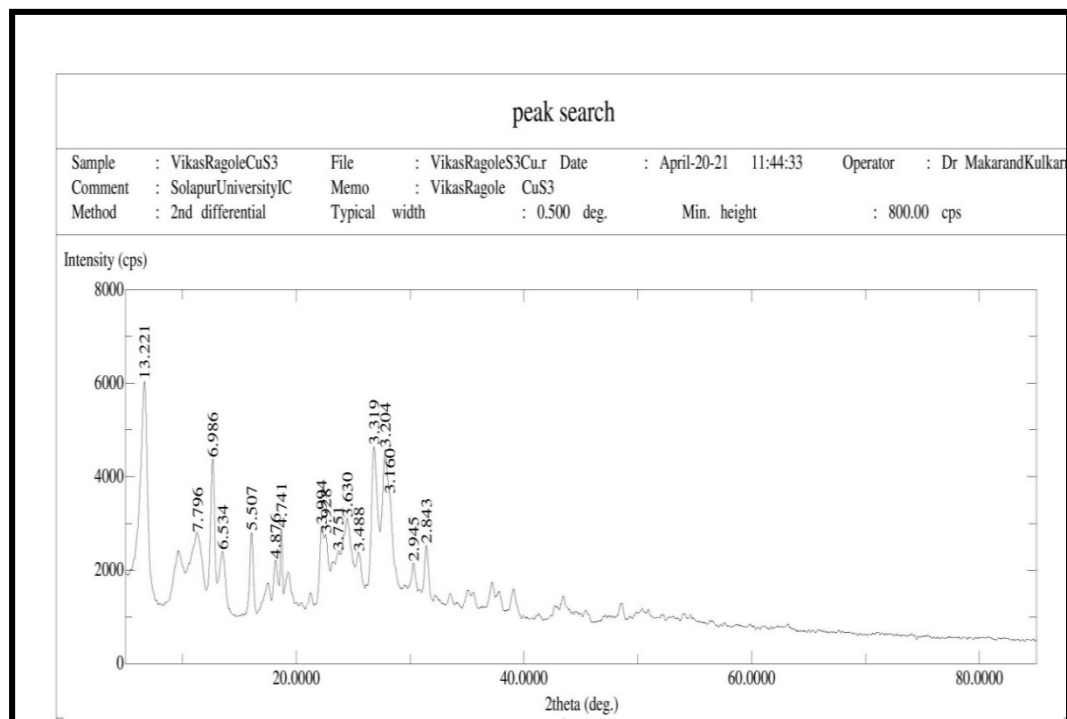
Fig. SI-25. Powder XRD of Cu(II) complex
