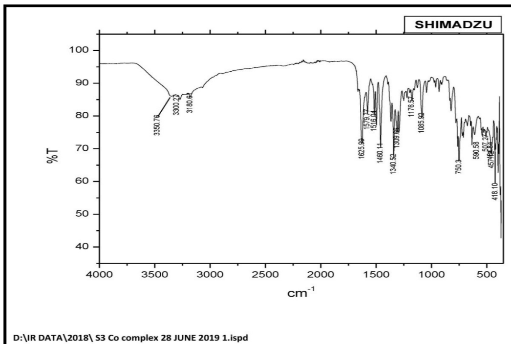
Fig. SI-3. IR spectrum of Co(II) Complex
