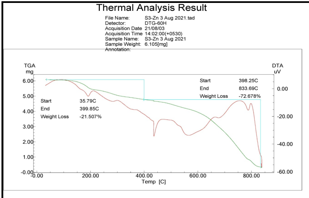
Fig. SI-21. TGA/DTA curves of Zn(II) complex
