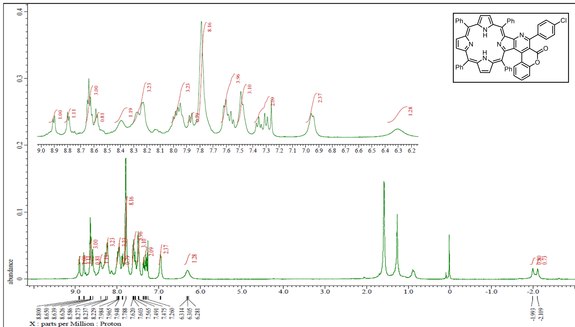
Figure S4. ^1\text{H} NMR spectrum of porphyrin (9) in \text{CDCl}_3
