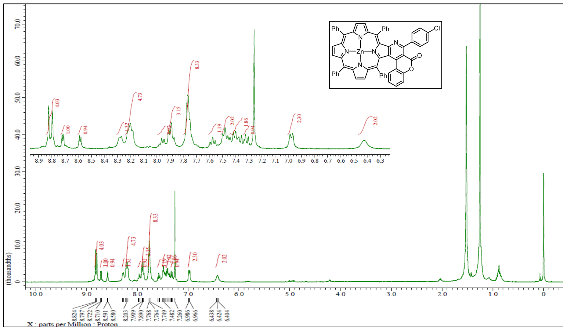
Figure S9. ^1\text{H} NMR spectrum of porphyrin ( 13 ) in \text{CDCl}_3
