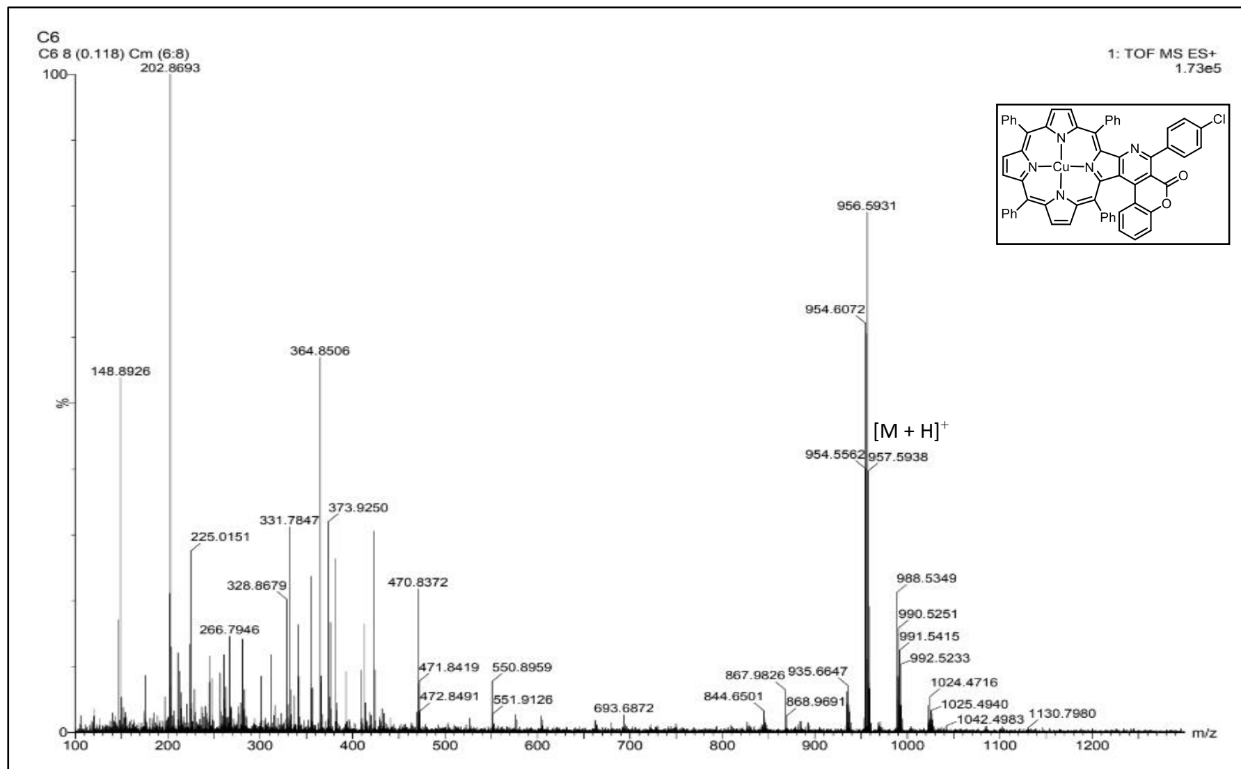
Figure S13. ESI mass spectrum of copper(II) porphyrin (4)
