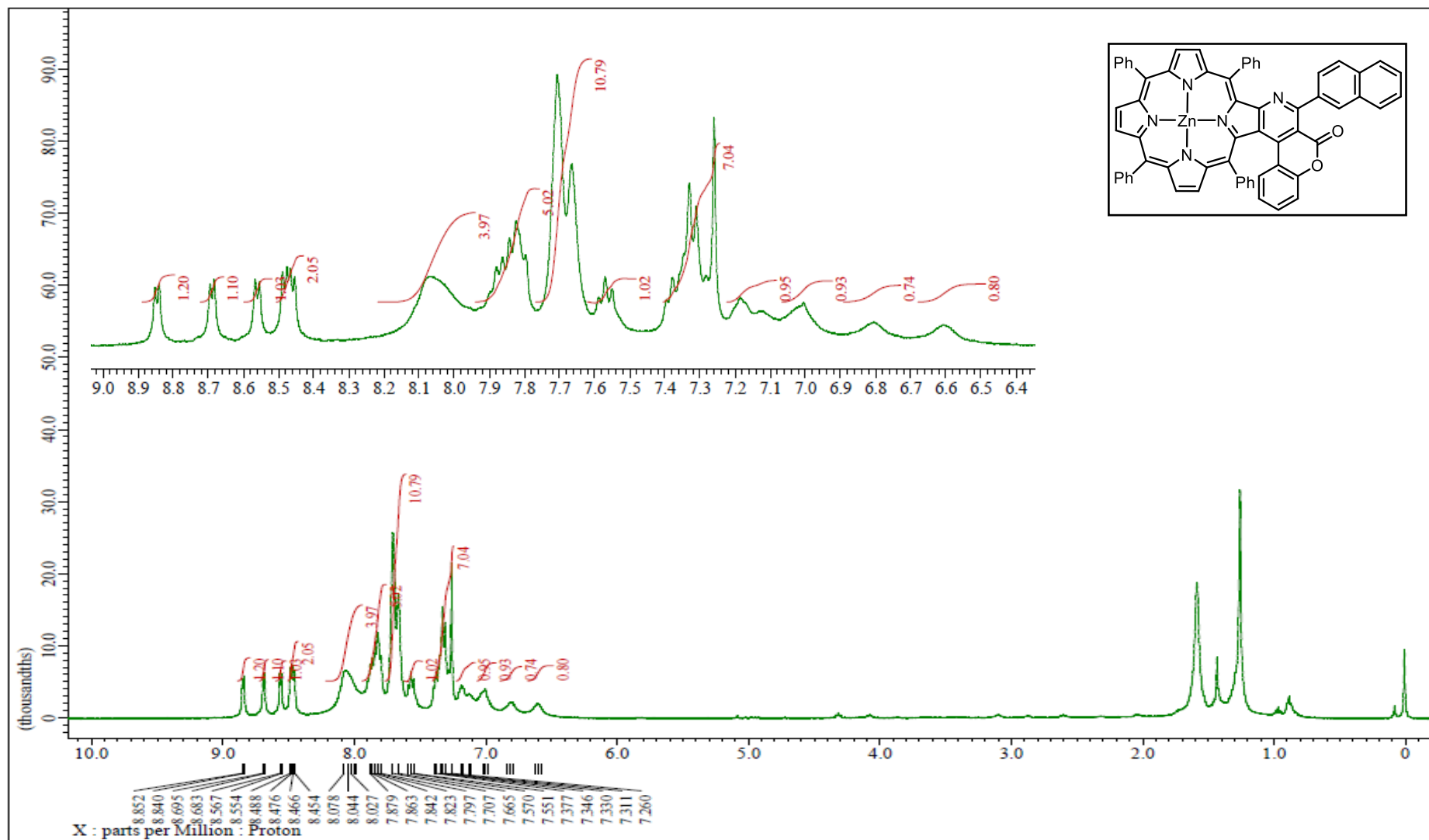
Figure S11. ^1\text{H} NMR spectrum of porphyrin (15) in \text{CDCl}_3
