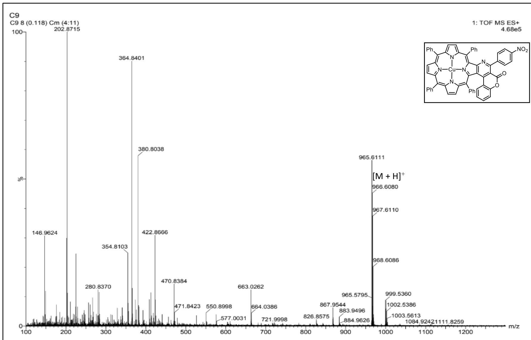
Figure S14. ESI mass spectrum of copper(II) porphyrin ( 5 )
