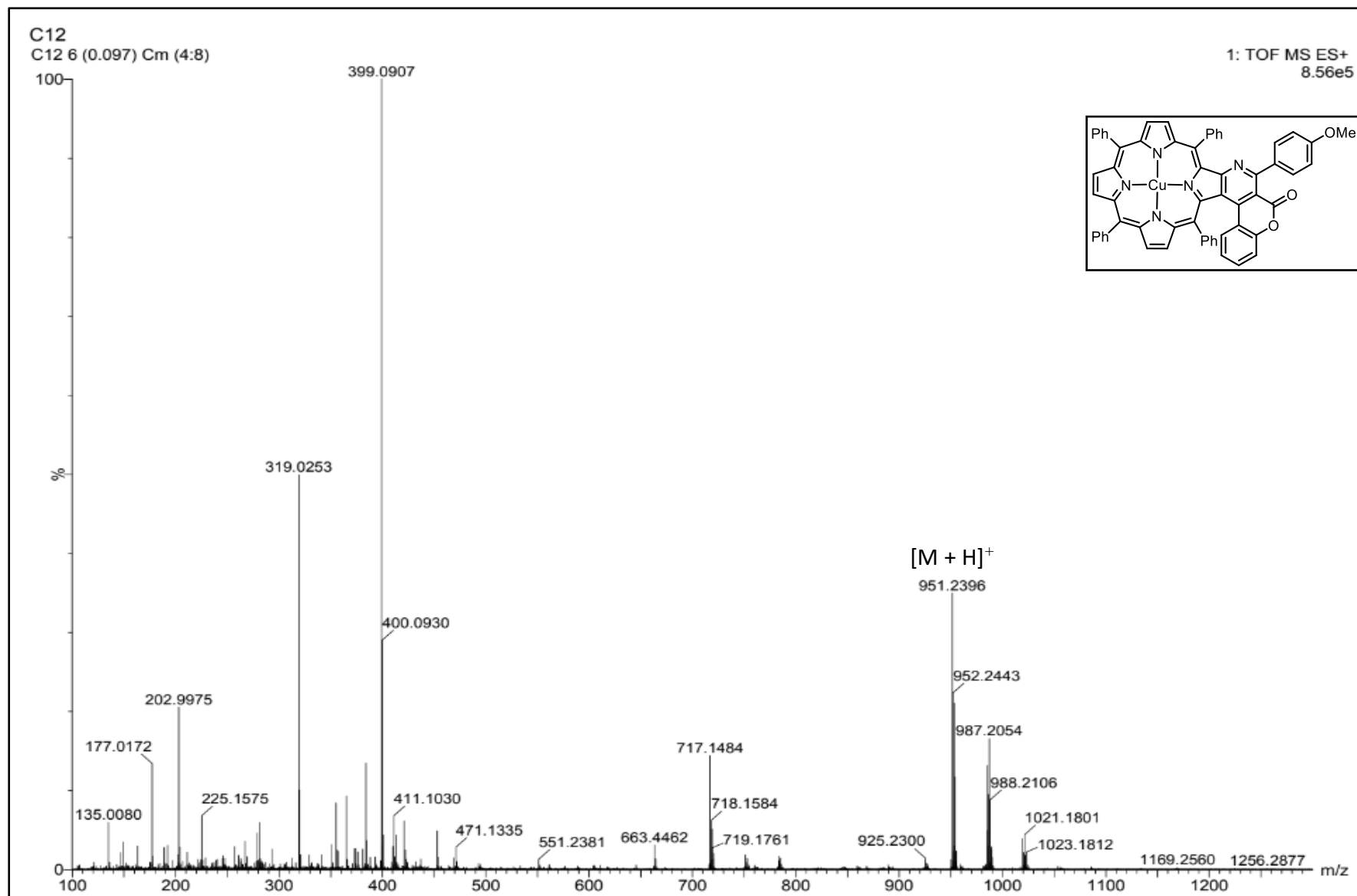
Figure S15. ESI mass spectrum of copper(II) porphyrin (6)
