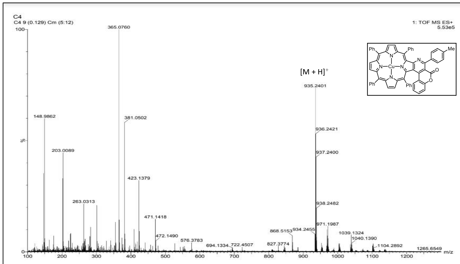
Figure S12. ESI mass spectrum of copper(II) porphyrin (3)
