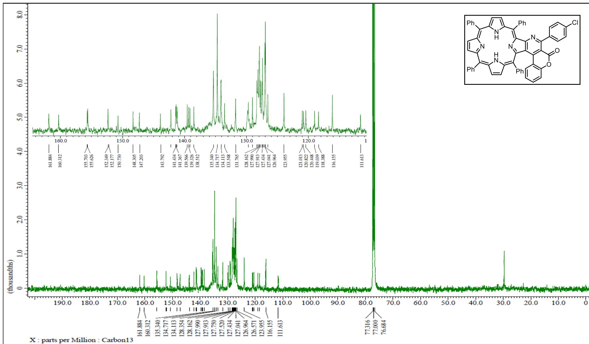
Figure S5. ^{13}\text{C} NMR spectrum of porphyrin (9) in \text{CDCl}_3
