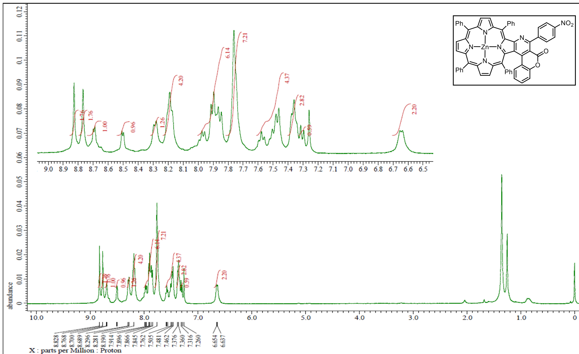
Figure S10. 1 H NMR spectrum of porphyrin ( 14 ) in CDCl 3
