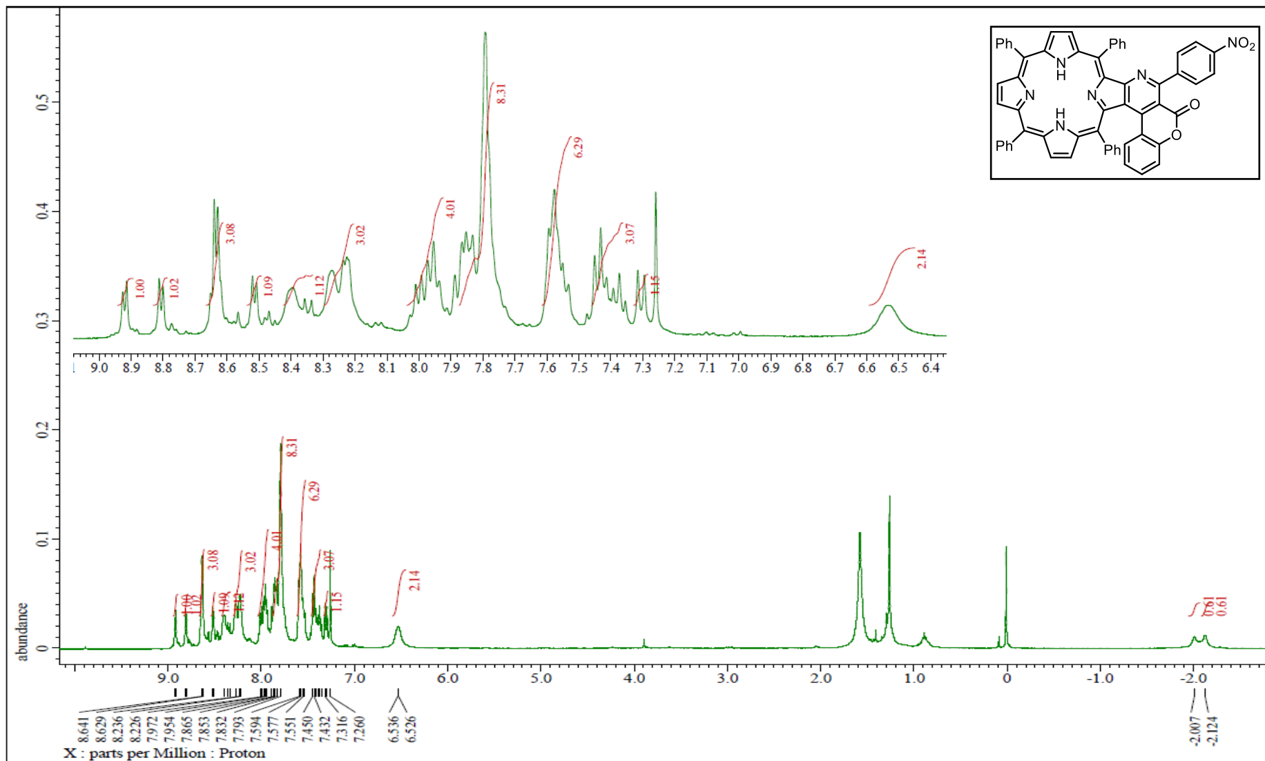
Figure S6. ^1\text{H} NMR spectrum of porphyrin (10) in \text{CDCl}_3
