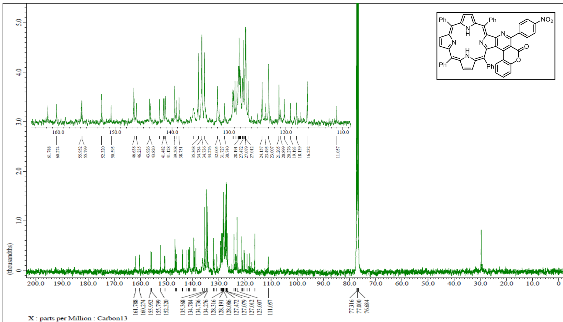
Figure S7. 13 C NMR spectrum of porphyrin ( 10 ) in CDCl 3
