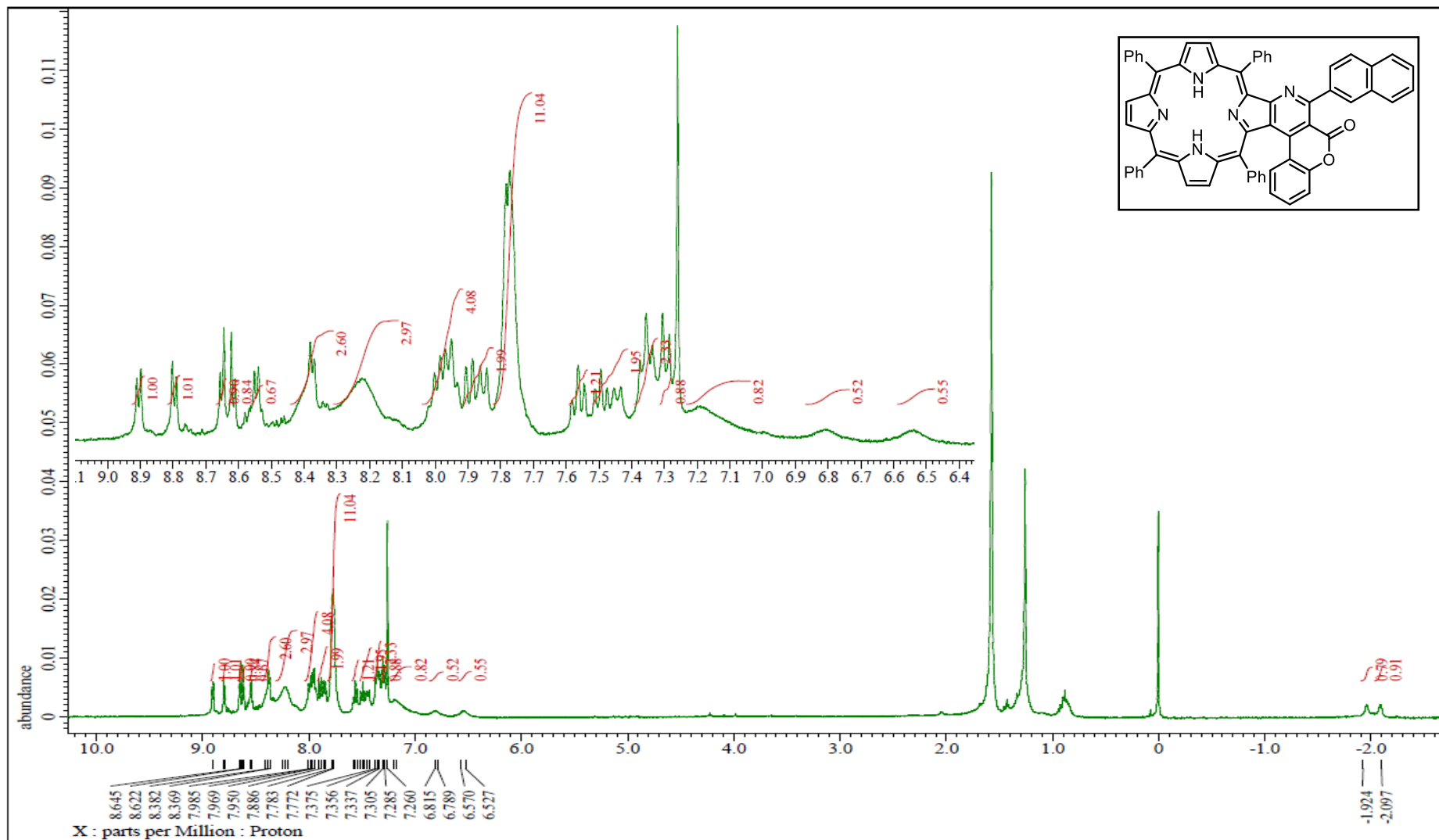
Figure S8. ^1\text{H} NMR spectrum of porphyrin ( 12 ) in \text{CDCl}_3
