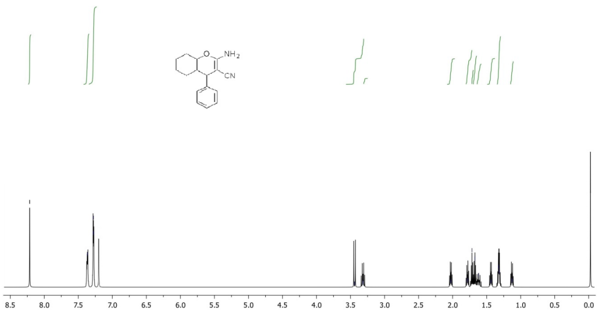
Fig. S5 — 1 H NMR spectrum of compound 2a
