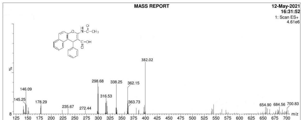
Fig. S9 — Mass spectrum of 3-acetamido-1-phenyl-1H-benzo[f]chromene-2carboxylic acid (compound 4)
