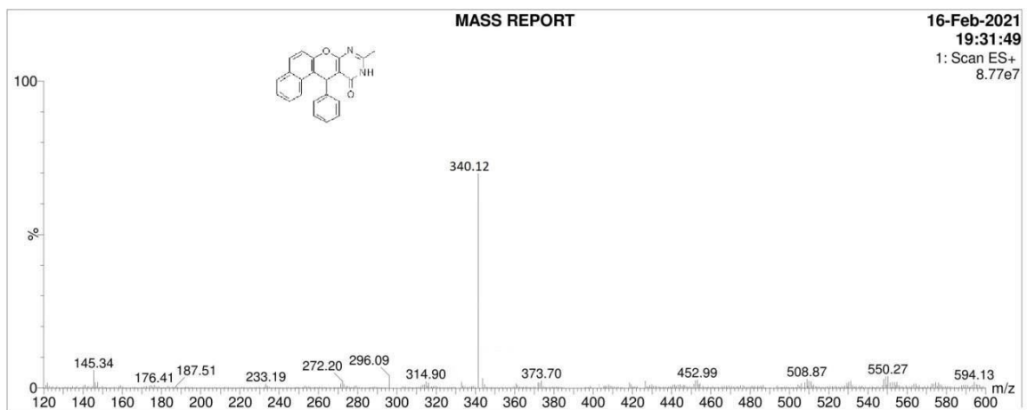
Fig. S6 — Mass spectra of 9 - methyl - 12- phenyl - 10H- benzo [5,6] chromeno [2,3,d] pyrimidine -11 (12H) one (3b)
