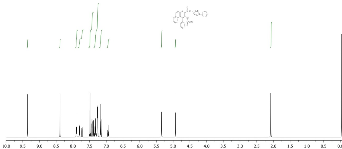
Fig. S3 — 1 H NMR spectrum of compound 6a
