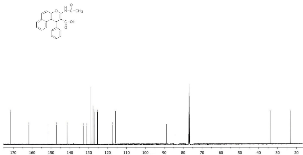
Fig. S10 — ^{13}\text{C} NMR spectrum of compound 4
