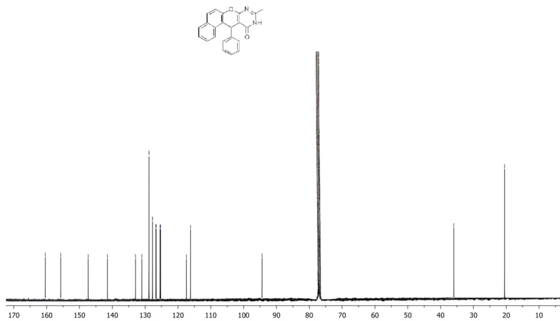
Fig. S7 — ^{13}\text{C} NMR spectrum of compound 3b
