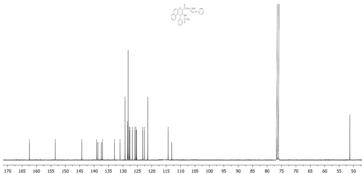
Fig. S4 — 13 C NMR spectrum of compound 6a
