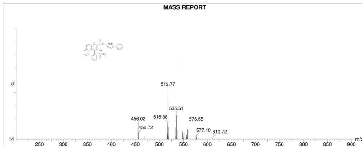
Fig. S1 — Mass spectrum of compound (1-phenyl-1H-1,2,3-triazolo-4-yl) methyl 2-acetamido-1-phenyl-1H-benzo[f]chromene-3-carboxylate ( 6a )
