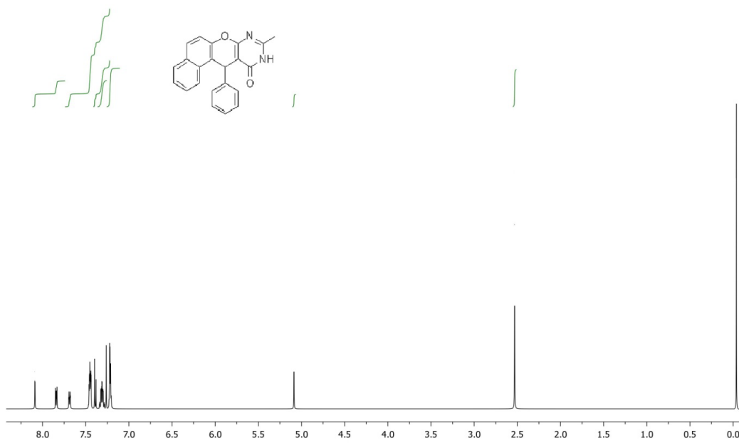
Fig. S8 — ^1\text{H} NMR spectrum of compound 3b
