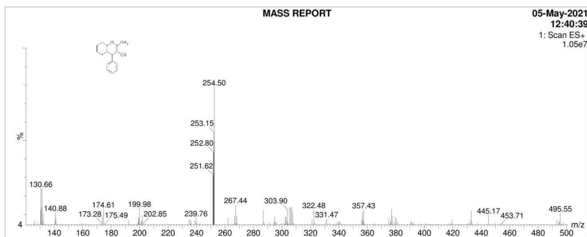
Fig. S2 — Mass spectra of 2-amino-4-phenyl-4a,5,6,7,8a-hexahydro-4H-chromene-3-carbonitrile ( 2a )
