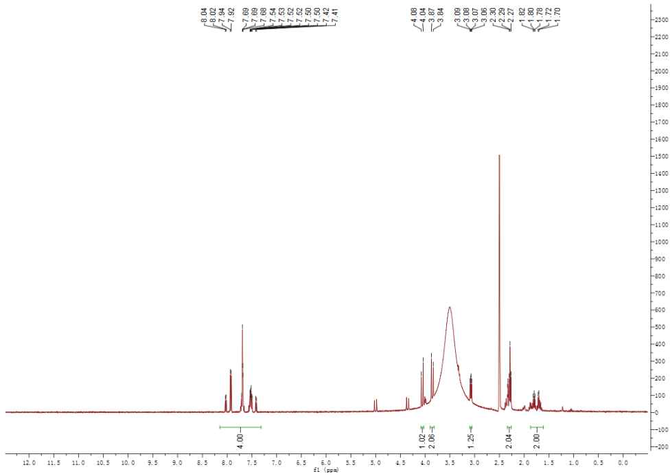
Fig. S2 — ^1\text{H} NMR spectrum of glutamic acid
