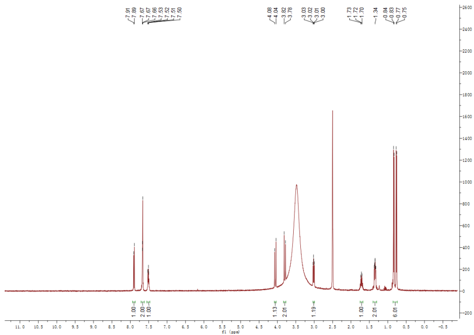
Fig. S3 — 1 H NMR spectrum of leucine
