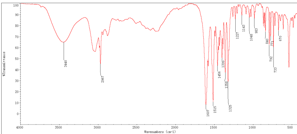
Fig. S8 — FTIR spectrum of valine
