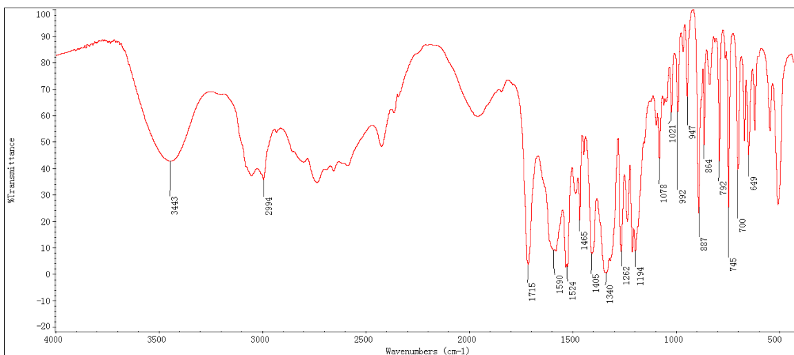
Fig. S5 — FTIR spectrum of aspartic acid
