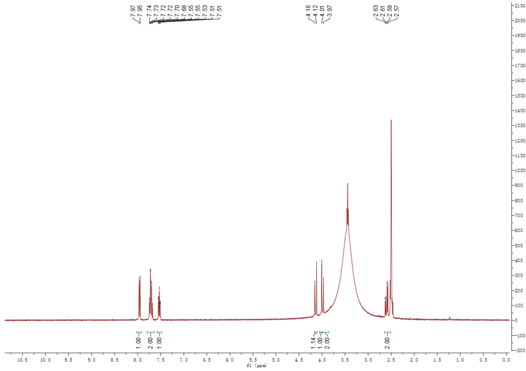
Fig. S1 — ^1\text{H} NMR spectrum of aspartic acid
