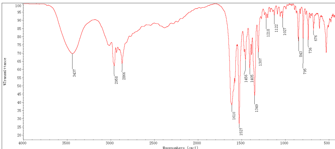
Fig. S7 — FTIR spectrum of leucine
