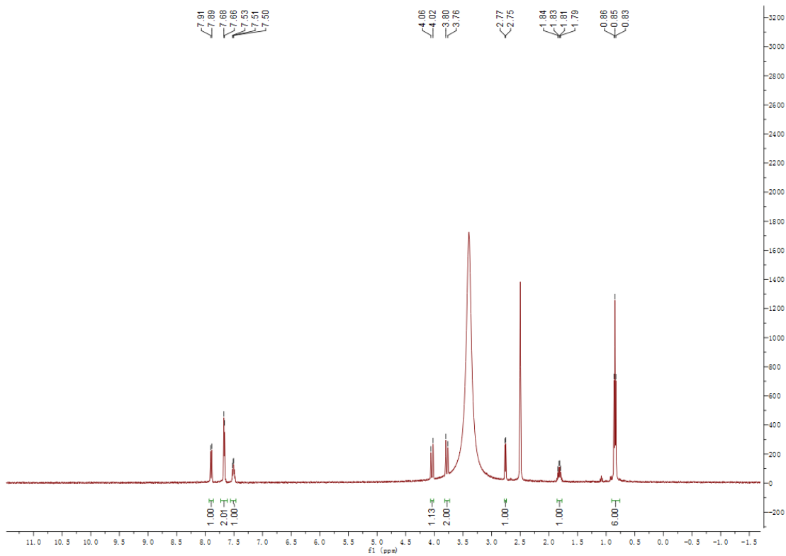
Fig. S4 — 1 H NMR spectrum of valine
