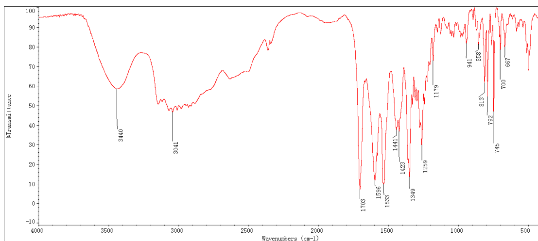
Fig. S6 — FTIR spectrum of glutamic acid
