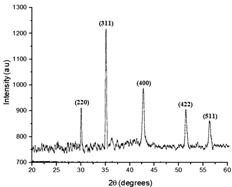
Fig. 7 — XRD pattern of ZnFe 2 O 4 NPs
