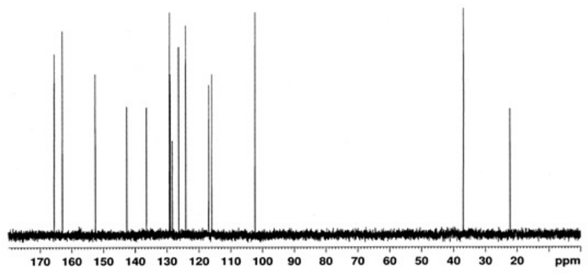
Fig.S 2. ^{13}\text{C} NMR Spectra of \text{L}^5
