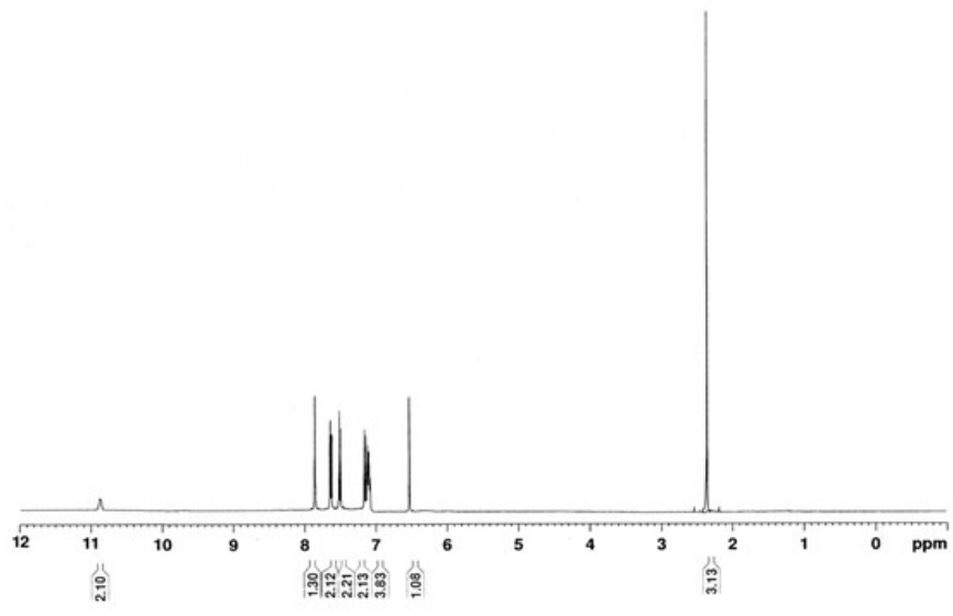
Fig.S 1. ^1\text{H} NMR Spectra of \text{L}^5
