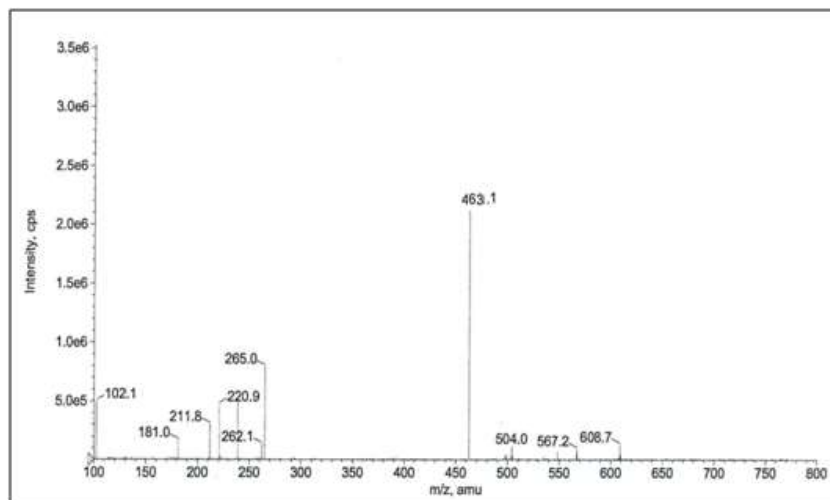
Fig.S 4. Mass Spectra of L 5
