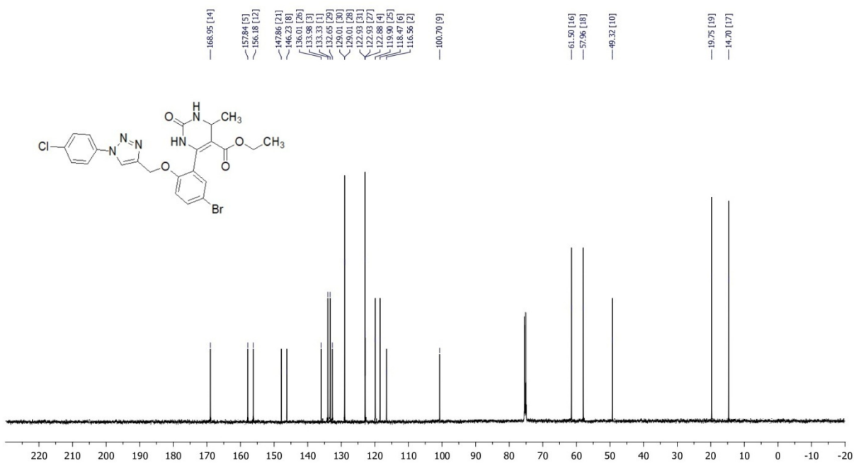
Figure S6 13 C NMR spectra of compound 4a
