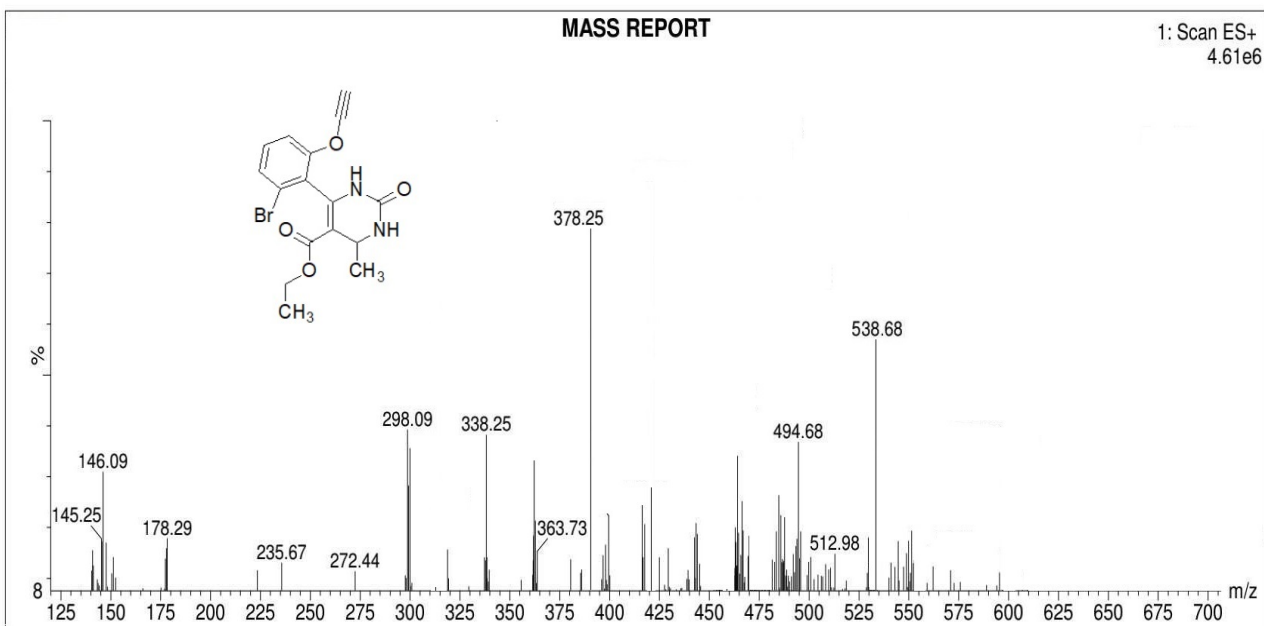
Figure S1 Mass spectra of compound 3(R=O)
