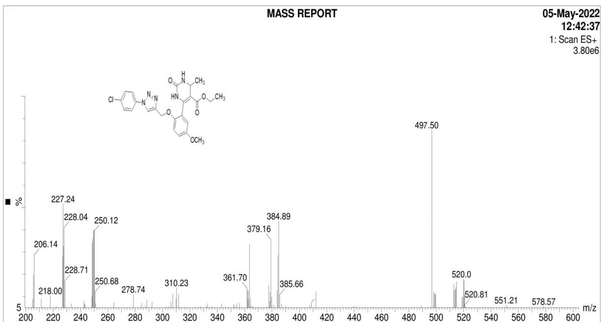
Figure S7 Mass spectra of compound 4d
