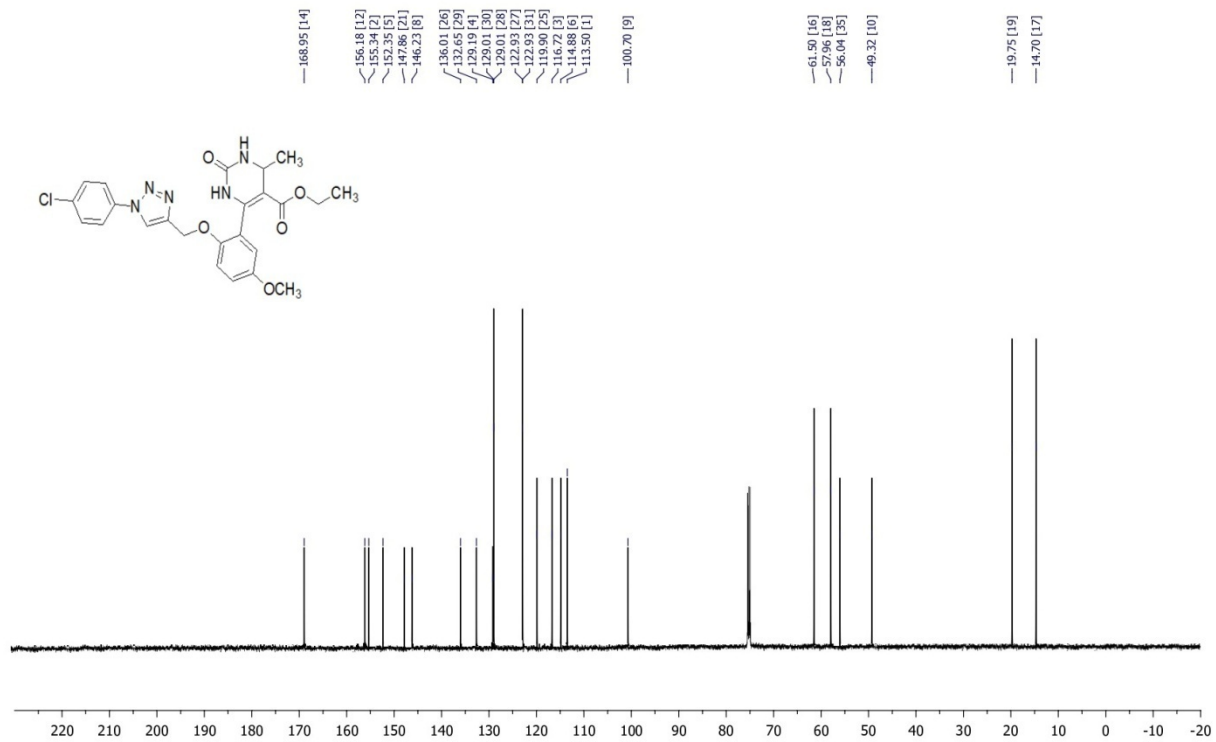
Figure S9 ^{13}\text{C} NMR spectra of compound 4d
