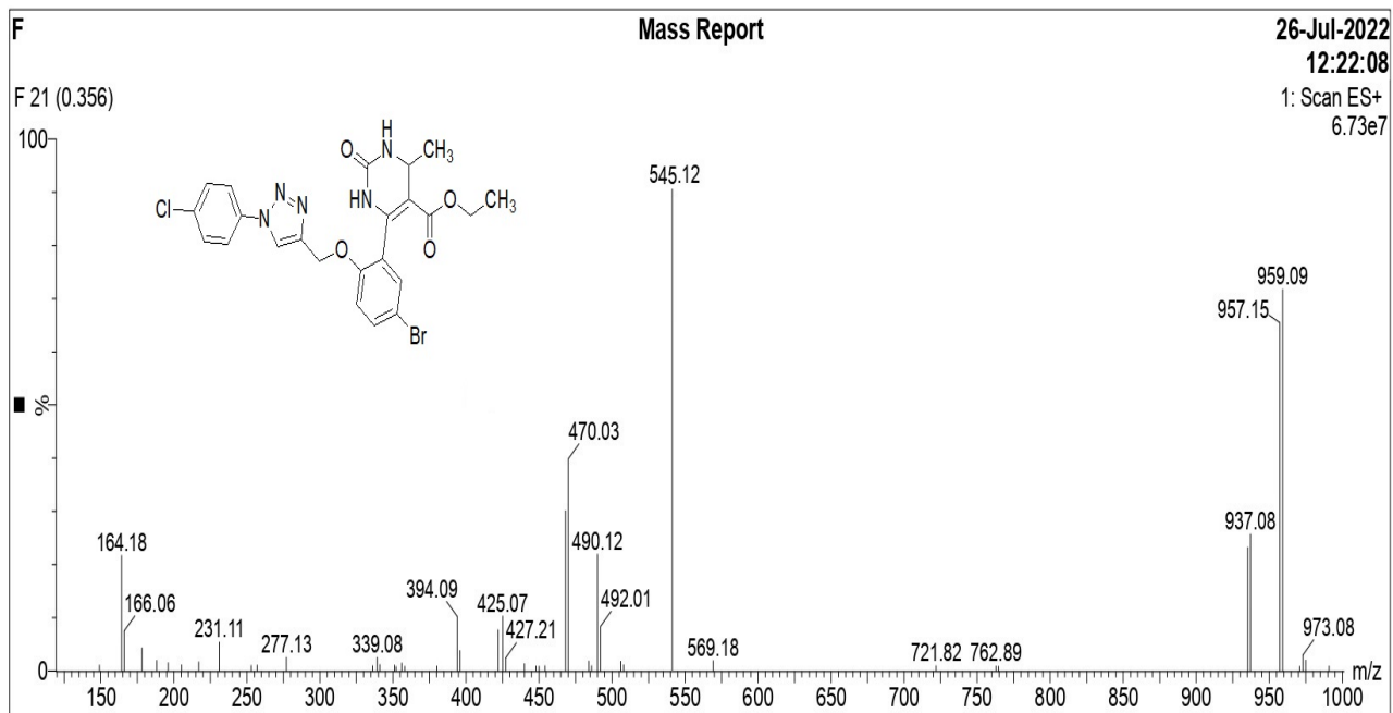
Figure S4 Mass spectra of compound 4a
