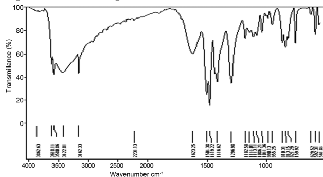
Fig. 1 — IR Spectrum of Complex (1)
