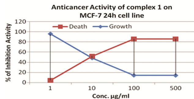
Fig. 6 — Complex displayed good cytotoxicity of IC_{50} 9.13\text{ }\mu\text{g/mL}
