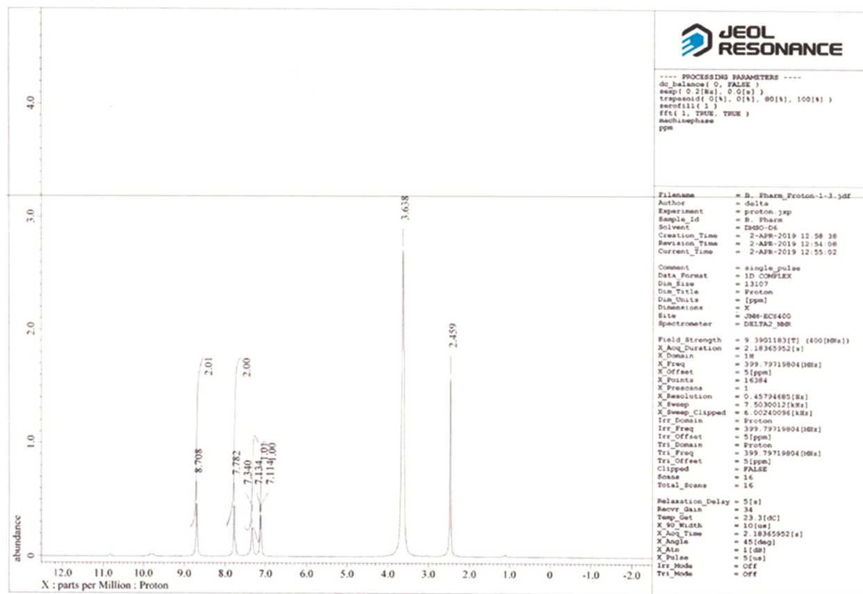
Fig. 6 — NMR spectral data for the title compounds -N-(4-fluoro phenyl)-2-isonicotonyl hydrazine carbothioamide 3(c)
