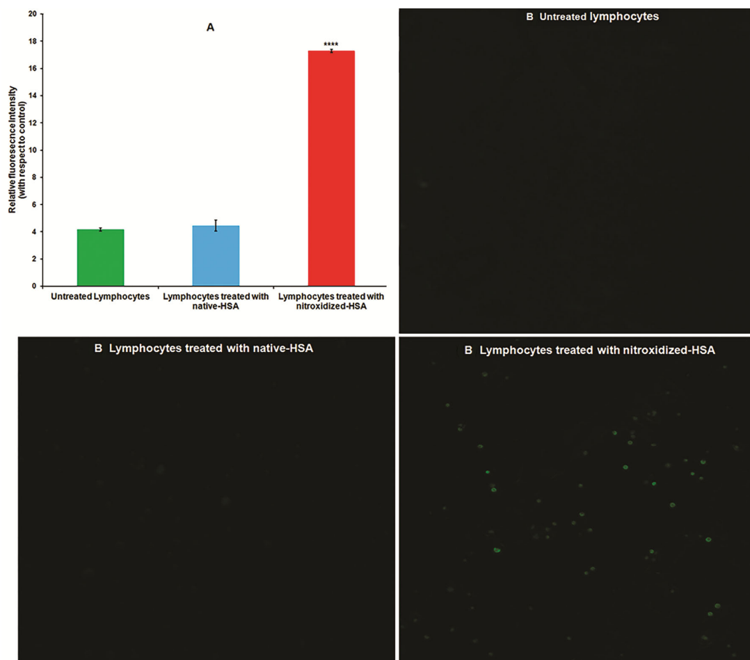
Fig. 3 — Detection of intracellular ROS generation in lymphocytes treated with HSA/nitroxidized-HSA. (A) Relative fluorescence intensities of lymphocytes treated with native/nitroxidized-HSA. All data has been expressed as mean \pm SD. Data were analysed by ANOVA followed by Tukey's multiple comparison test. Significantly different compared to untreated and native-HSA treated lymphocytes at **** P \leq 0.0001 ; and (B) Microscopic visualisation of intracellular ROS in untreated lymphocytes; and lymphocytes treated with native/nitroxidized-HSA
