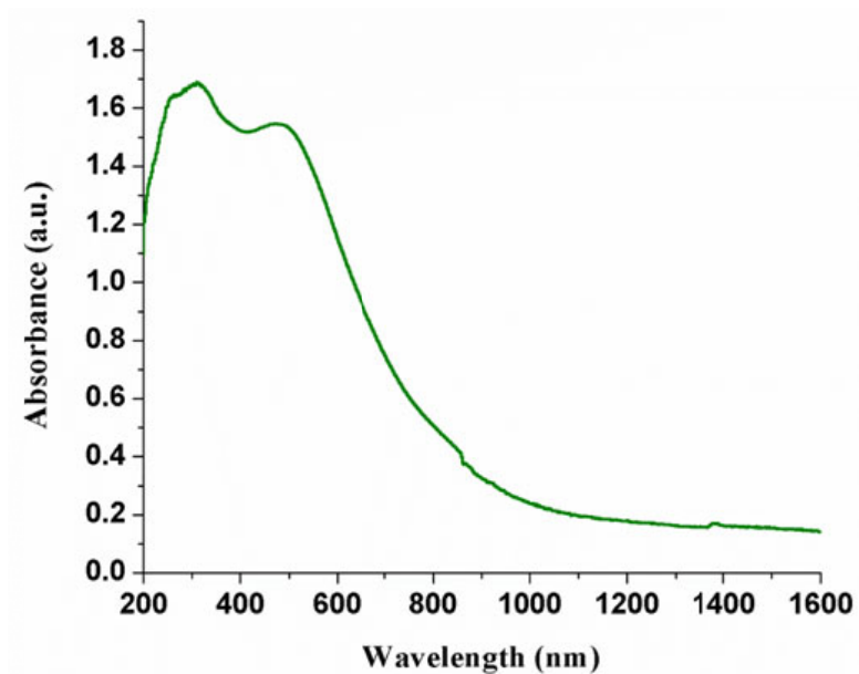
Suppl. Fig. S7 — Electronic Spectrum of Complex D1
