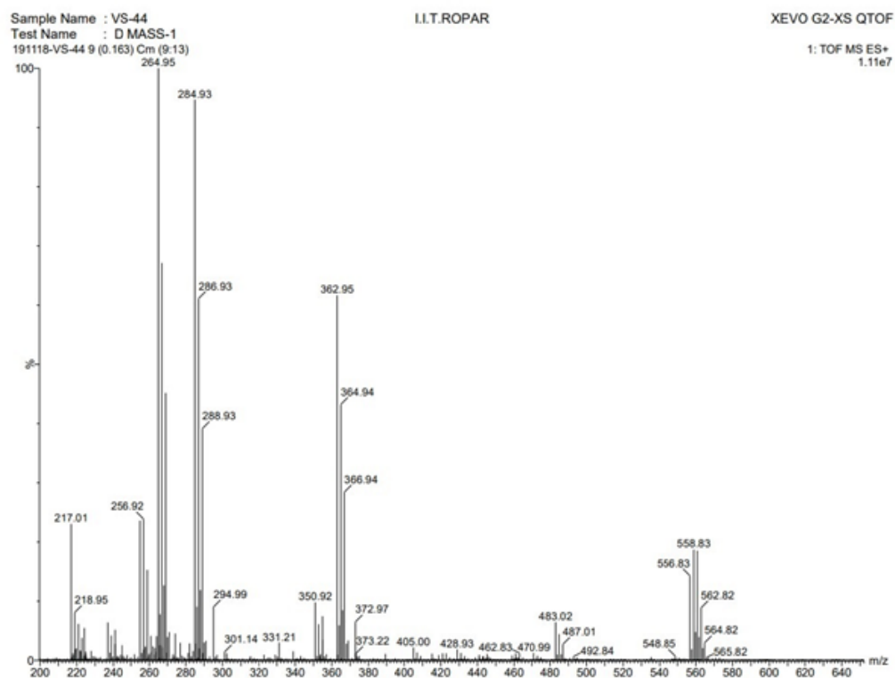
Suppl. Fig. S5 — ESI-MS data of complex D7
