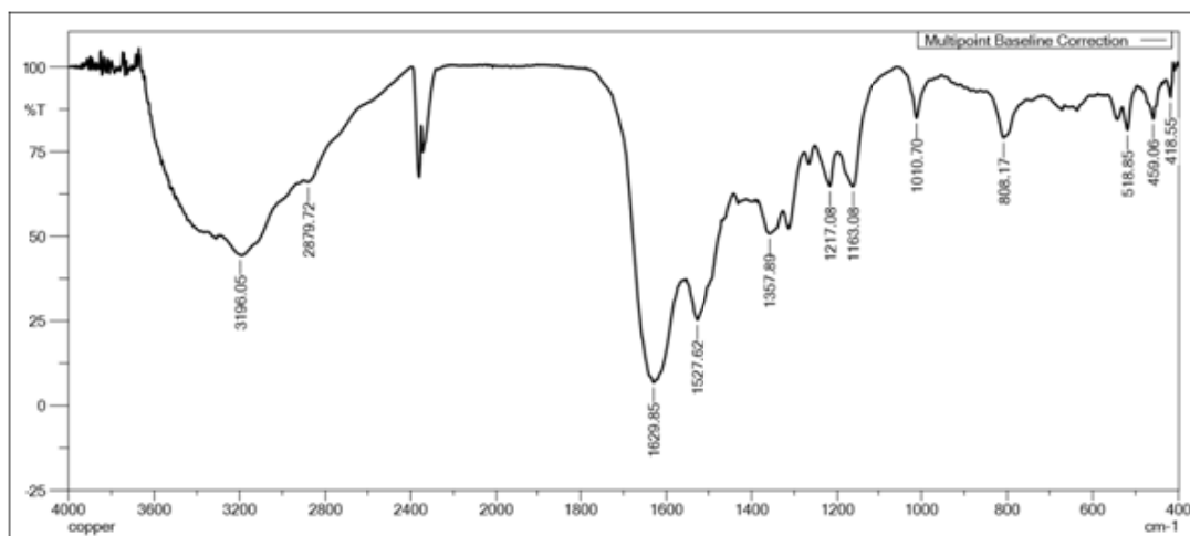
Suppl. Fig. S3 — IR Spectrum of Complex D7
