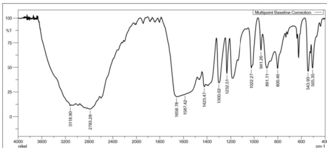
Suppl. Fig. S2 — IR Spectrum of Complex D4
