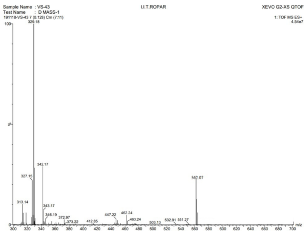
Suppl. Fig. S6 — ESI-MS data of complex D10
