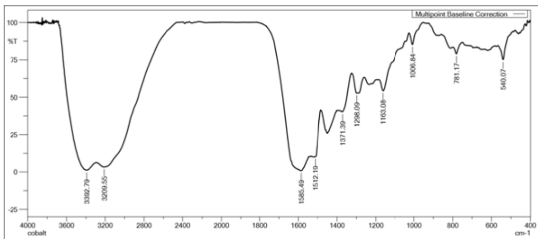
Suppl. Fig. S1 — IR Spectrum of Complex D1
