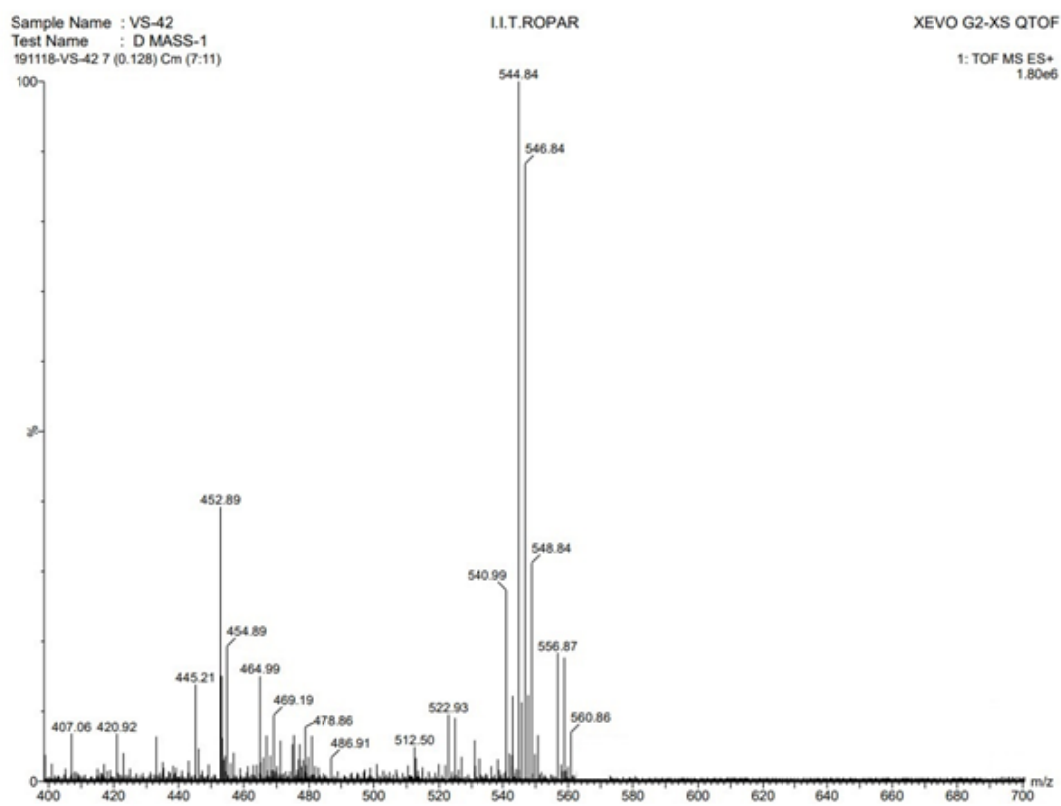
Suppl. Fig. S4 — ESI-MS data of complex D4
