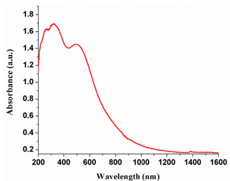
Suppl. Fig. S8 — Electronic Spectrum of Complex D4
