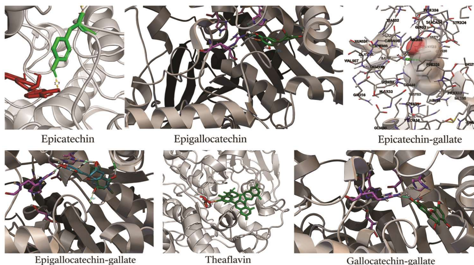
Suppl. Fig. S3 — Molecular docking of several tea-flavonoids on AChE
