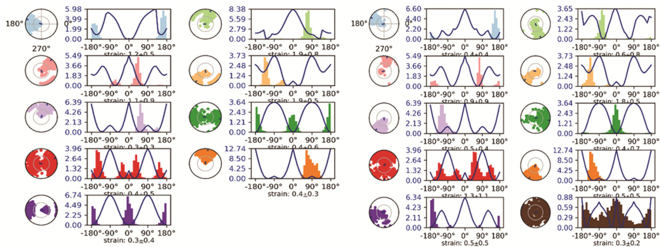
Fig. 9 — Ligand torsion angle profiles of 1B2Y & 5KZW
