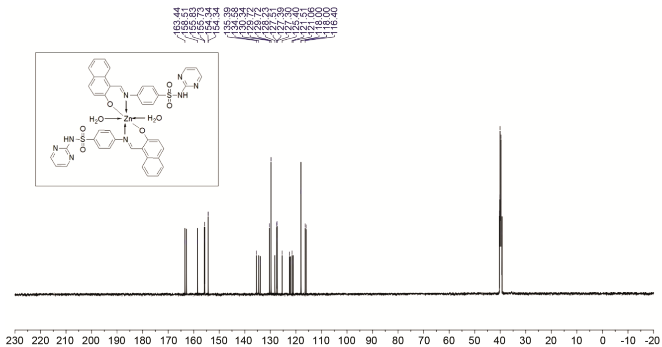
Suppl. Fig. S7 — ^{13}\text{C} NMR spectrum of Zn Complex 5
