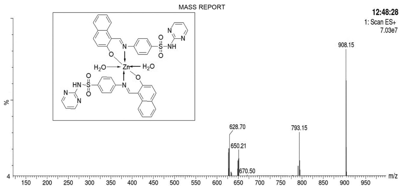
Suppl. Fig. S5 — Mass spectrum of Zn Complex 4
