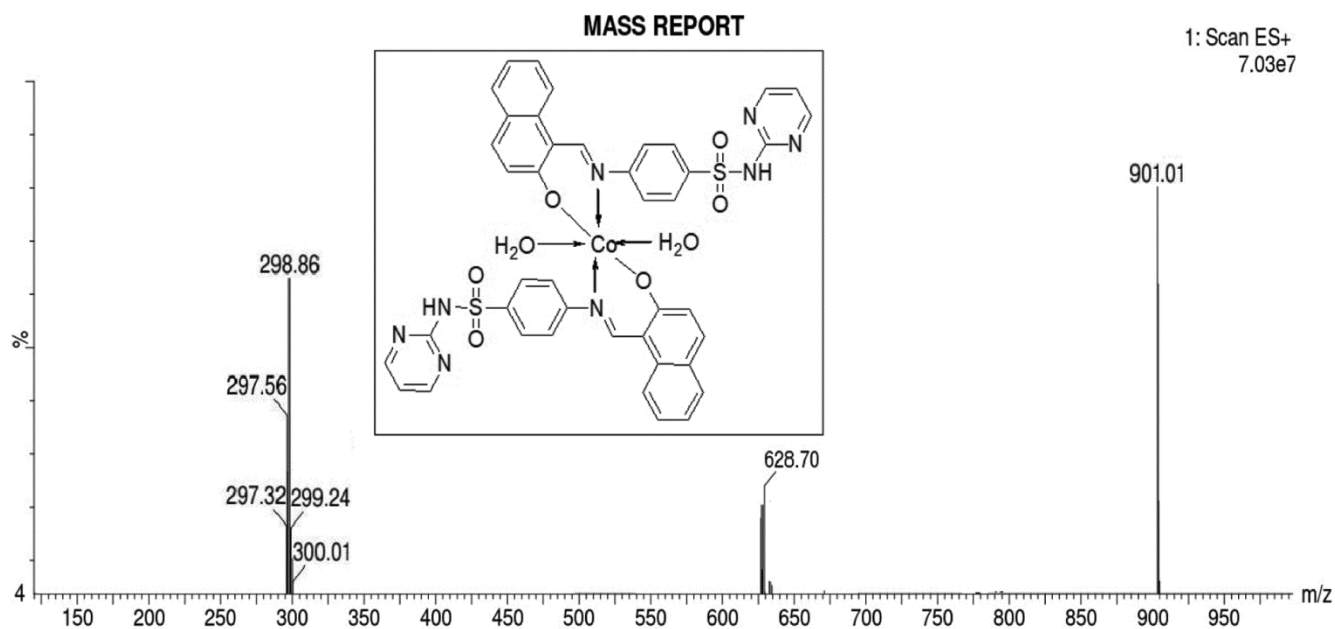
Suppl. Fig. S9 — Mass spectrum of Co Complex 6
