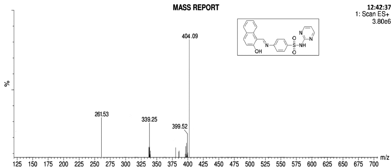
Suppl. Fig. S1 — Mass spectrum of Ligand 2
