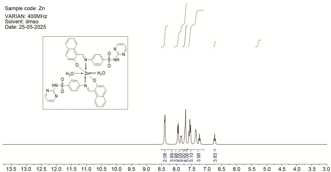
Suppl. Fig. S6 — ^1\text{H} NMR spectrum of Zn Complex 4
