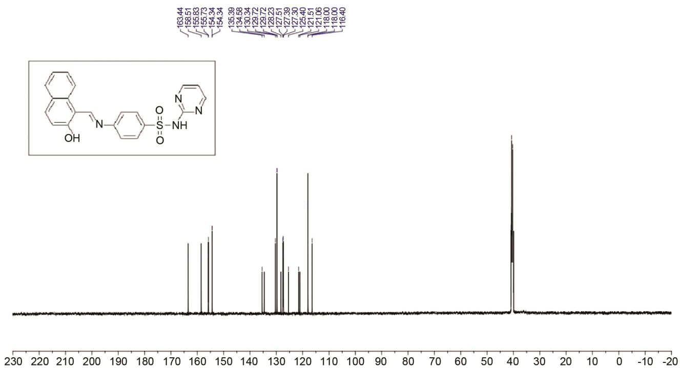
Suppl. Fig. S3 — 13 C NMR spectrum of Ligand 3
