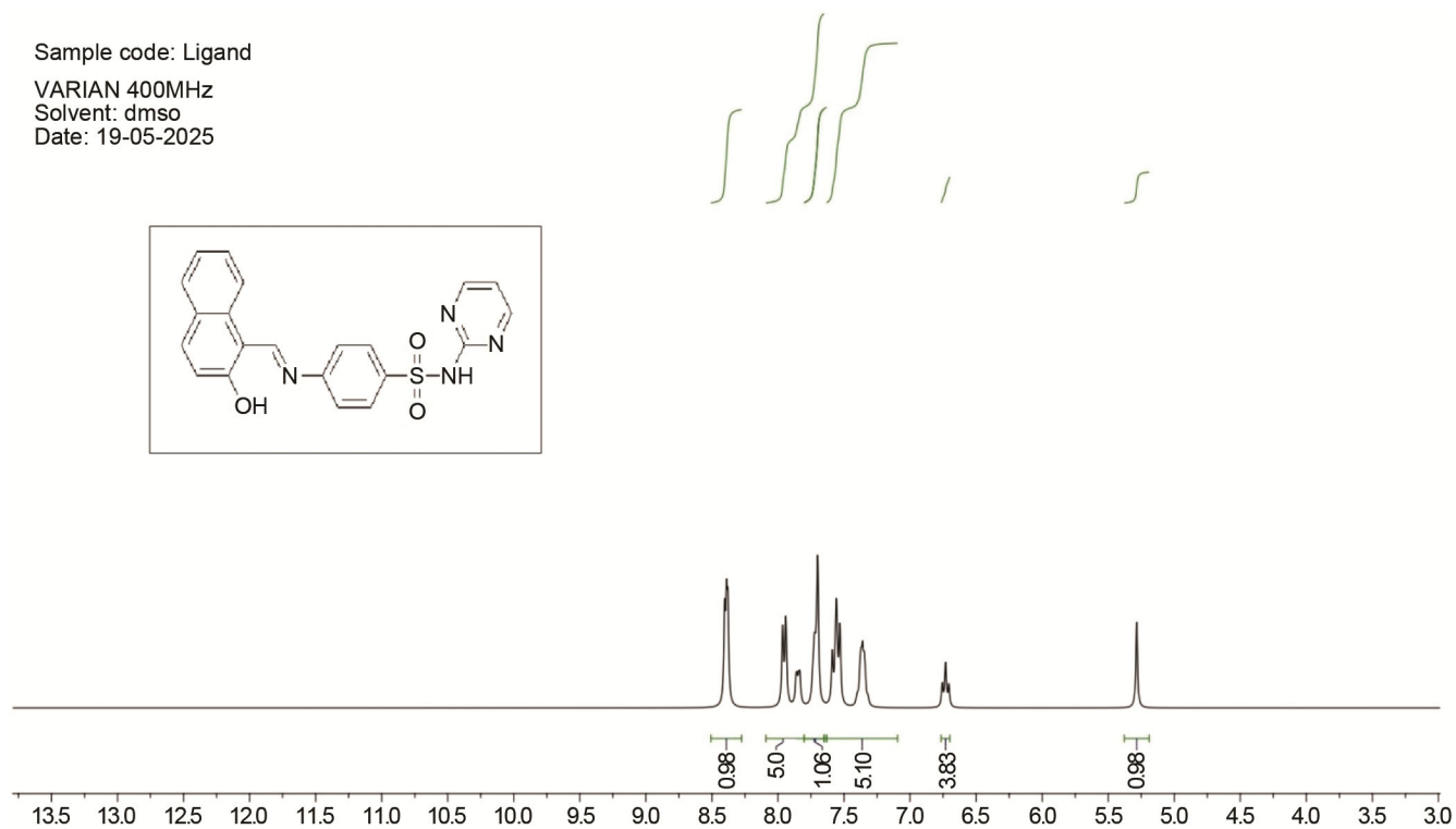
Suppl. Fig. S2 — 1 H NMR spectrum of Ligand 2
