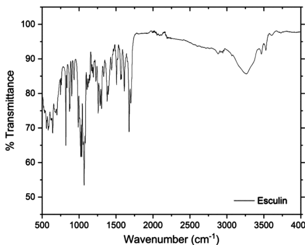
Suppl. Fig. 2 — FTIR Spectrum of Esculin
