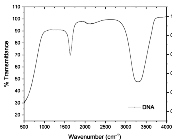
Suppl. Fig. 1 — FTIR Spectrum of DNA
